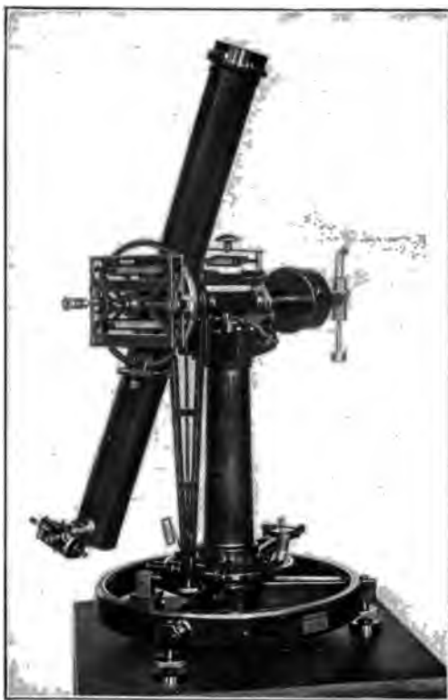
FIG. 12.—ZENITH TELESCOPE.
