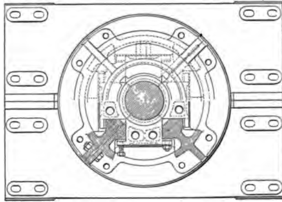
THRUST BEARING AS DESIGNED BY FAESCH & PICCARD
