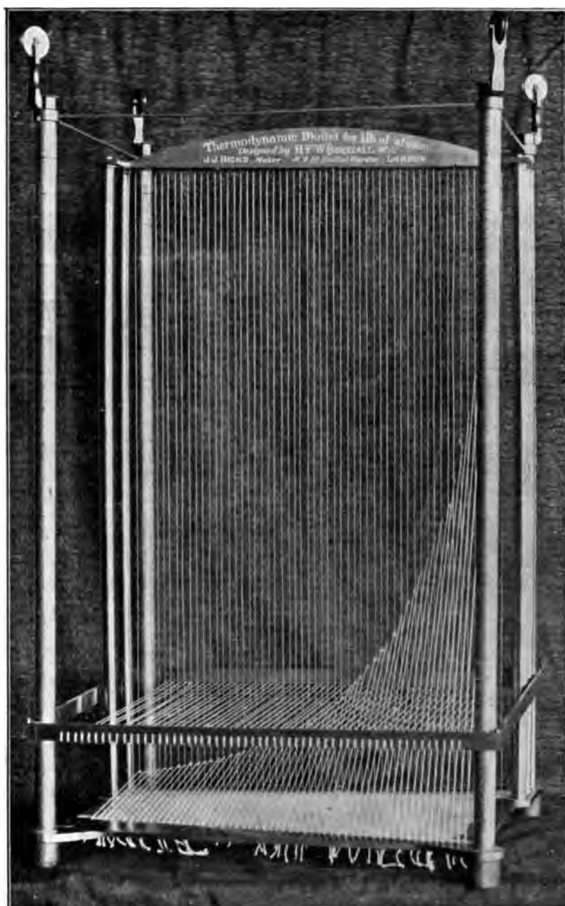
FIG. 131.—THERMODYNAMIC MODEL.
