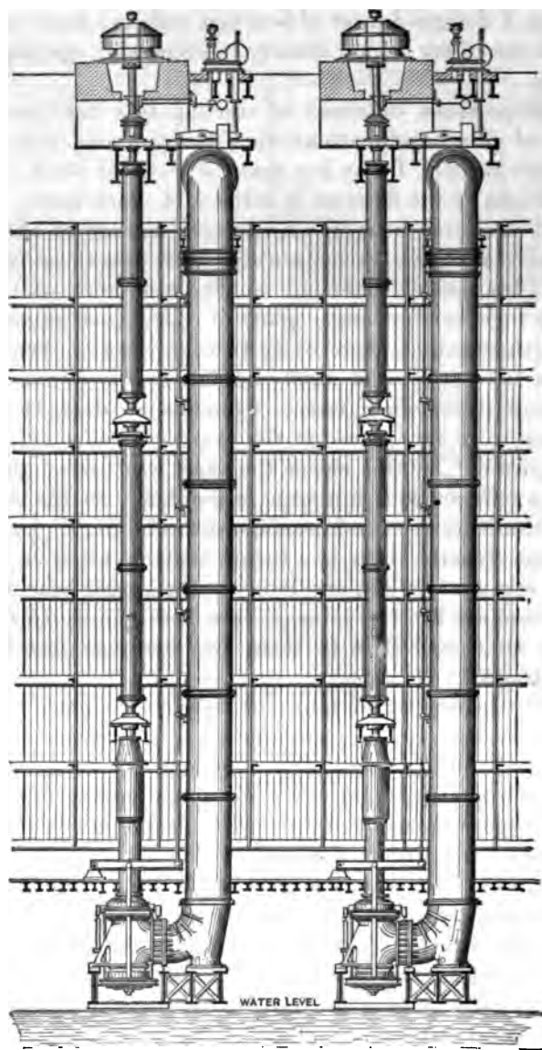
FIG. 211.—GENERAL ELEVATION. FAESCH & PICCARD DESIGN.
