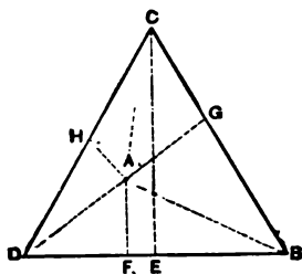
FIG. 126.—TERNARY ALLOYS.
