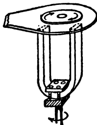
FIG. 2.—Another Form of Arago's Experiment.
