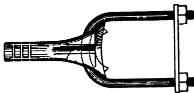
Fig. 101.—Solid metal clamp pin.
