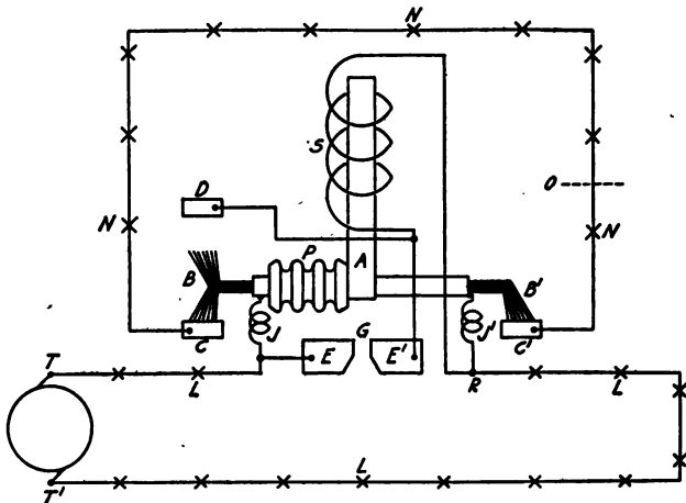
FIG. 251.—Automatic arc loop cutout switch.
