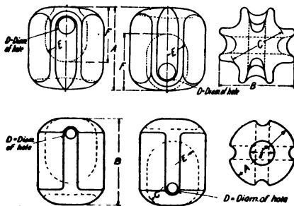
FIG. 129.—Porcelain strain insulators.
