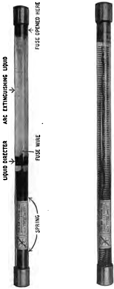
FIG. 259.—Chemical fuse. Upper cut illustrates a blown fuse. Lower cut a fuse ready for operation.
