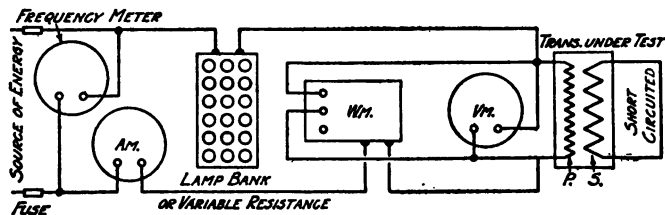
Fig. 187.—Copper loss or impedance test.
