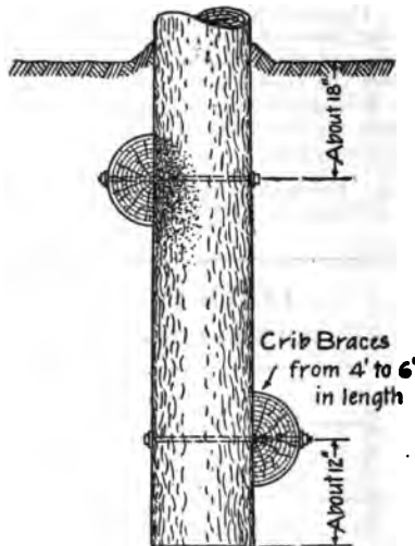
FIG. 368.—Crib bracing.
