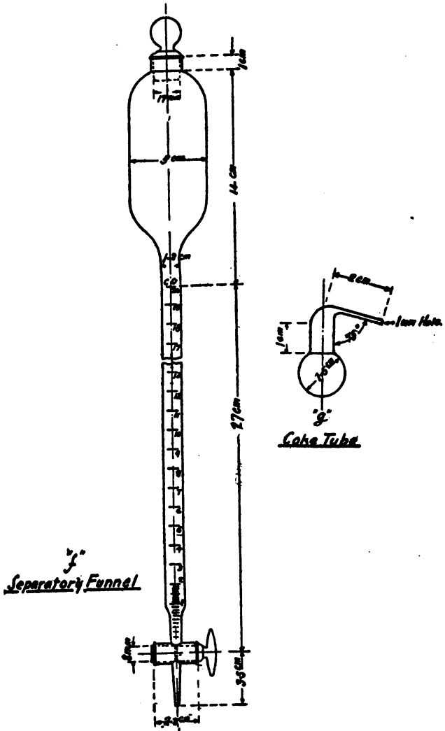
FIG. 359.—National Electric Light Association creosote oil analysis.
