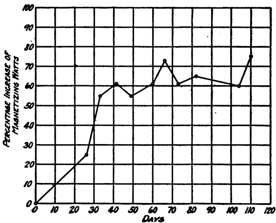
Fig. 163.—Increase in hysteresis loss of iron due to continued heating.
