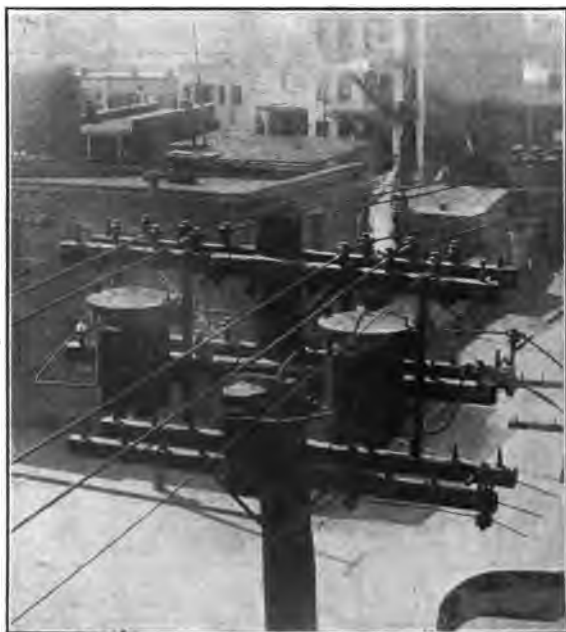
FIG. 407.—Installation of three transformers.
