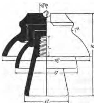
FIG. 118.—Glass pin type insulator, line voltage 25,000 volts.
