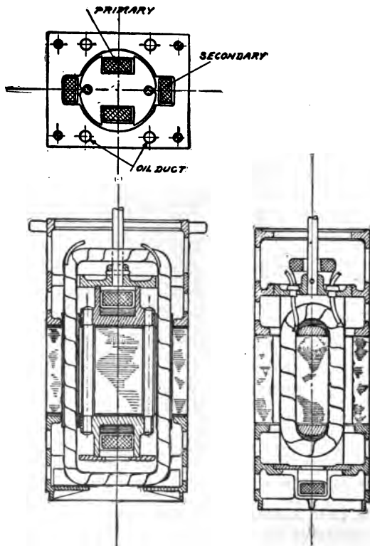
FIG. 219.—Section of regulator winding and core.
