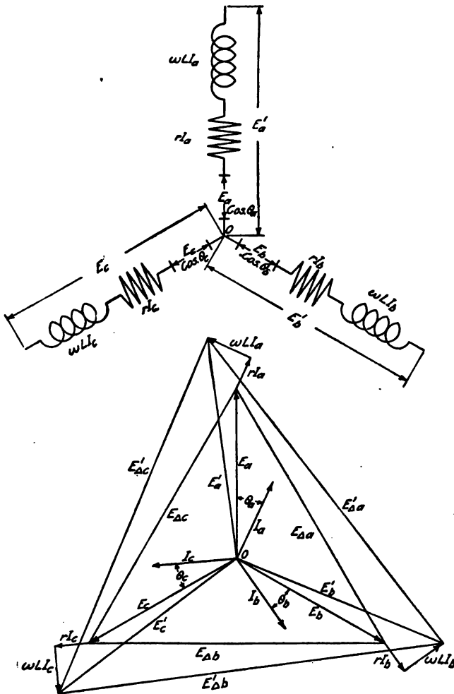
Fig. 294.—Three-phase system.
