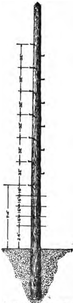
FIG. 369.—Location of steps on pole.
