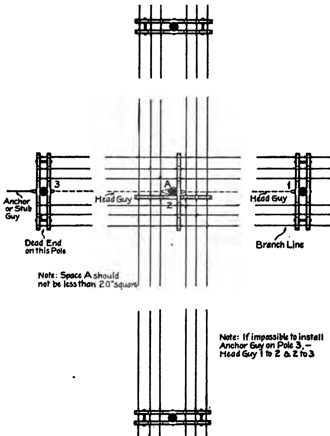
FIG. 374.—Junction pole without double arms.
