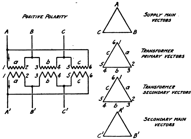
Fig. 197.—Transformers connected "Δ" primary and "Δ" secondary.
