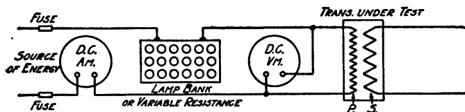
Fig. 186.—Measurement of resistance by the fall of potential method.
