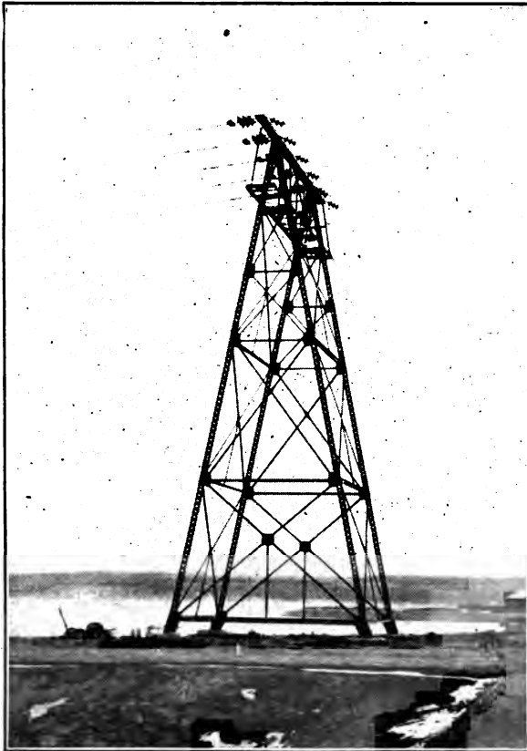
FIG. 65.—Double circuit river crossing, three-phase, 66,000 volts, 2,000 feet span
