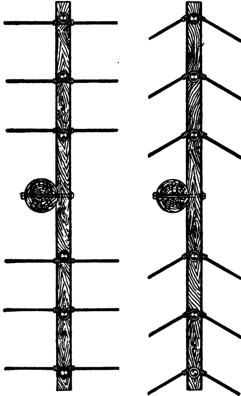
Fig. 389.—Location of wires on insulators.
