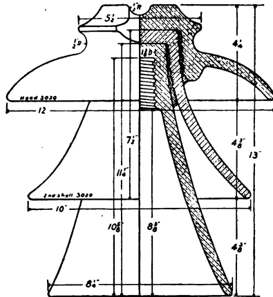
FIG. 115.—Porcelain pin type insulator, line voltage 44,000 volts.
