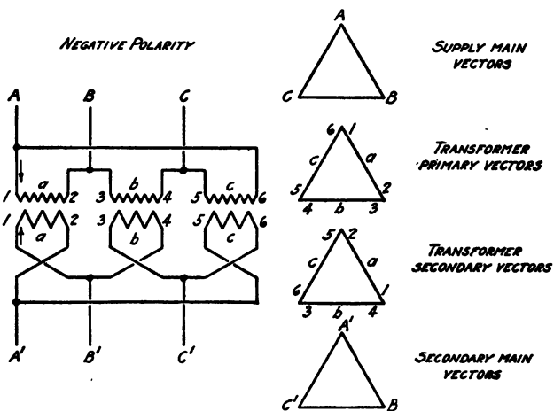
FIG. 202.—Transformers connected "Δ" primary and "Δ" secondary.
