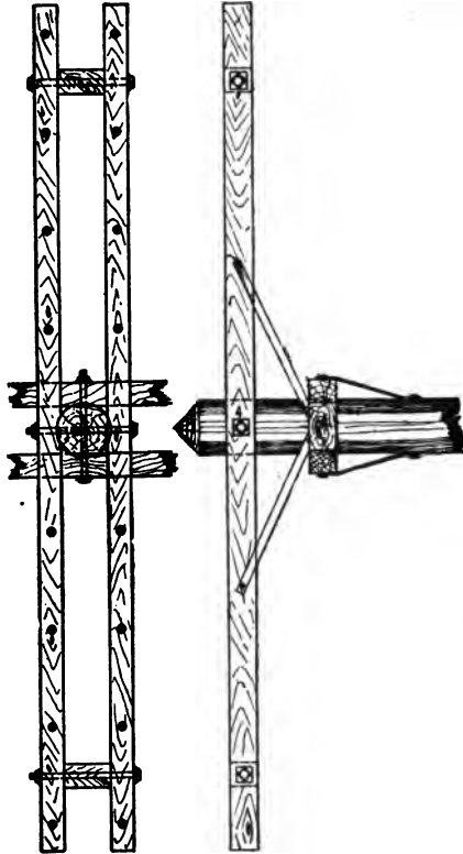
FIG. 372.—Double cross-arms.
