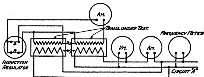
FIG. 181.—Heat test of single-phase transformer using induction regulator and testing transformer. (Losses only supplied.)
