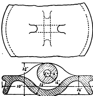
FIG. 124.—Porcelain suspension type insulator.
