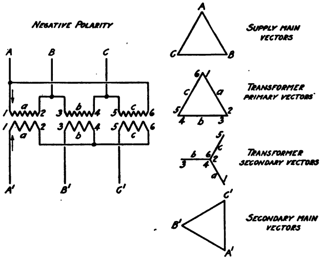
FIG. 205.—Transformers connected "Δ" primary and "Y" secondary.
