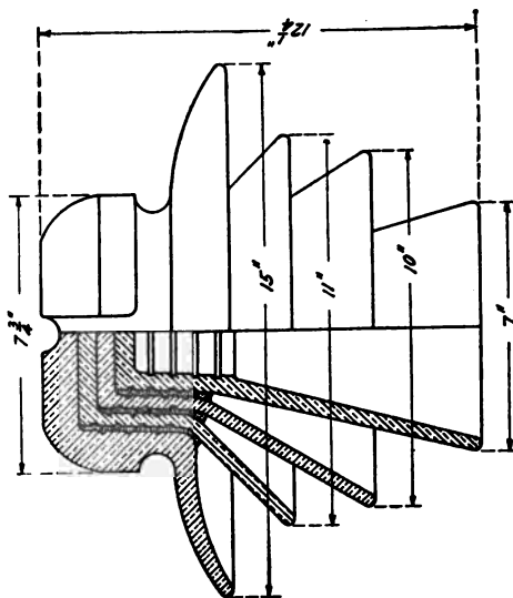
Fig. 113.—Porcelain pin type insulator, line voltage, 50,000 volts.
