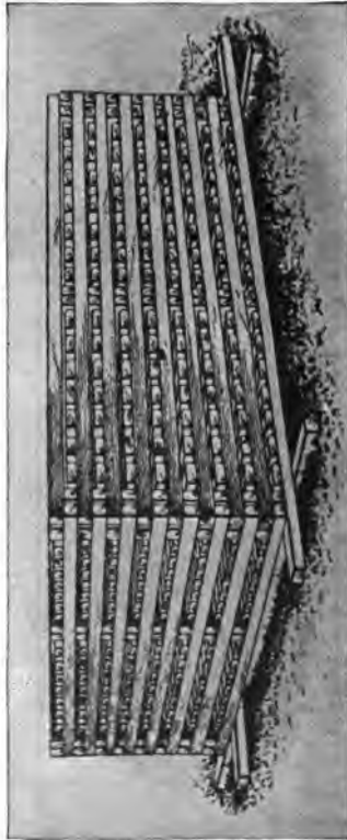
Fig. 332.—Ideal form of piling cross-arms, 20 x 20, giving free circulation of air.
