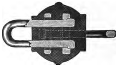
FIG. 132.—Composition strain insulator.
