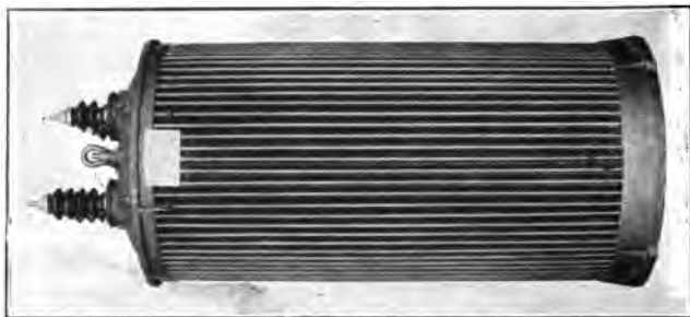
Fig. 157. —Self cooling out-door type transformer, single-phase, 500 kv-a, 33,000/5,600 volts, 60 cycles.
