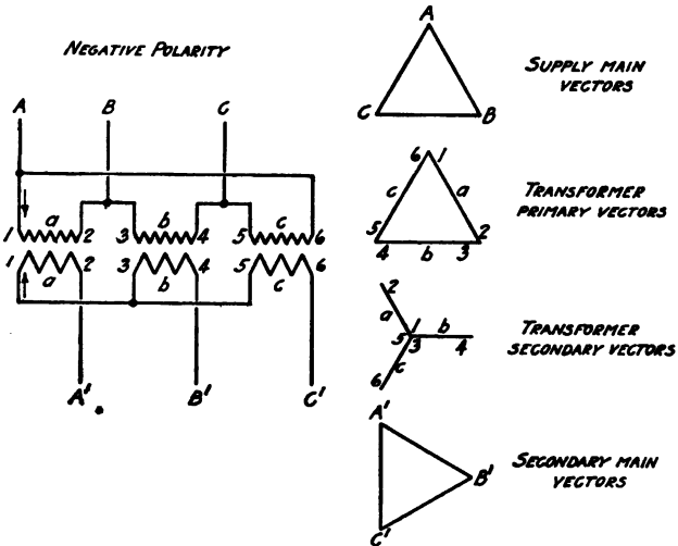
FIG. 206.—Transformers connected "Δ" primary and "Y" secondary.
