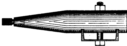
Fig. 100.—Swedged pipe pin, separable thimble.
