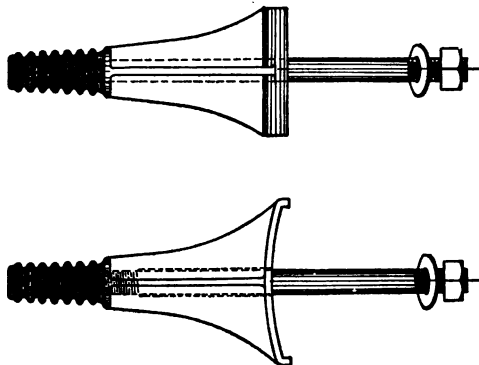
Fig. 99.—Solid metal pin, with separable thimble.
