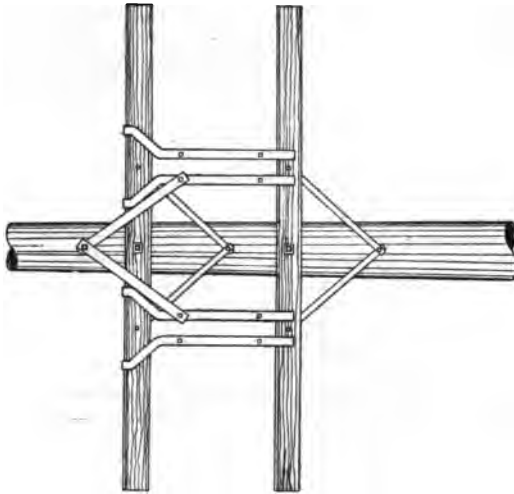
Fig. 400.—Special iron braces for two transformers.
