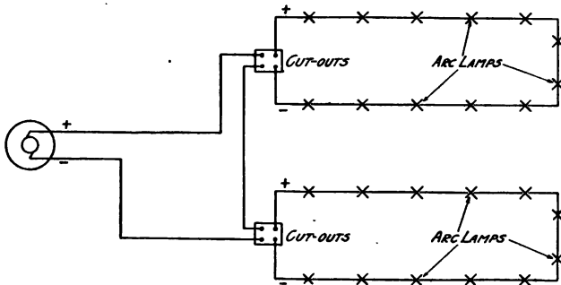
Fig. 275.—Direct current series arc lighting system.
