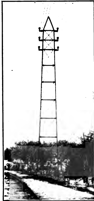
FIG. 53.—Double circuit three-phase steel "A" frame 35,000 volts.
