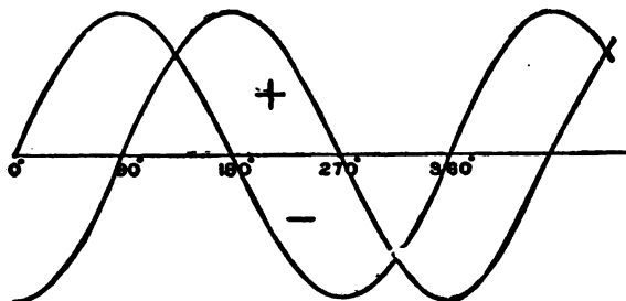
FIG. 18.—Relation of the Waves of Current, or e.m.f.'s. in a Two-phase System.
