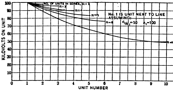
FIG. 140.—Calculated voltage across different insulators in a string of "n" units.
