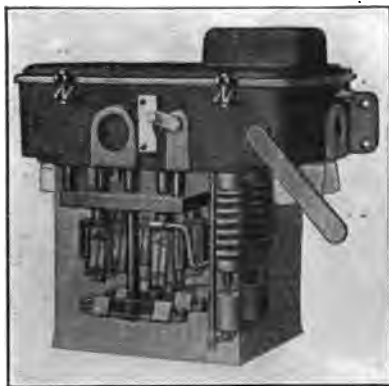
FIG. 253.—Automatic oil switch 3 P. S. T., 100 amperes, 2,200 volts.
