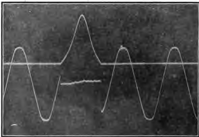
FIG. 260.—Oscillogram illustrating the action of the fuse in FIG. 259 when opening a short circuit.
