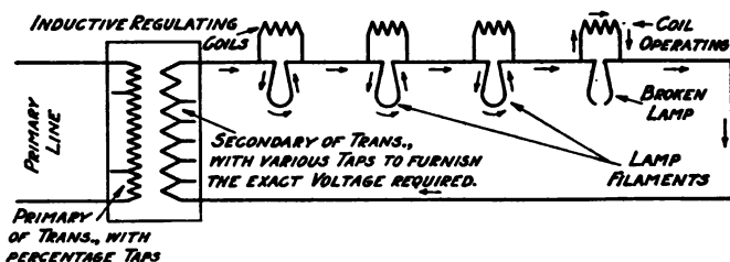
FIG. 212.—Special series incandescent lighting transformer.
