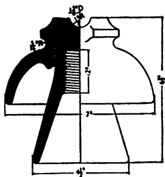
FIG. 119.—Glass pin type insulator, line voltage 20,000 volts.
