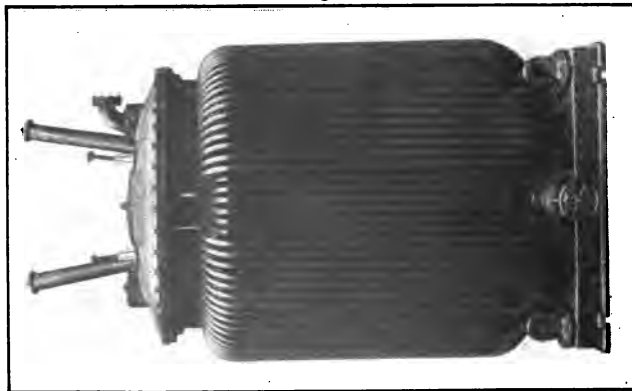
Fig. 155. —Self cooling out-door type transformer, single-phase, 2,000 kv-a, 101,200/13,200 volts, 60 cycles.
