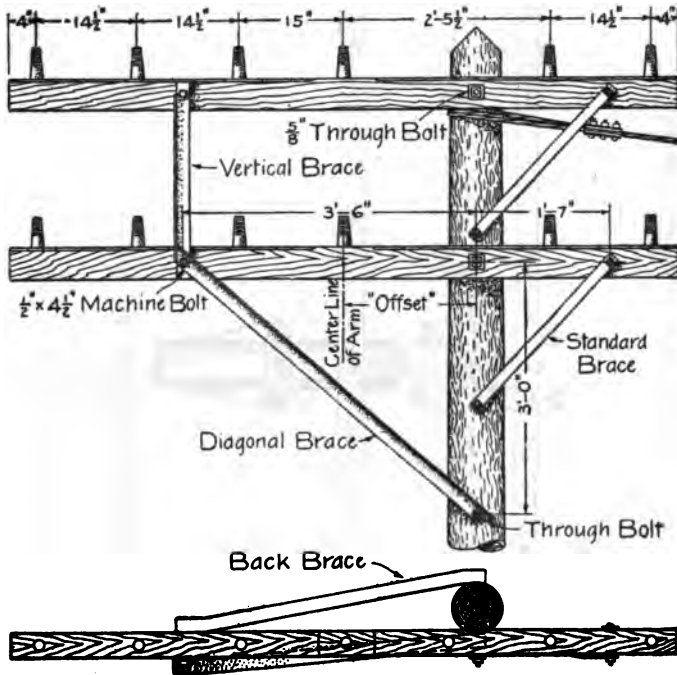
FIG. 371.—Side cross-arm bracing.
