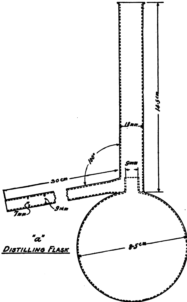
FIG. 356.—National Electric Light Association creosote oil analysis.
