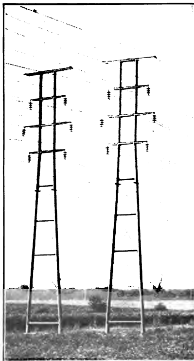
FIG. 54.—Double circuit three-phase steel "A" frames.
