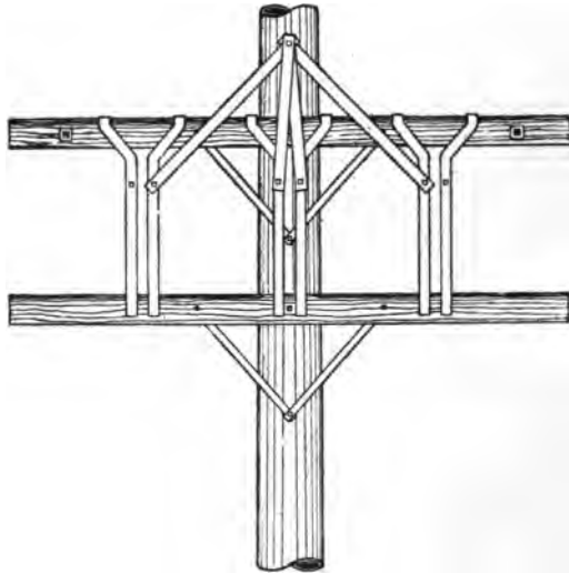
Fig. 401.—Special iron braces for three transformers.
