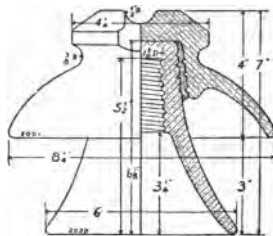
FIG. 117.—Porcelain pin type insulator, line voltage 22,000 volts.
