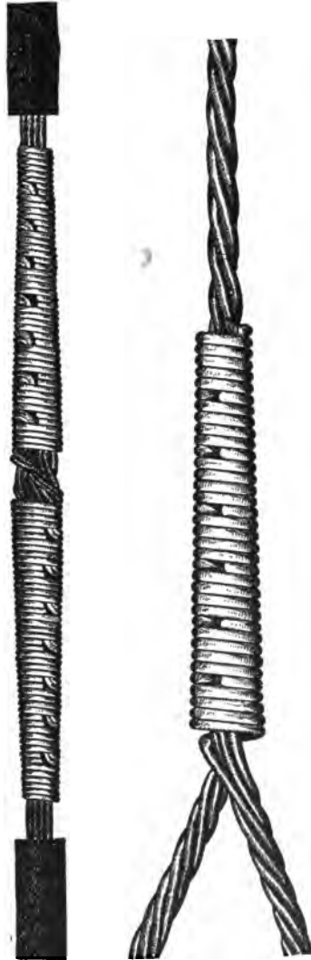
FIG. 393.—Stranded cable splice and tap.
