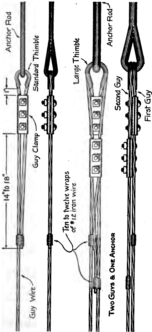
FIG. 383.—Methods of attachment of guys to anchor rods.
