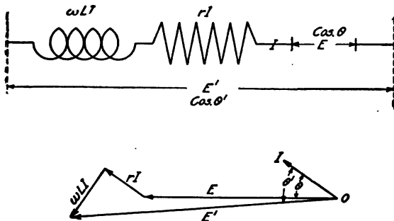
Fig. 291.—Single phase system
