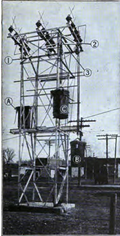
FIG. 76.—Steel outdoor sub-station for 33,000 volts. 1, 2 and 3 are jib cranes for handling transformers A, B, and C, respectively.
