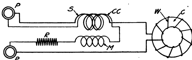
FIG. 184.—Internal connections of iron loss voltmeter.
