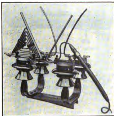
FIG. 257.—Horn gap link fuse.
