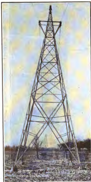
FIG. 56.—Single circuit three-phase steel tower 50 feet high for 66,000 volts.
