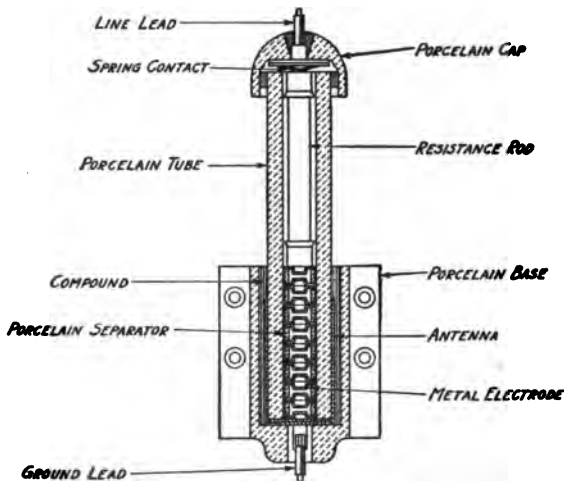
FIG. 227.—Compression type arrester.
