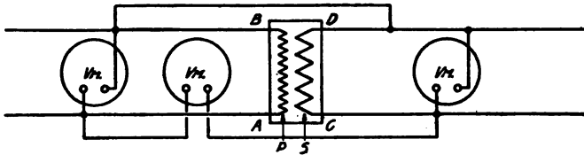
FIG. 191.—Connections for polarity test.
