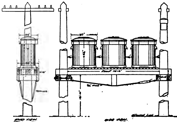
FIG. 403.—Special transformer rack.
