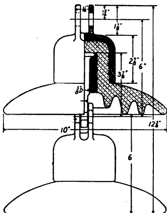
FIG. 122.—Porcelain suspension type insulators.
