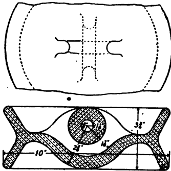
FIG. 128.—Porcelain strain insulators.
