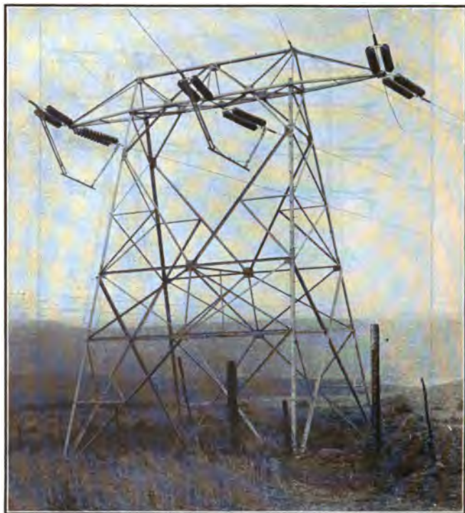
FIG. 61.—Single circuit steel anchor tower at corner, 150,000 volts.
