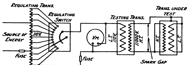
Fig. 174.—Insulation test. (Using special testing transformer.)
