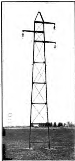
FIG. 52.—Single circuit three-phase steel "A" frame 60,000 volts.
