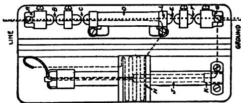
FIG. 228.—Diagrammatic view of circuit breaker lightning arrester.
