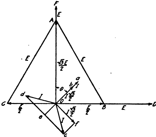
FIG. 211.—Vector analysis of three-phase, two-phase transformation.
