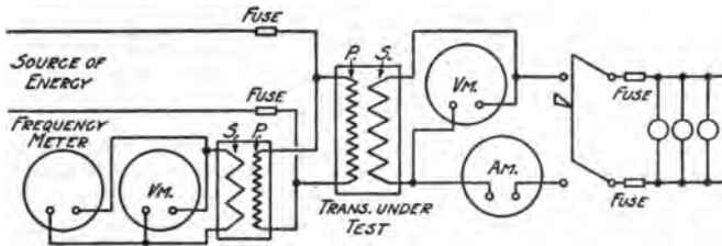
Fig. 188.—Connections for regulation test.
