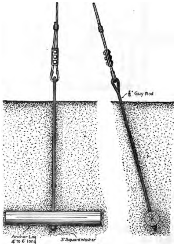
FIG. 382.—Anchor guy.
