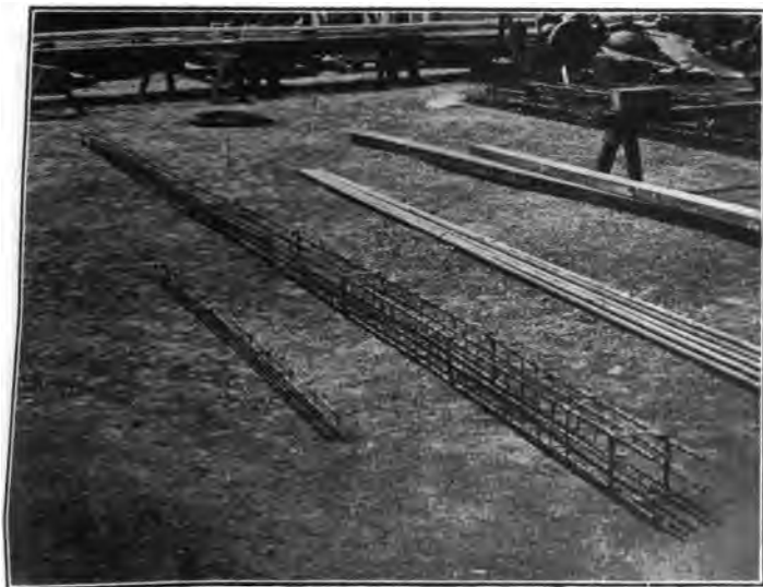
FIG. 36.—Steel reinforcement for solid concrete pole and cross-arm.
