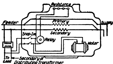
FIG. 220.—Connection diagram of pole type regulator.
