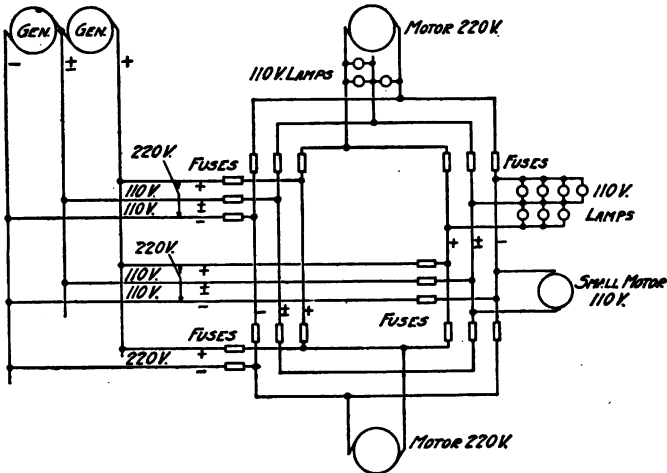
Fig. 274.—Edison three-wire system.
