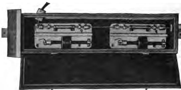
FIG. 230.—Circuit breaker lightning arrester, single pole, 6,800 volts.
