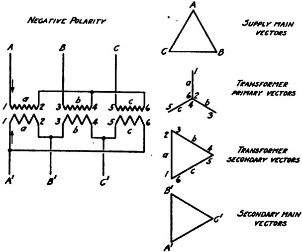
FIG. 203.—Transformers connected "Y" primary and "Δ" secondary.
