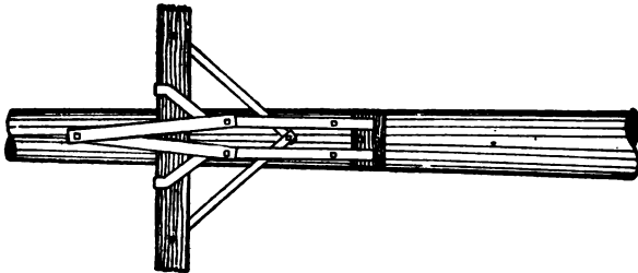
Fig. 399.—Special iron braces for individual transformer.
