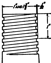
FIG. 91.—Standard pin threads.
