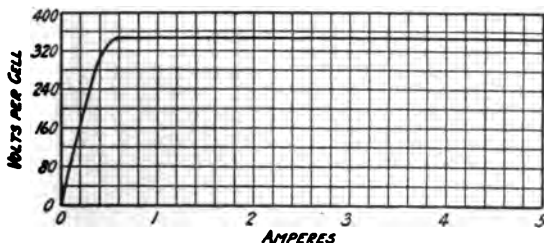
FIG. 231.—Characteristic curve of aluminum cell or electrolytic lightning arrester for alternating current.
