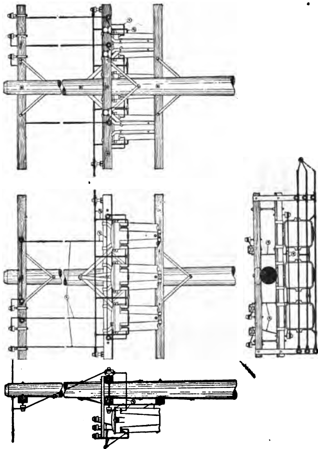
FIG. 402.—Wiring diagram of a three transformer installation.
