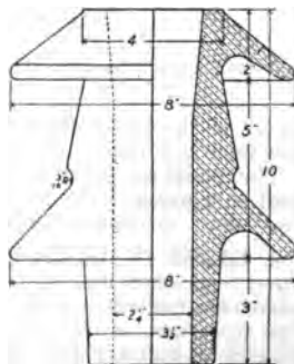
FIG. 125.—Porcelain through pin type insulator, line voltage 23,000 volts.
