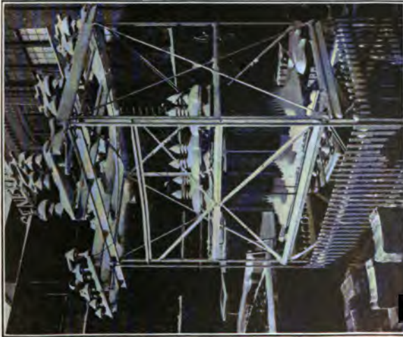
FIG. 72.—70,000 volt sub-station after a heavy snow storm.
