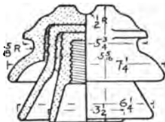
FIG. 116.—Porcelain pin type insulator, line voltage 25,000 volts.
