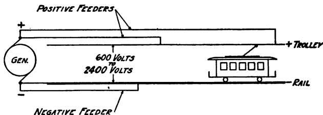
Fig. 273.—D. C. railway system.
