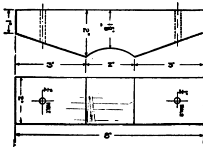
FIG. 385.—Standard tree block.
