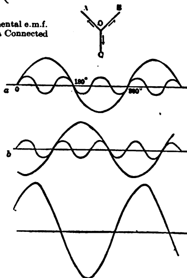
FIG 7.—Relation of the Fundamental e.m.f. and Triple Harmonics in a Star Connected Circuit.
