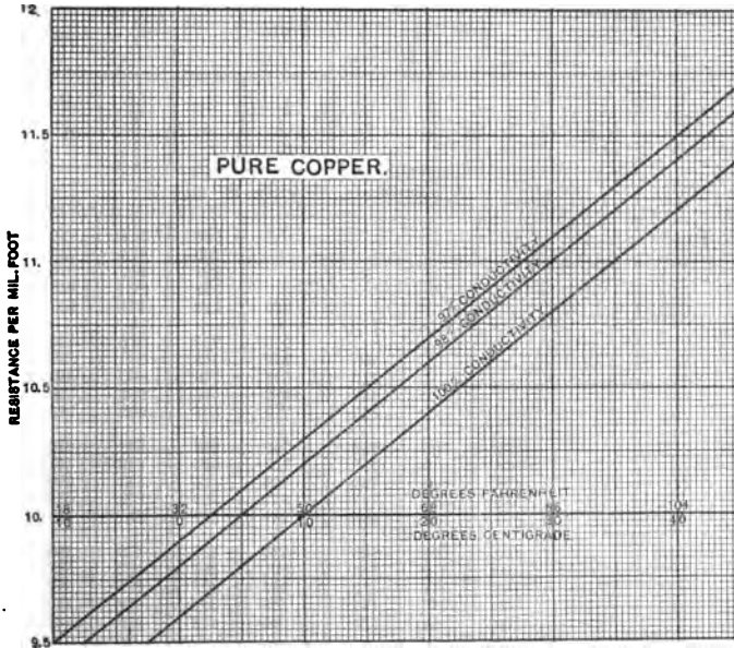
Fig. 77.—Resistance per Mil-Foot of Pure Copper at Various Temperatures and Conductivities. Values of K in expression C \sqrt{t \frac{d^2}{K}}
