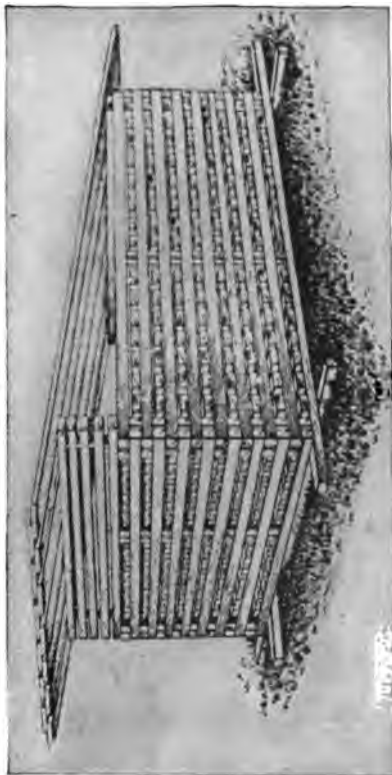
FIG. 333.—Recommended method of roofing, cross-arm piles with boards.
