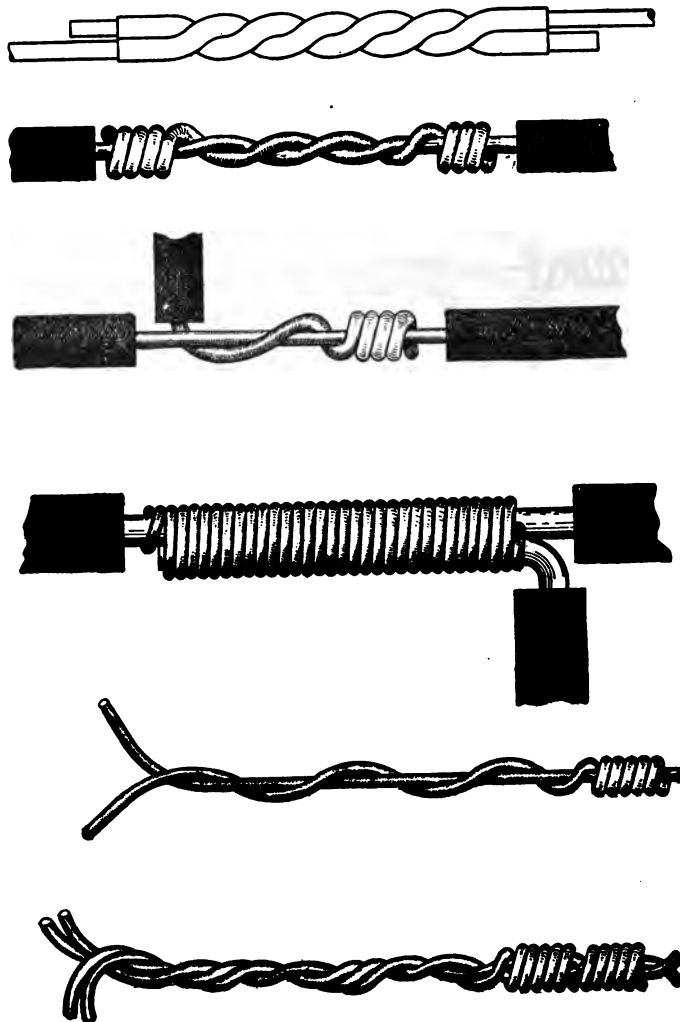
FIG. 392.—Solid wire splices and taps.
