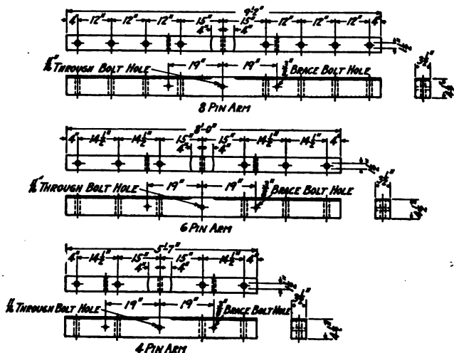
FIG. 88—Standard cross-arms
