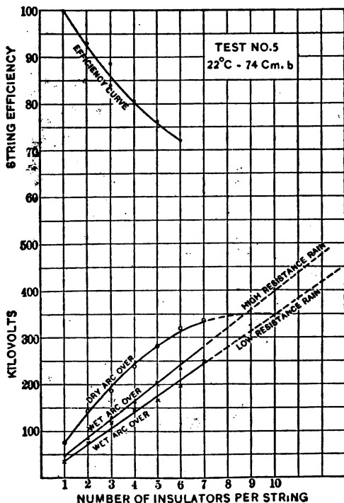
FIG. 142.—Test characteristic curves of suspension insulators.
