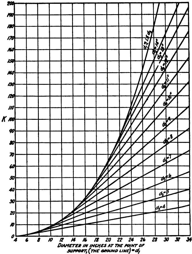
FIG. 322. Fibre stress in \frac{lb}{in^2} per lb-ft. of bending moment, -\frac{1}{2} .
