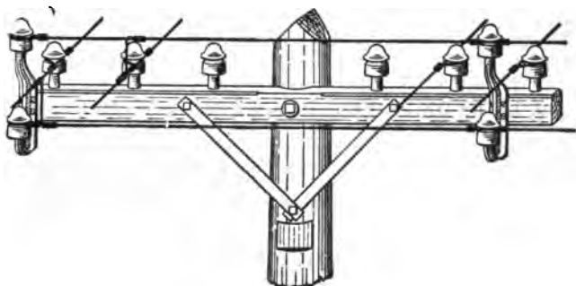
FIG. 304.—Branch tap line with spreader brackets.
