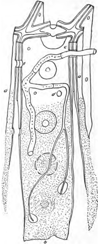
FIG. 342.—Tracheid of Pinus sylvestris , decomposed by Trametes Pini . The primary cell-wall has been completely dissolved as far as a. In the lower part the secondary and tertiary layers consist only of the cellulose, in which lime-granules are distinctly visible, b; filamentous mycelia, c, penetrate the walls and make holes as at d and e.
