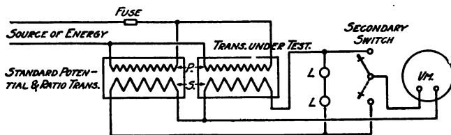
FIG. 189.—Connections for ratio test.
