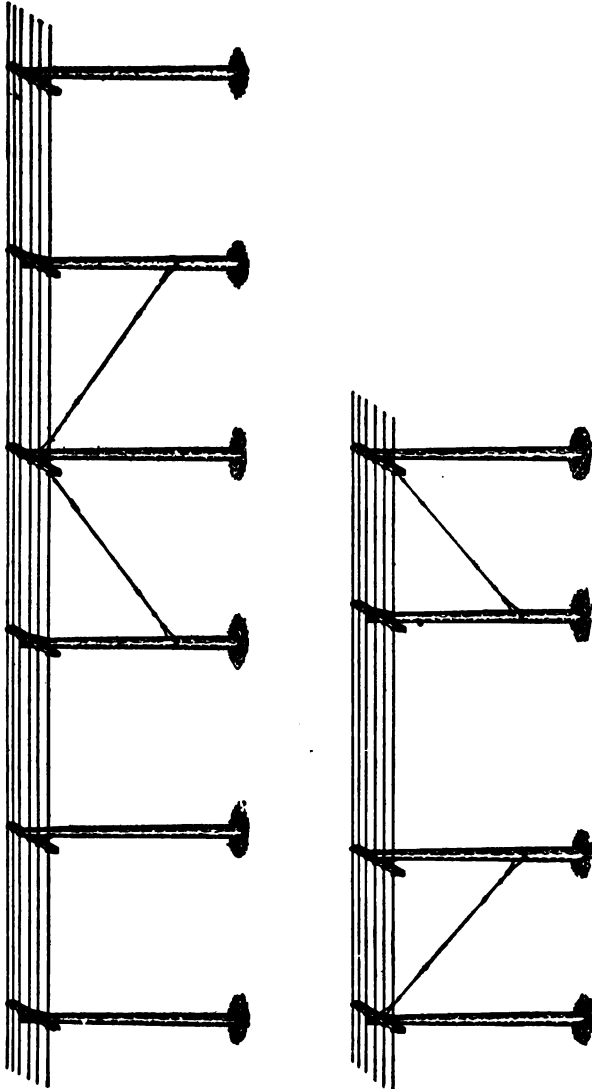
FIG. 375.—Head guys on straight lines and long spans.
