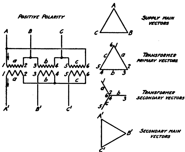
Fig. 199.—Transformers connected "Δ" primary and "Y" secondary.
