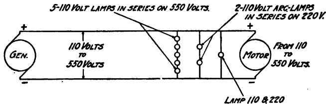
Fig. 272.—D. C. two-wire system.
