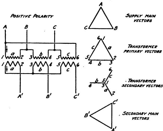
Fig. 200.—Transformers connected "Δ" primary and "Y" secondary.
