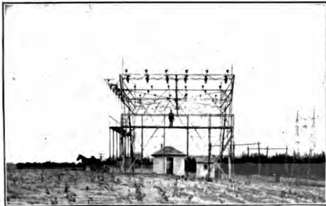
FIG. 69.—Outdoor sectionalizing and branch tower, three-phase, 66,000 volts.
