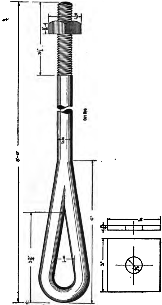
FIG. 110.—Standard guy rod and washer.
