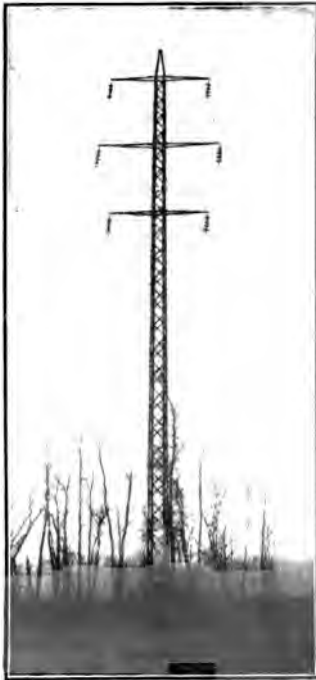
FIG. 47.—Double circuit three-phase steel pole.
