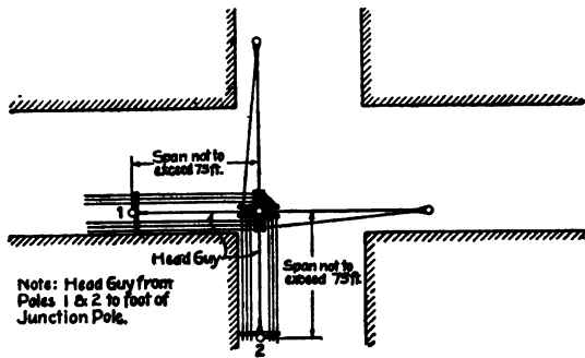
FIG. 387.—Cross-arm guying. One-pole method of turning corner.
