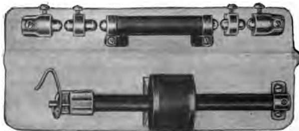
FIG. 229.—Circuit breaker lightning arrester, single pole, 3,300 volts.
