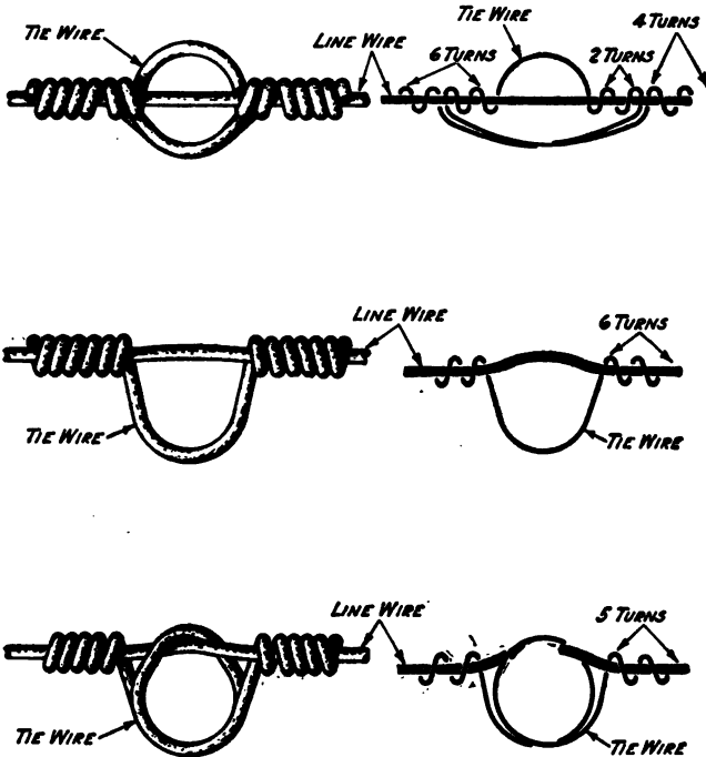
FIG. 391.—Ties.
