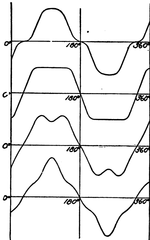
FIG. 13.—Various Distortions of the Fundamental Wave by Triple and Quintuple Harmonics of Characteristics given Below :
