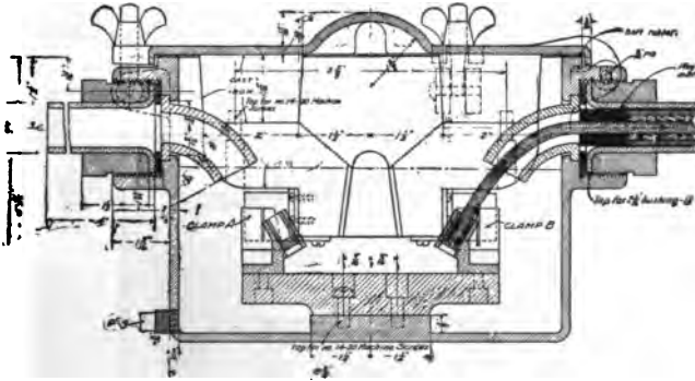
FIG. 261.—Oil fuse box showing details of construction.
