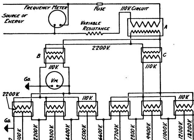
Fig. 175.—Insulation test (using standard transformers.)
