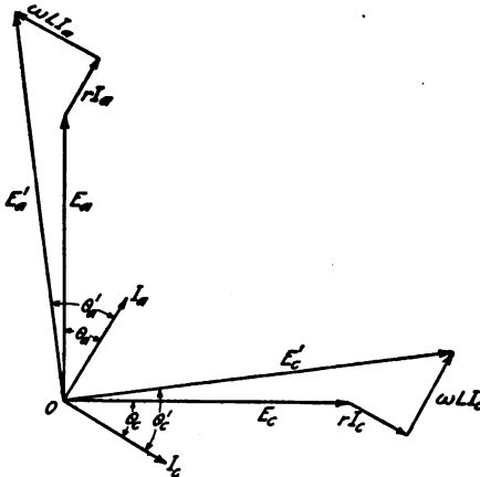
Fig. 292.—Two phase, four wire system.
