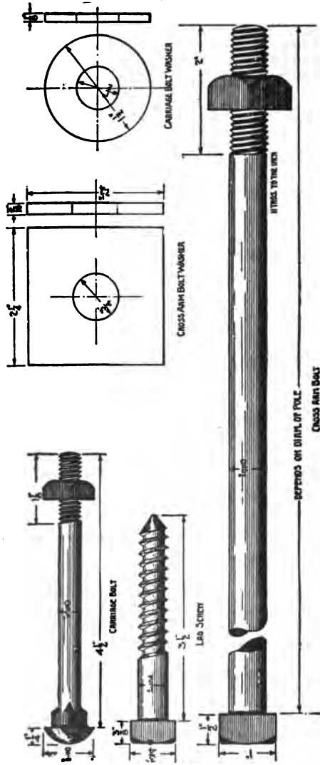
FIG. 108.—Standard cross-arm bolt, lag bolt, carriage bolt and washers.
