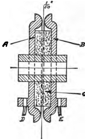
FIG. 236.—Diagrammatic view of single gap lightning arrester.
