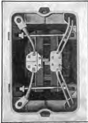
FIG. 147.—Method of insulating leads from case, 6600/110-220 volt transformer.
