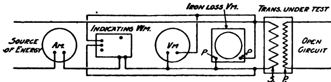
FIG. 183.—Iron loss test.
