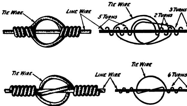
FIG. 390.—Ties.
