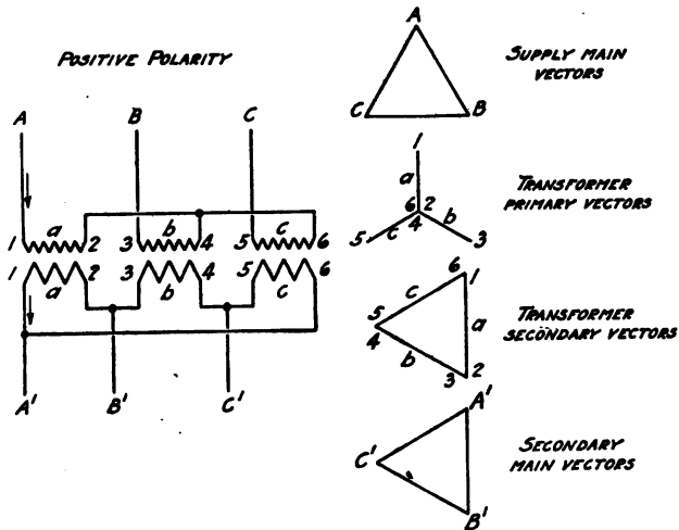
Fig. 198.—Transformers connected "Y" primary and "Δ" secondary.
