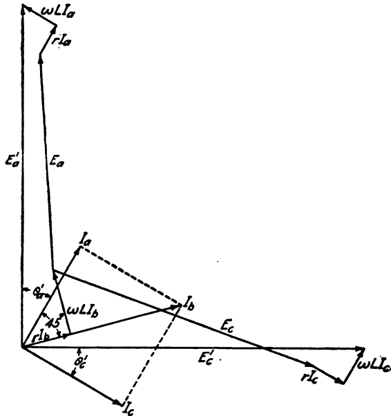
Fig. 293.—Two-phase, three-wire system.
