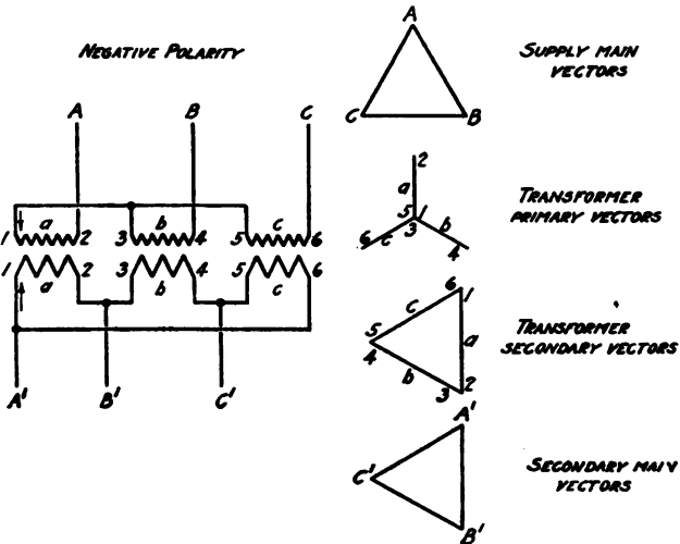
FIG. 204.—Transformers connected "Y" primary and "Δ" secondary.
