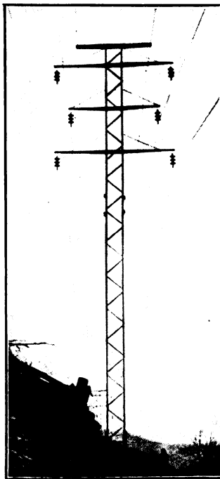
FIG. 50.—Double circuit narrow base flexible steel frame three-phase 44,000 volts.
