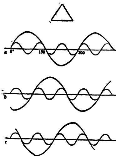
FIG. 6.—Relations of the Fundamental e.m.f. and Triple Harmonics in a Delta Connected Circuit.
