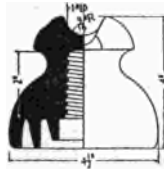
FIG. 120.—Glass pin type insulator, line voltage 10,000 volts.
