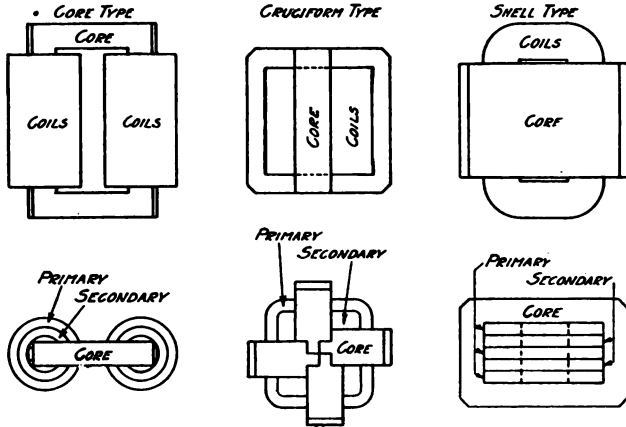
FIG. 149.—Types of transformer cores.
