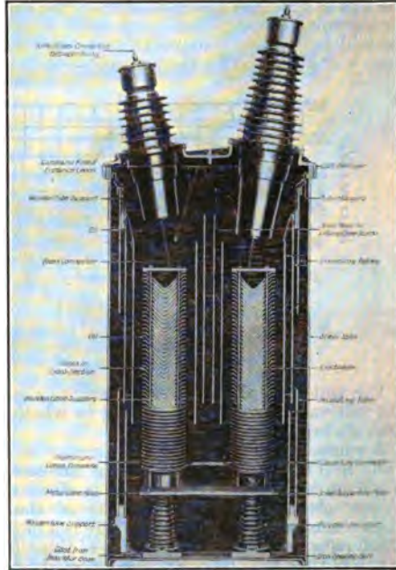
FIG. 233.—Single pole aluminum cell lightning arrester for 110,000 volt circuits.
