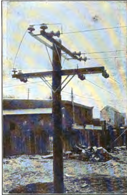
FIG. 423. —Turning a 90° bend on one pole.
