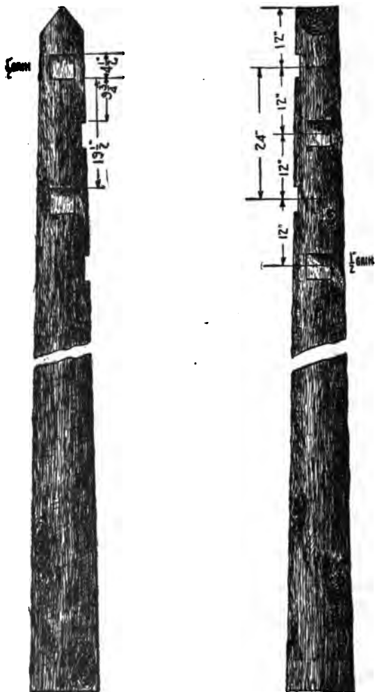
FIG. 366.—Pole framing.
