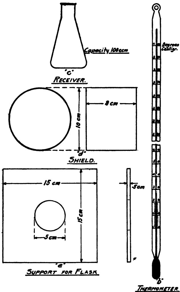
FIG. 357.—National Electric Light Association creosote oil analysis.
