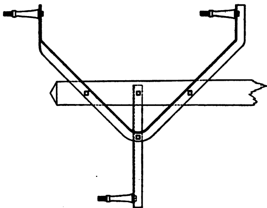
FIG. 90.—Special cross-arm.
