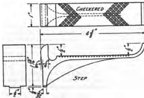
FIG. 370.—Two types of pole step sockets.
