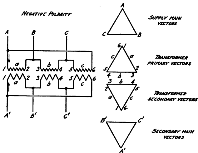
FIG. 201.—Transformers connected "Δ" primary and "Δ" secondary.
