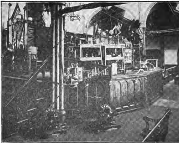
FIG. 22.—Three H. P. Motor and Generator supplying Bank of Lamps and operated by shielding with the hand a Selenium cell from an Acetylene Flame.
