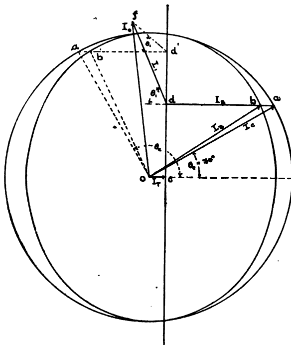
FIG. 16. CONSTRUCTION DIAGRAM FOR BRUSH-SHIFTING CHARACTERISTICS AT NO LOAD.
