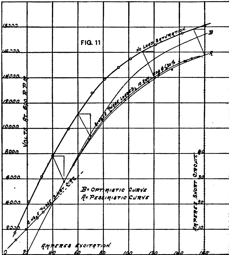
Single-Phase Regulation Curve.
