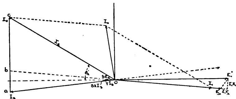
FIG. 22. HEYLAND MACHINE AS GENERATOR
