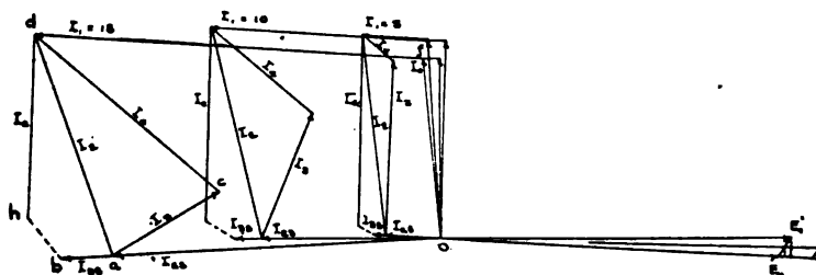
FIG. 30 DIAGRAM FOR TEST No. 14. (DRAWN TO SCALE.)
