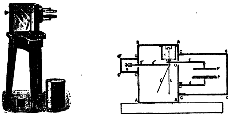
FIG. 5.—Curie's Electroscope for the study of Radio-activity.
