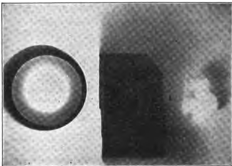
FIG. 6.—Radiograph Made by Radium of a Disc for Testing Radioactivity, a Block of Rock-salt and a Lump of Pitchblende.
