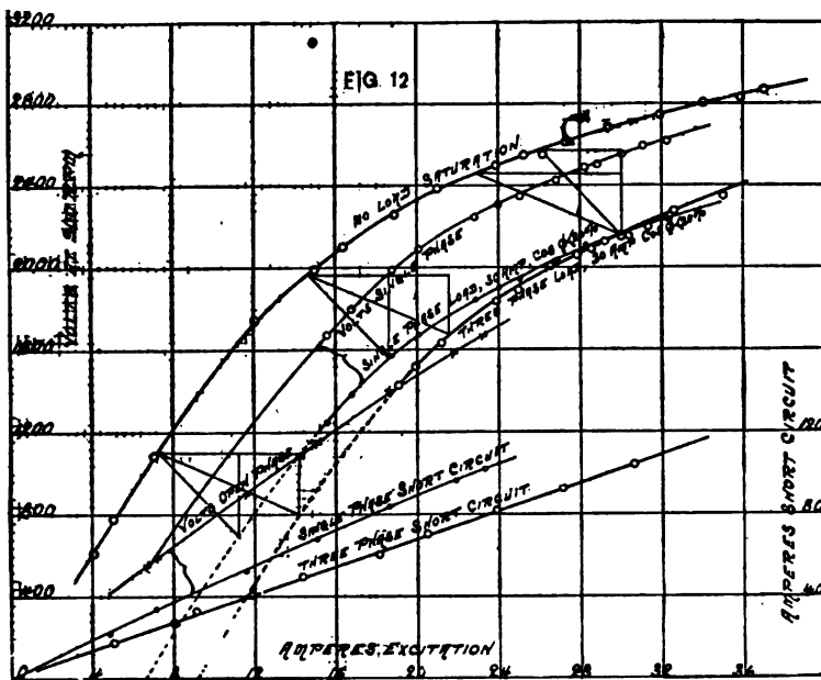
Regulation Curves on 100 k.w. 3-Phase Generator.
