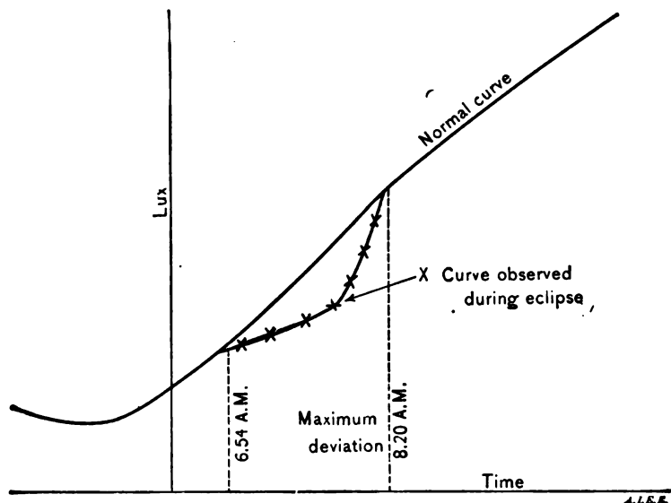
FIG. 30.—Curve Taken with Ruhmer Cell During Eclipse, Oct. 31, 1902.
