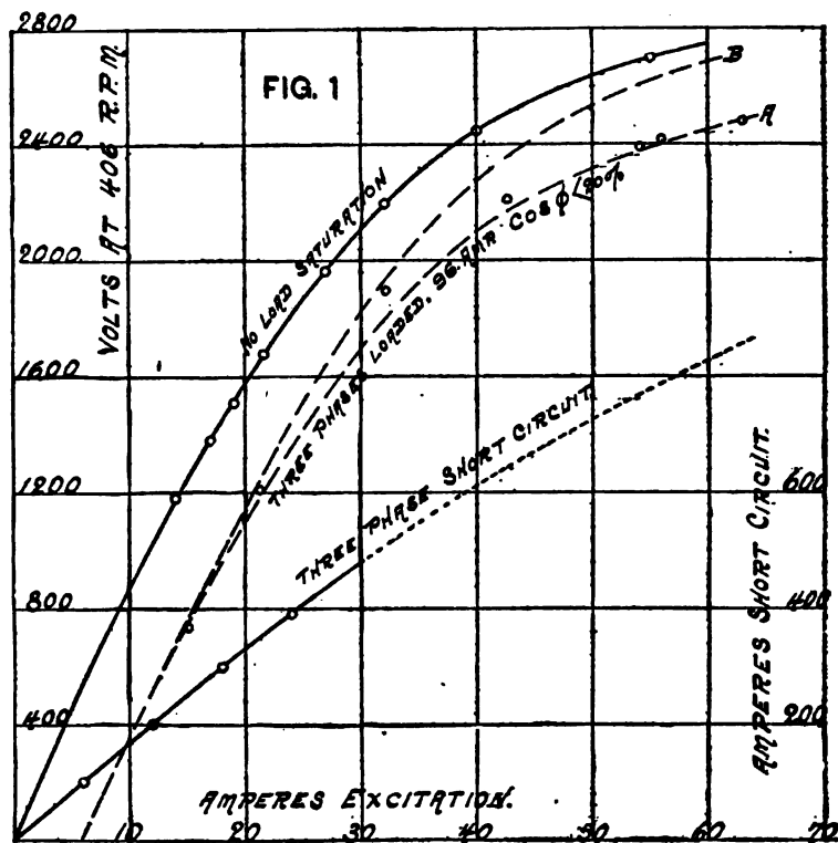
Regulation Curves on 500 k.w. 3-Phase Induction Generator.
