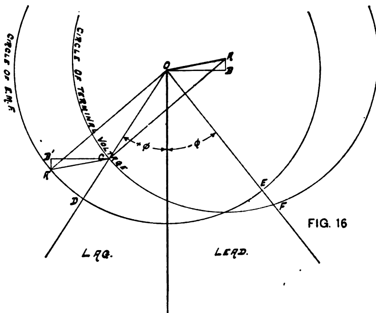
Kapp's Diagram for the Determination of the Regulation at Different Power Factors.
