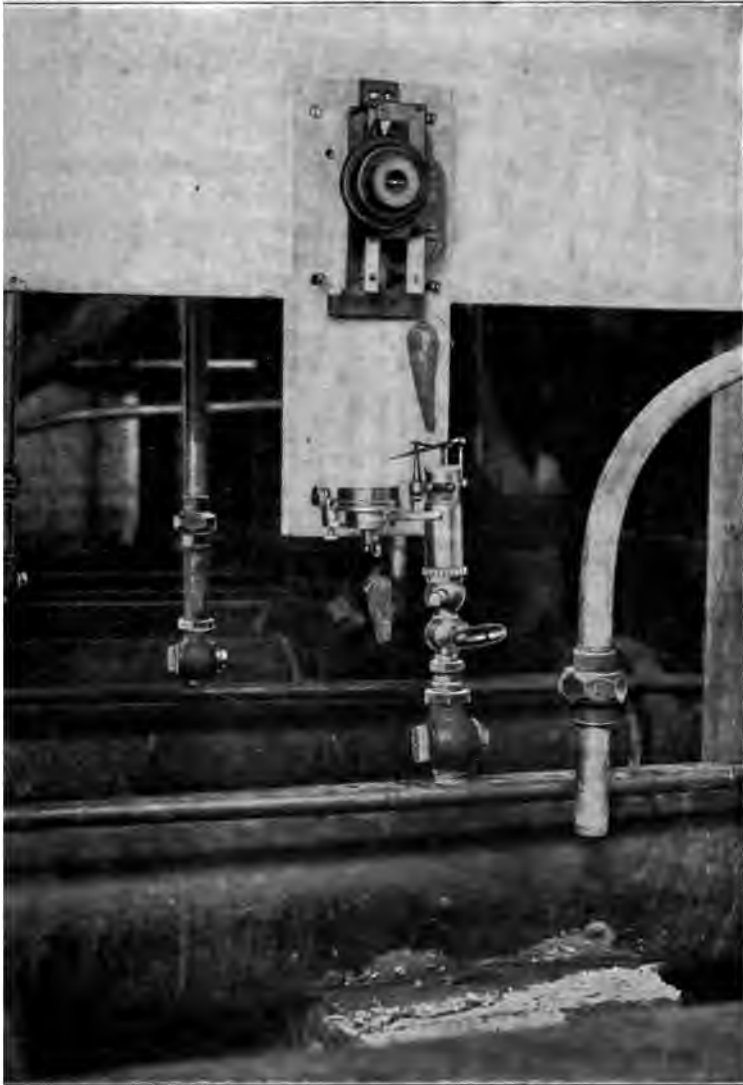
Fig. 210.—APPARATUS FOR TAKING WATER-HAMMER CARDS.
