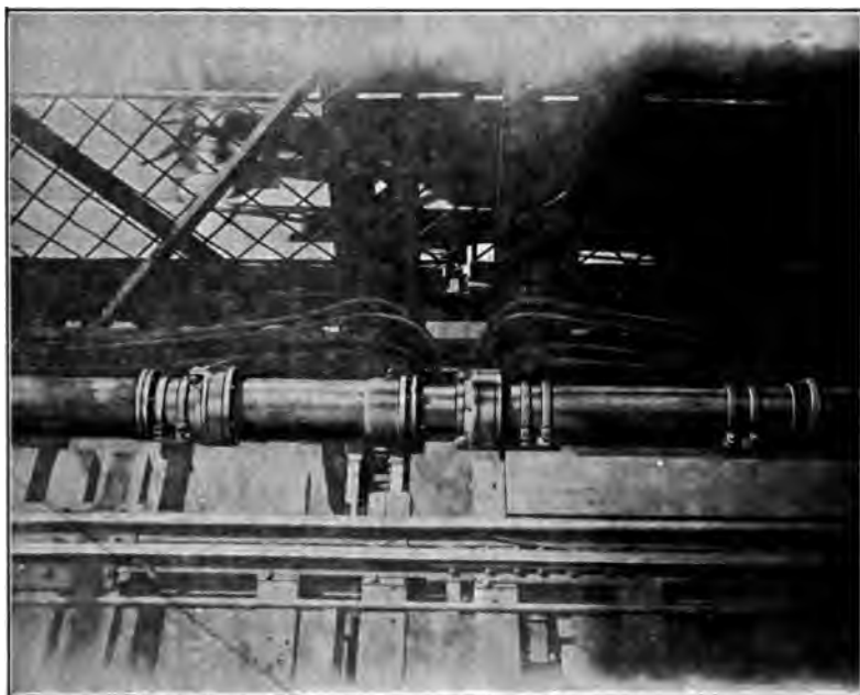
FIG. 185.—EXPANSION JOINT IN THE PNEUMATIC TUBE AT THE CENTER OF THE NEW YORK AND BROOKLYN BRIDGE.
