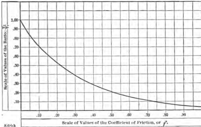
FIG. 41.—SHOWING THE VARIATION OF THE RATIO OF THE BELT TENSIONS WITH THE COEFFICIENT OF FRICTION.
