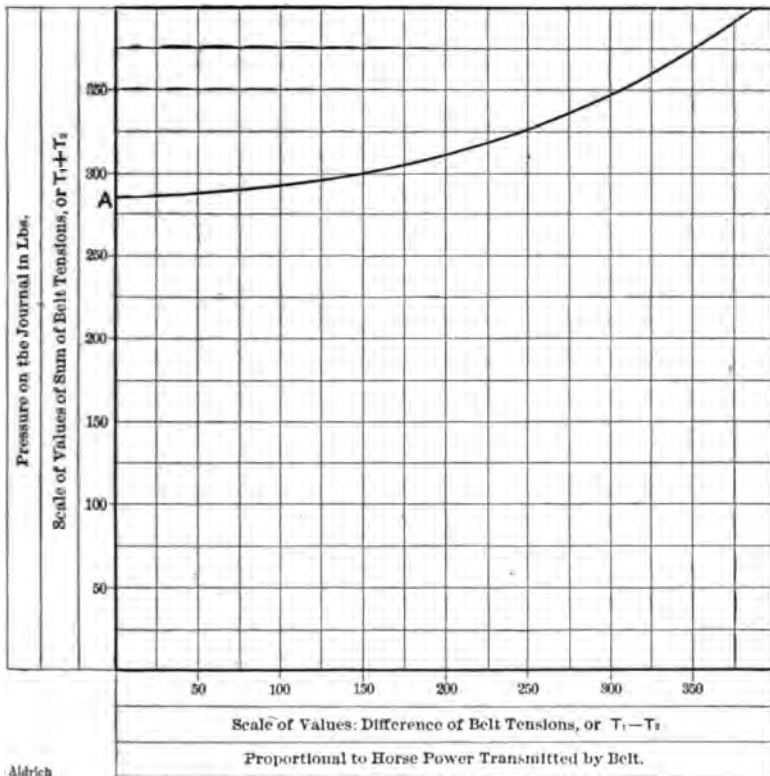
FIG. 40.—SHOWING THE VARIATION OF THE SUM AND THE DIFFERENCE OF THE BELT TENSIONS, OR THE INCREASE OF PRESSURE ON THE JOURNAL AS THE HORSE-POWER TRANSMITTED BY THE BELT IS INCREASED. AT THE POINT "A", THE PRESSURE IS DUE TO THE INITIAL OR LACED TENSION AND THE BELT IS AT REST.
