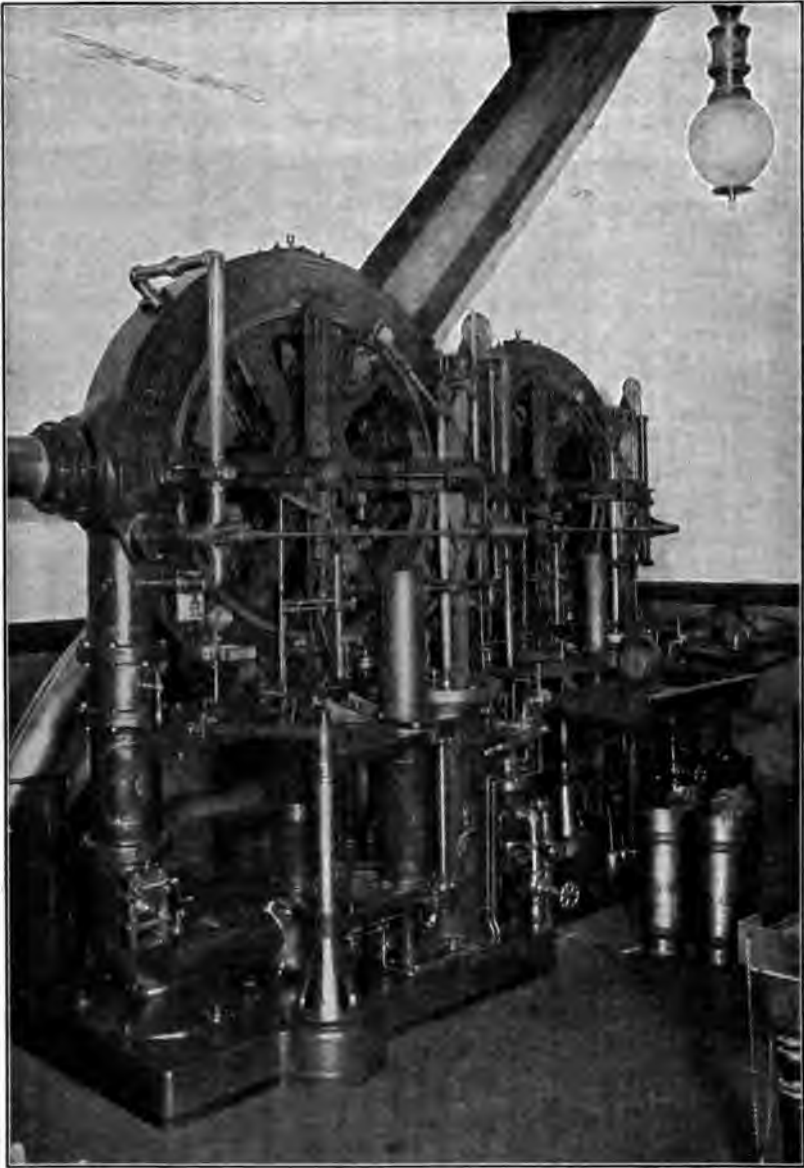
FIG. 132.—MAIL ROOM, READING RAILWAY STATION, PHILADELPHIA, SHOWING PNEUMATIC-TUBE APPARATUS.
