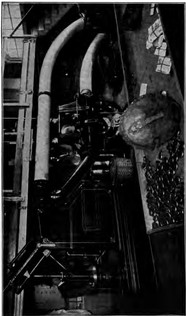
FIG. 188.—PNEUMATIC-TUBE SENDING AND RECEIVING APPARATUS, NORTH UNION RAILWAY STATION, BOSTON, MASS.
