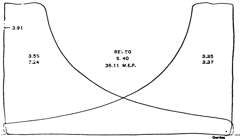
FIG. 358.—STEAM CYLINDER CARD.
