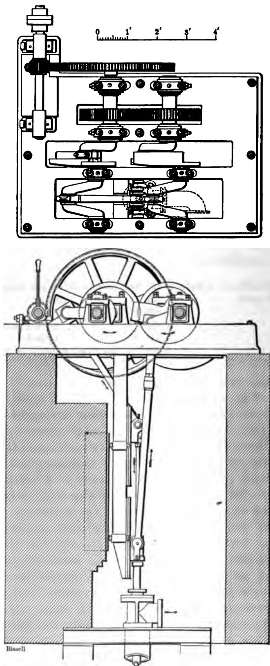
FIG. 253.—JOHNSON CONTINUOUS-FLOW PUMP.
