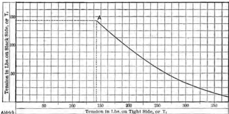
FIG. 39.—SHOWING THE VARIATION OF THE BELT TENSIONS, T_1 AND T_2 , AS THE LOAD IS INCREASED. AT THE POINT "A" THE TENSIONS ARE EQUAL AND THE BELT IS AT REST.
