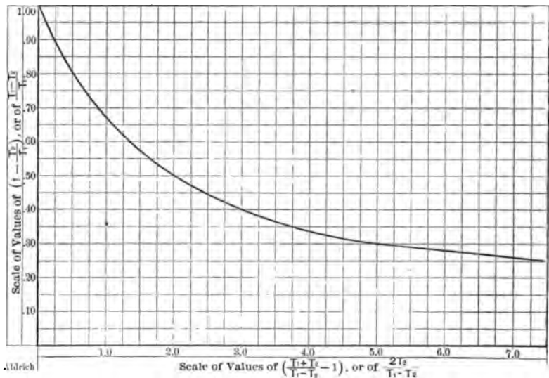
FIG. 43.—SHOWING THE SAME LAW OF VARIATION AS FIG. 42, AND FROM WHICH THE EMPIRICAL FORMULA WAS DERIVED.
