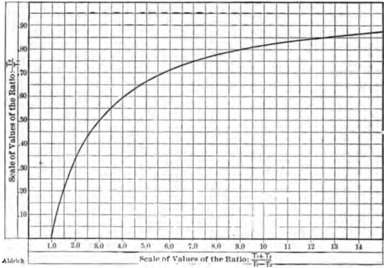
FIG. 42.—SHOWING THE VARIATION OF THE RATIO OF THE BELT TENSIONS WITH THE RATIO OF THEIR SUM AND DIFFERENCE.
