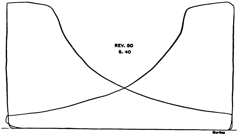
FIG. 357.—STEAM CYLINDER CARD.
