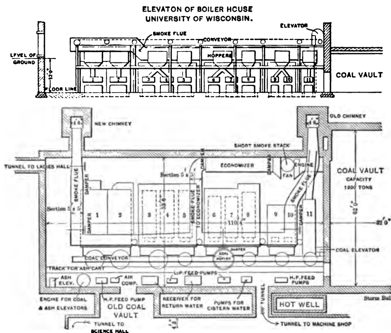
PLAN OF BOILER HOUSE UNIVERSITY OF WISCONSIN.
