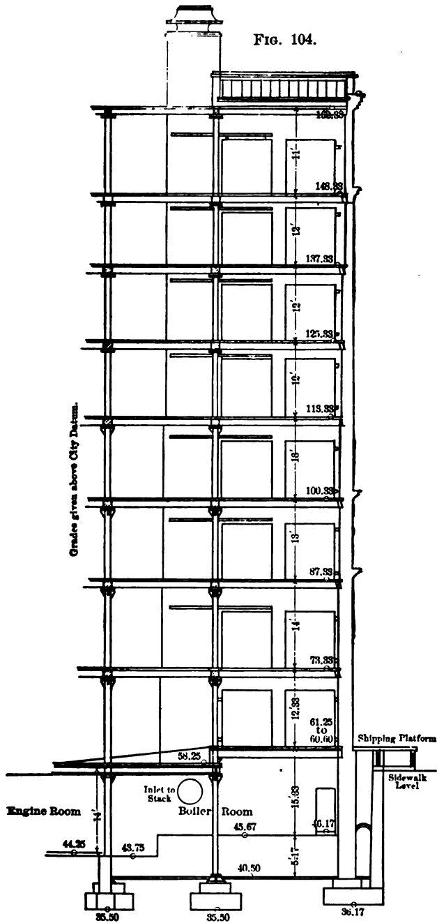
LONGITUDINAL SECTION AT REAR END OF BUILDING LOOKING WEST.
