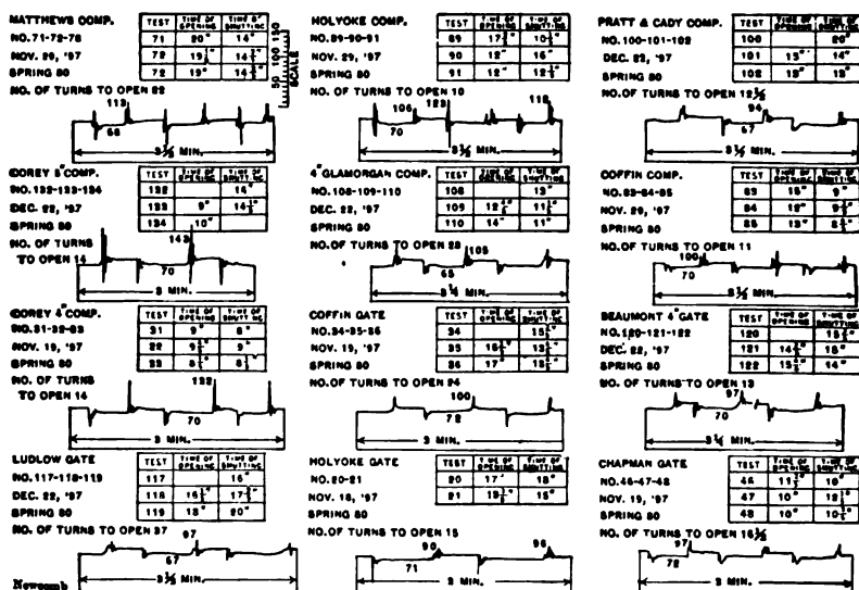
FIG. 211.—WATER-HAMMER CARDS.
