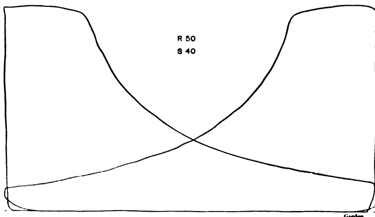
FIG. 354.—STEAM CYLINDER CARD.
