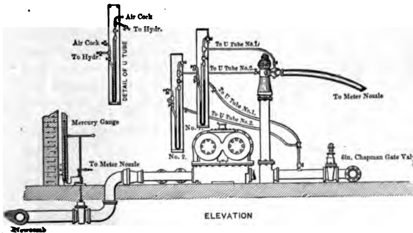
FIG. 155.—PLAN AND ELEVATION OF PIPING, SHOWING THE ARRANGEMENT FOR TESTING OF FIRE HYDRANTS, HOLYOKE, MASS., NOVEMBER, 1897.
