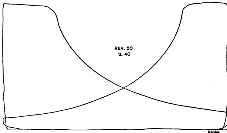
FIG. 356.—STEAM CYLINDER CARD.
