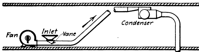
FIG. 10 ARRANGEMENT OF INJECTOR INLET FOR PRESSURE SYSTEM
