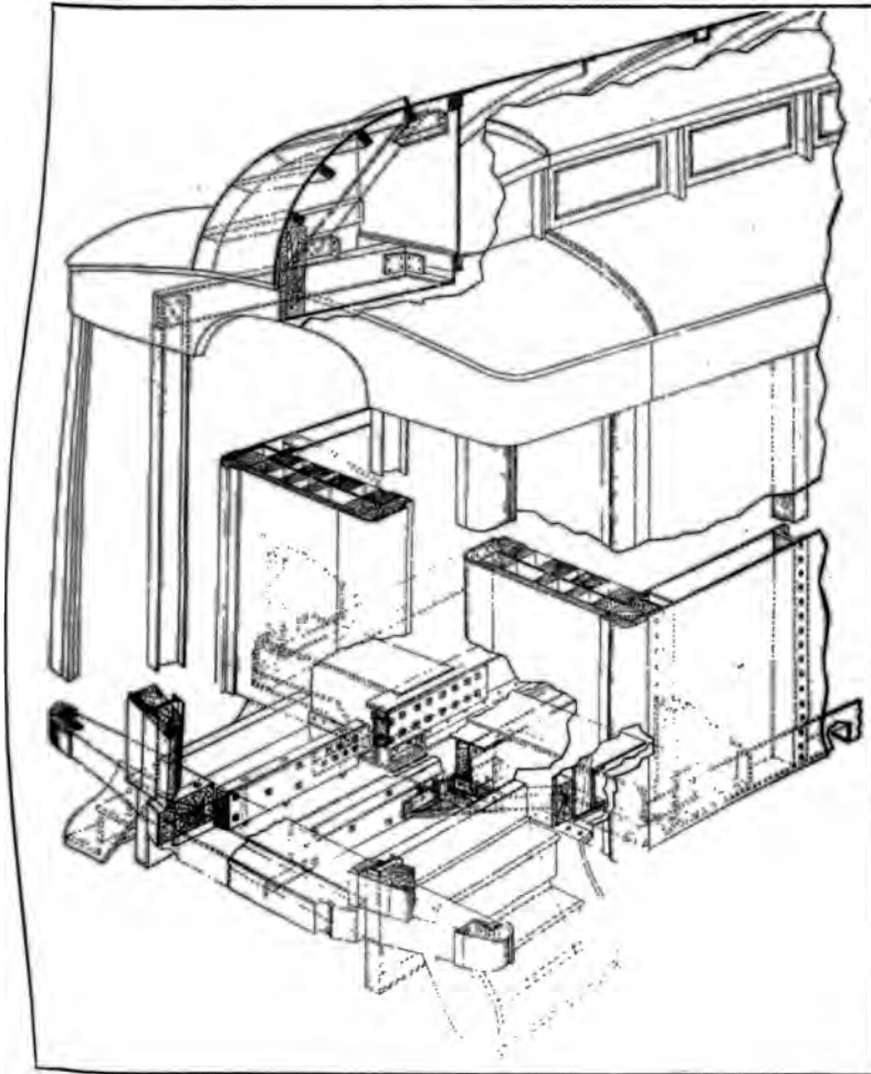
FIG. 14 COLLAPSIBLE VESTIBULE MADE OF A SERIES OF WOODEN POSTS TO SECURE ADVANTAGE OF ELASTIC AND CUSHIONING PROPERTIES OF WOOD
