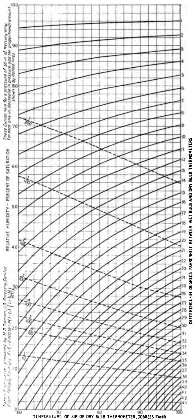
CHART A HUMIDITY CHART
