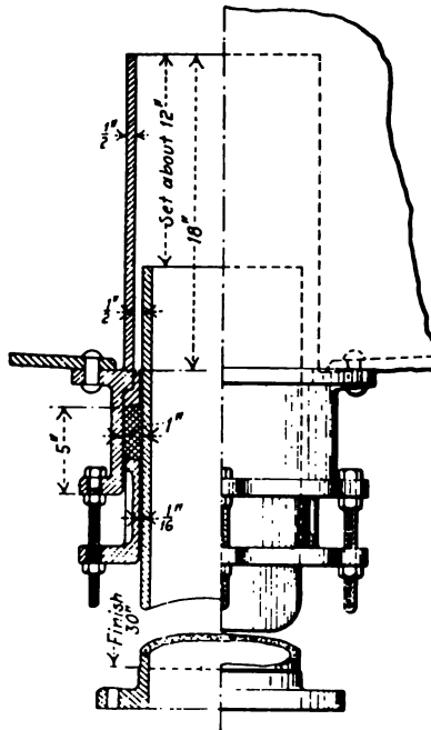
FIG. 13 EXAMPLE OF PROPER DESIGN OF EXPANSION JOINT FOR STEEL TANK
