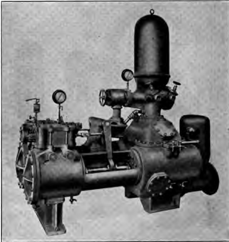
FIG. 10 GENERAL VIEW OF UNDERWRITER STEAM FIRE PUMP
