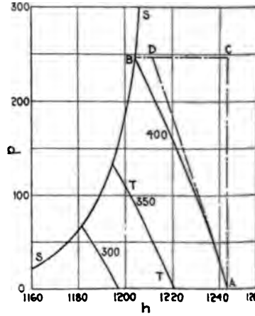
FIG. 2 ISOTHERMALS OF h ON p
