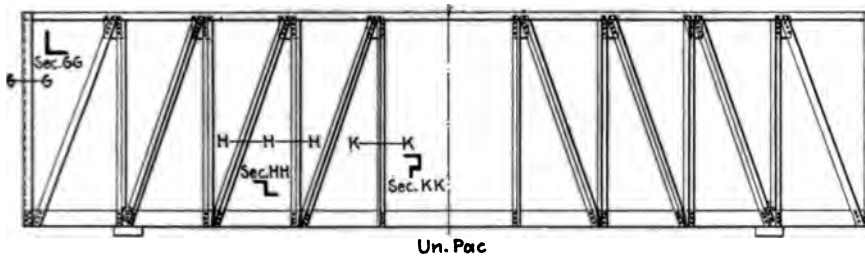
FIG. 7 STEEL FRAMING USED ON THE UN. PAC. CARS HAVING NINE PANELS WITH END PANEL BRACED DIAGONALLY; SIDE DOOR POSTS PREASED STEEL SECTION AND ANGLE IRON
