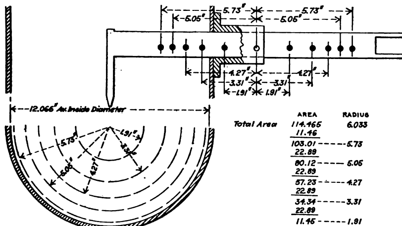
FIG. 6 SKETCH SHOWING POSITIONS AT WHICH READINGS OF VELOCITY HEAD WERE TAKEN
