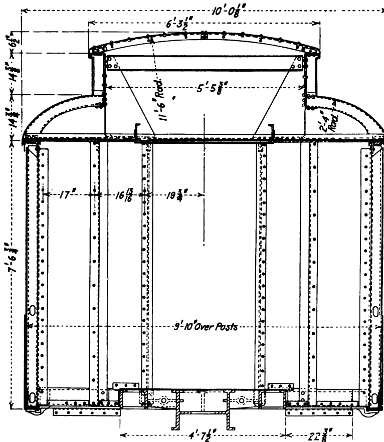
FIG. 10 BODY END FRAMING, TYPE SHOWN IN FIG. 11
