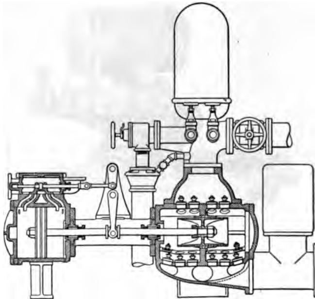
FIG. 8 SECTIONAL VIEW OF UNDERWRITER STEAM FIRE PUMP
