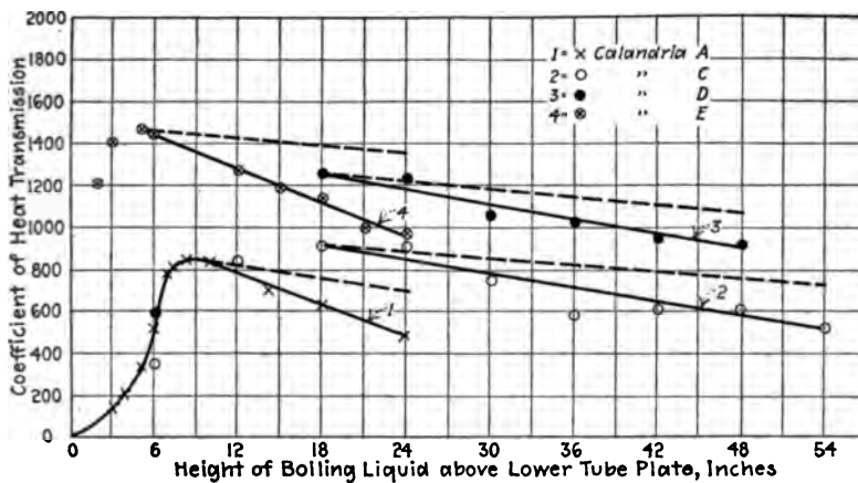
FIG. 9 CURVES SHOWING EFFECT OF HYDROSTATIC HEAD UPON HEAT-TRANSMISSION. FULL LINES PLOTTED FROM TEST; BROKEN LINES DRAWN ACCORDING TO CALCULATIONS BASED UPON THEORETICAL LOSS OF TEMPERATURE FALL DUE TO HYDROSTATIC HEAD
