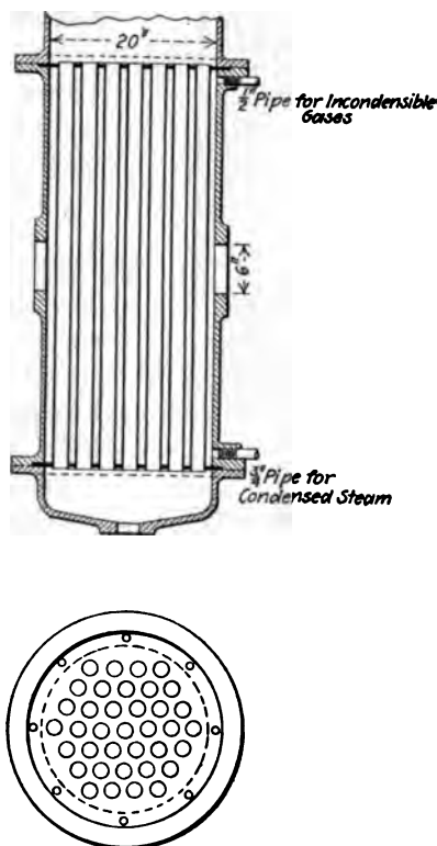
FIG. 5 37 COPPER TUBES 2 IN. BY 48 IN. BY 18 BIRMINGHAM WIRE GAGE. TUBE PLATES \frac{1}{8} IN. COPPER
