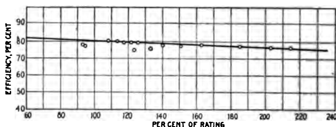
FIG. 4 CURVE SHOWING OVER-ALL EFFICIENCY OF BOILER AND FURNACE AT DIFFERENT RATINGS—TAYLOR-STOKER FIRED UNITS
