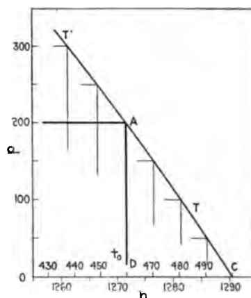
FIG. 9 DETERMINATION OF h - p ISOTHERMAL
