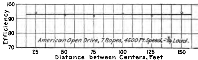
FIG. 8 CURVE SHOWING EFFICIENCY RELATIVE TO VARYING CENTERS
