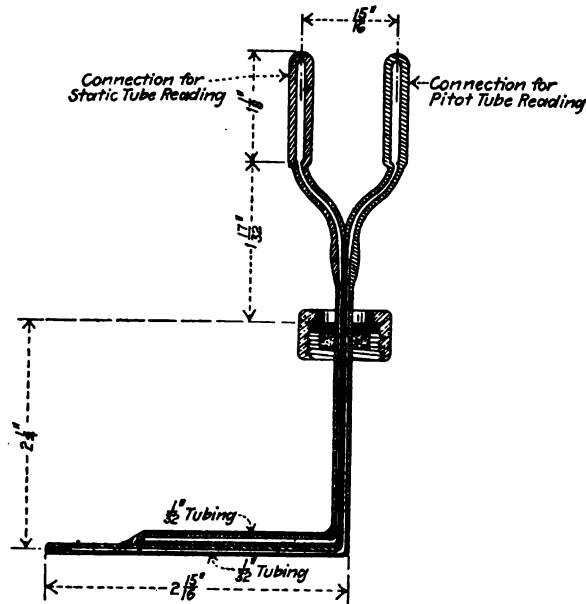
FIG. 3 DETAIL OF PITOT AND STATIC TUBES
