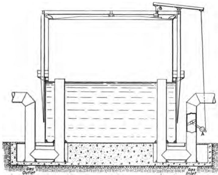
FIG. 3 ARRANGEMENT OF REGULATING VALVE FOR GAS HOLDER
