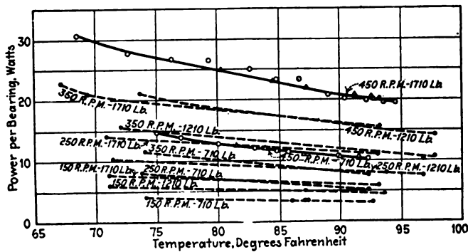
FIG. 9 BALL BEARINGS. POWER-TEMPERATURE CURVES FOR VARIOUS SPEEDS AND LOADS PER BEARING
