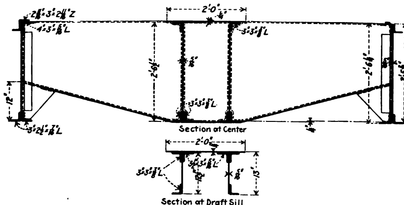
FIG. 1 TYPE a: WEIGHT OF CAR CARRIED EQUALLY ON CENTER AND SIDE SILLS
