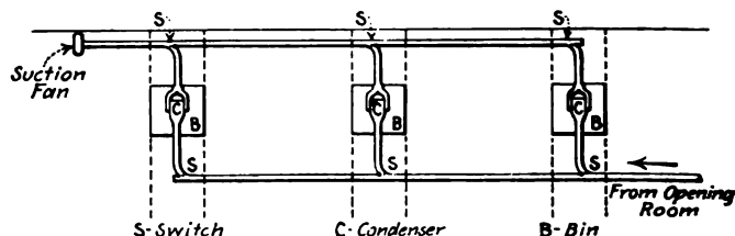
FIG. 9 PLAN SHOWING ARRANGEMENT IN PICKER ROOM WITH MECHANICAL CONVEYOR OMITTED
