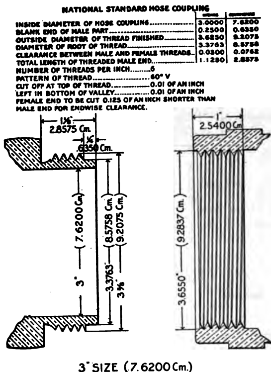
FIG. 2 DETAILS OF 3-IN. COUPLING
