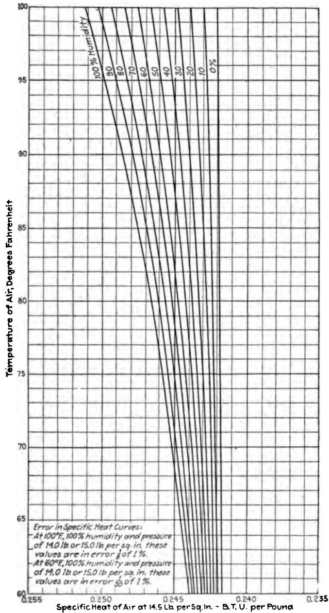
CHART B CHART GIVING THE SPECIFIC HEAT OF MIXTURES OF AIR AND WATER VAPOR AT 14.5 LB. PER SQ. IN. ABSOLUTE PRESSURE FOR VARYING CONDITIONS OF TEMPERATURE AND HUMIDITY
