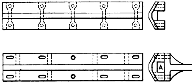
FIG. 3 CHILLER FOR LATHEWAYS
