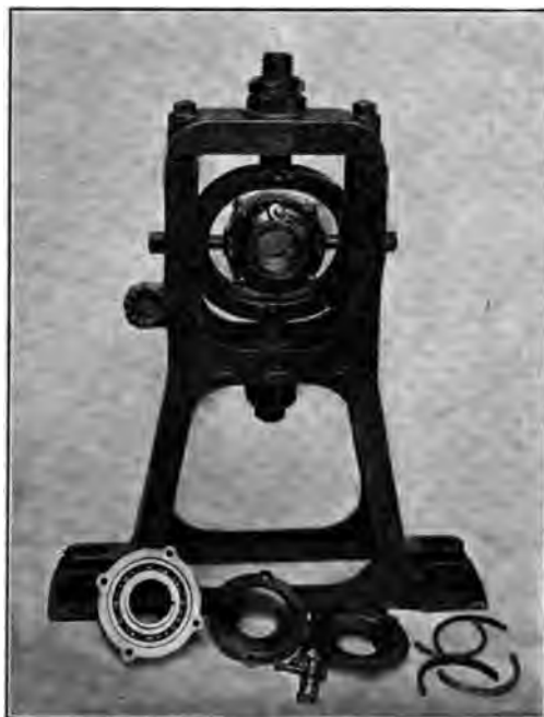
FIG. 6 TYPE OF BALL BEARING USED IN TESTS
