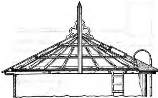
FIG. 4 A GOOD DESIGN OF DOUBLE ROOF FOR ELEVATED TANK
