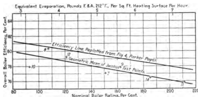
FIG. 12 COMPARATIVE CURVES SHOWING RELATION BETWEEN RESULTS REPORTED BY MR. PARKER AND THOSE OBTAINED IN DR. JACOBUS' TESTS ON THE SAME BOILERS
