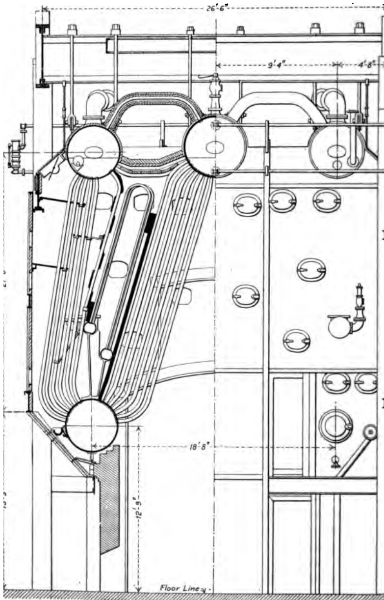
FIG. 6 END SECTION OF BOILER SHOWING ARRANGEMENT OF GAS PASSES
