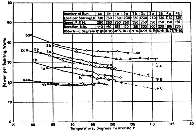
FIG. 37 RABBITS BEARINGS, GRAPHICAL LOGS
