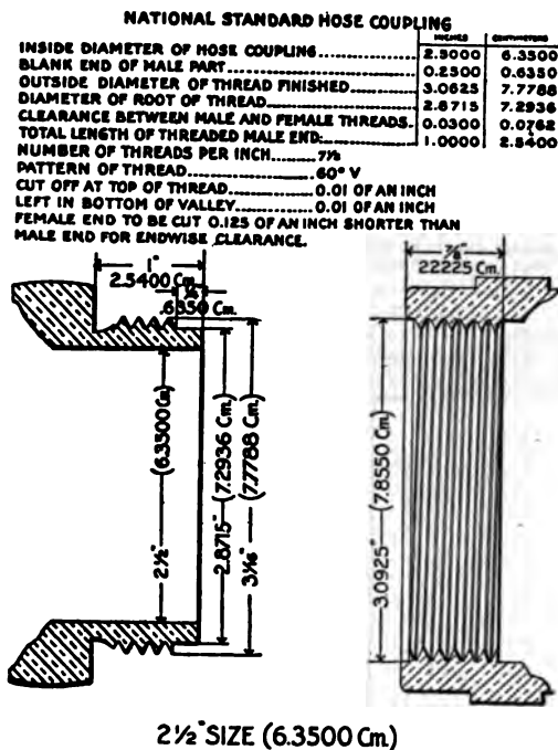
FIG. 1 DETAILS OF 2\frac{1}{2} -IN. COUPLING
