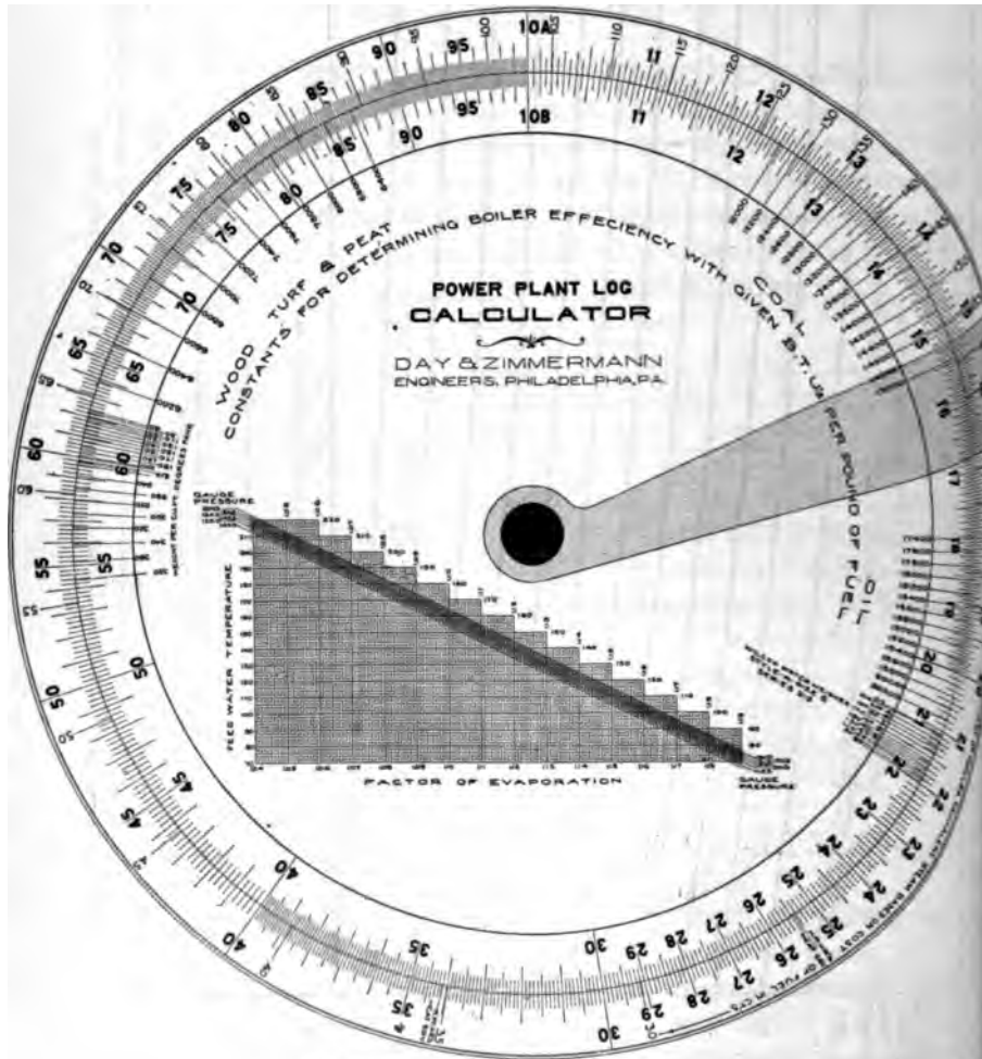
FIG. 5 POWER PLANT LOG CALCULATOR
