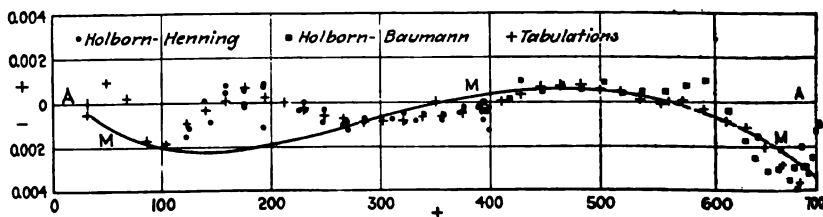
FIG. 10 PRESSURE-TEMPERATURE COMPARISONS
