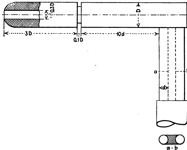
FIG. 30 PRANDTL'S TUBE WITH SPHERICAL END
