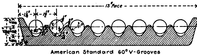
American Standard 60° V-Grooves
