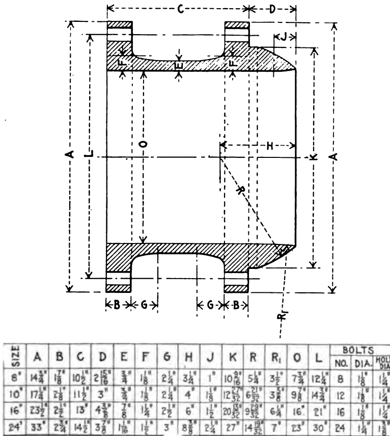
FIG. 12 DETAIL OF VALVE CONNECTING PIECE
