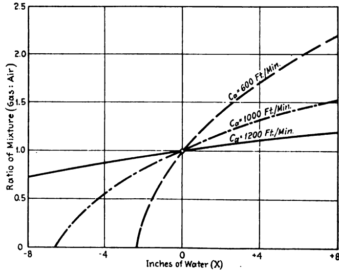
FIG. 4 CURVE SHOWING VARIATIONS IN RATIO OF MIXTURE OF GAS AND AIR WITH DIFFERING VELOCITIES OF AIR DRAWN IN
