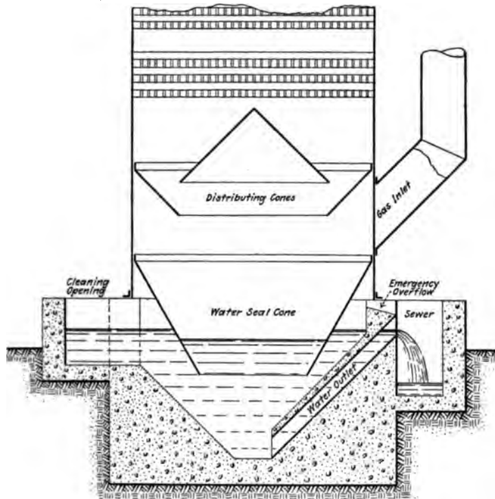
FIG. 2 SCRUBBER BOTTOM
