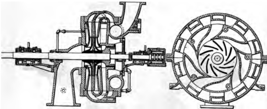
FIG. 12 CENTRIFUGAL FIRE PUMP WITH DIFFUSION VANES
