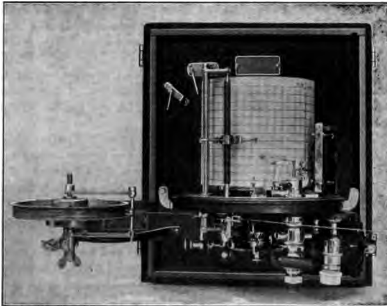
FIG. 3 RECORDING INSTRUMENT
