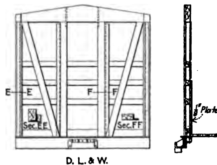
FIG. 19 END FRAMING USED ON D. L. & W. CARS SHOWING CENTER AND CORNER POSTS MADE UP OF ANGLE IRON AND WOOD FILLERS; DIAGONAL BRACES RUN FROM END SILL AT CENTER POSTS TO END PLATE AT CORNER POSTS \frac{1}{2} -IN. END REINFORCING PLATE
