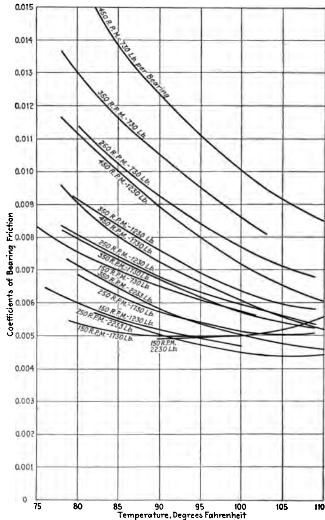
FIG. 10 BABBITT BEARINGS. COEFFICIENT OF FRICTION-TEMPERATURE CURVES FOR VARIOUS SPEEDS AND LOADS PER BEARING
