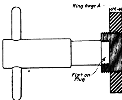
FIG. 1 VIEW OF PLUG AND RING GAGE
