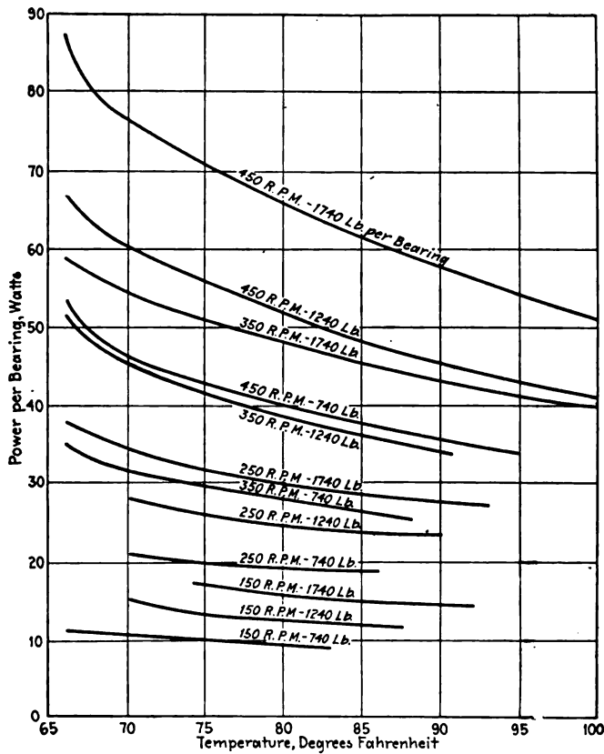
FIG. 8 ROLLER BEARINGS. POWER-TEMPERATURE CURVES FOR VARIOUS SPEEDS AND LOADS PER BEARING
