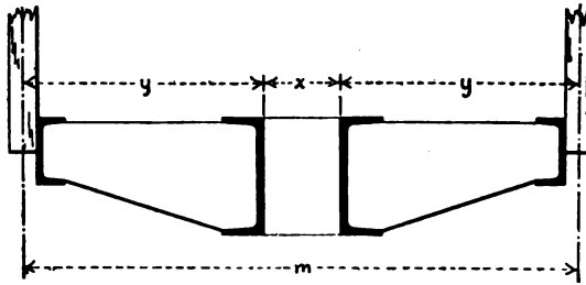
FIG. 30 DIAGRAM FOR LOAD DISTRIBUTION
