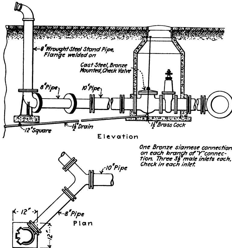
FIG. 4 FIREBOAT CONNECTION
