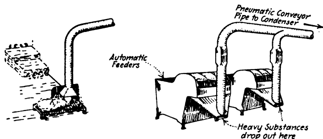
FIG. 7 ARRANGEMENT IN OPENING ROOM WITH BALE BREAKER OMITTED
