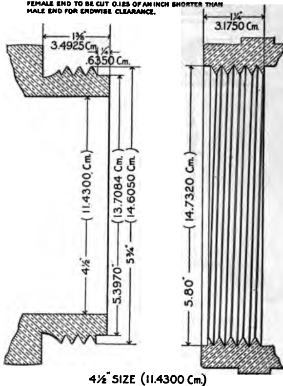
FIG. 4 DETAILS OF 4½-IN. COUPLING
