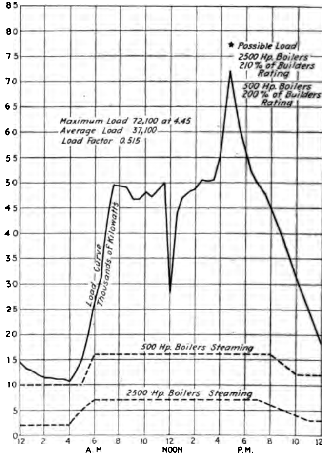
FIG. 2 PEAK LOAD CURVE, DECEMBER 6, 1912
