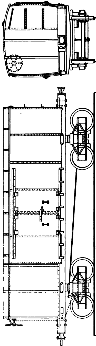
FIG 15 DESIGN OF IRON BOX CAR BUILT BY THE BALTIMORE & OHIO R. R. IN 1862
