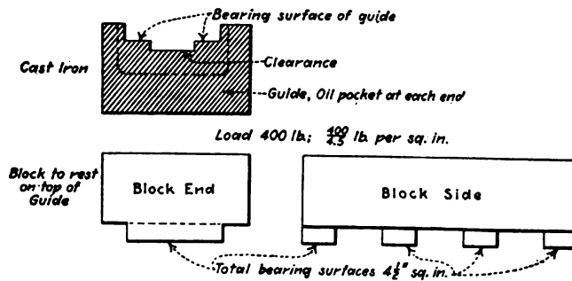
FIG. 4 BLOCK AND GUIDE FOR TESTING RUBBING SURFACES
