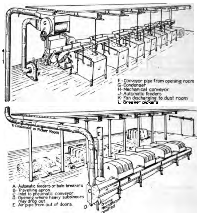
FIG. 6 SUCTION PNEUMATIC SYSTEM TAKING COTTON FROM AN OPENING ROOM AND DELIVERING TO A MECHANICAL CONVEYOR FOR DISTRIBUTION
