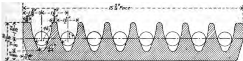
Engineers' Standard 45° V-Grooves
