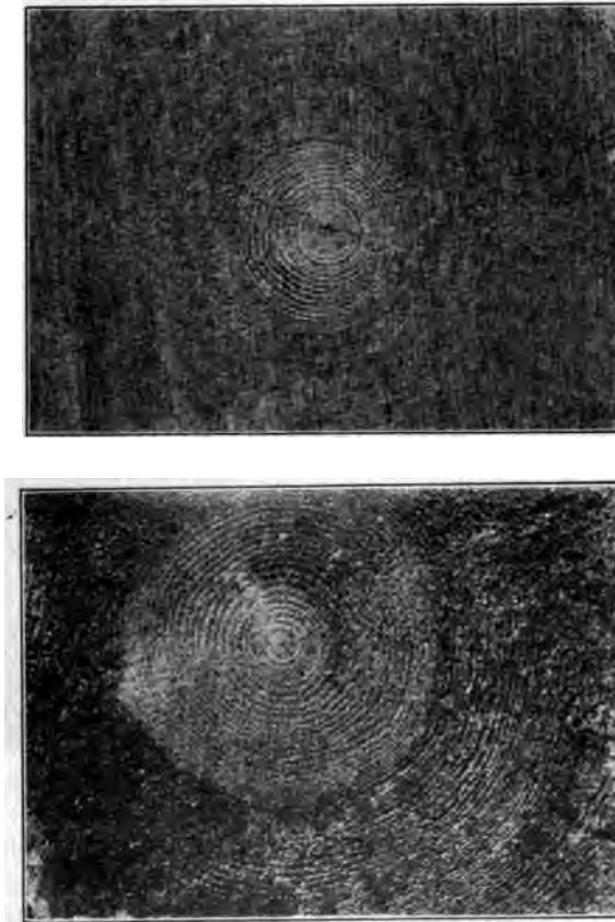
FIG. 4 SOUND AND ROTTED SECTIONS OF 12 IN. BY 14 IN. BEAMS; PROBABLY SHORTLEAF PINE
