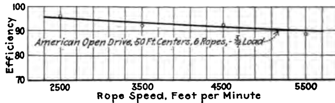
FIG. 7 RESULTS OBTAINED IN AMERICAN OPEN DRIVE TEST WITH EFFICIENCY PLOTTED AGAINST SPEED
