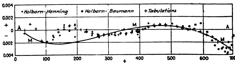
FIG. 10 PRESSURE-TEMPERATURE COMPARISONS
