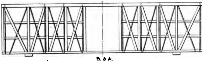
FIG. 4 SIDE FRAME USED ON B. & A. CARS HAVING NINE PANELS WITH WOOD POSTS AND DIAGONAL ROD BRACING
