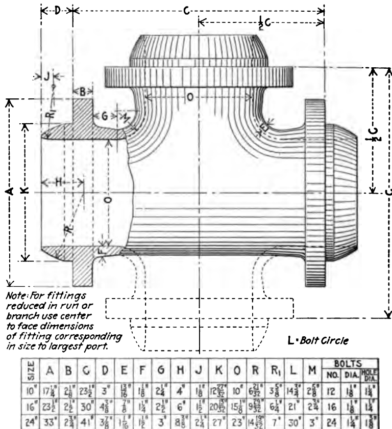
FIG. 11 DETAIL OF TEES AND CROSSES
