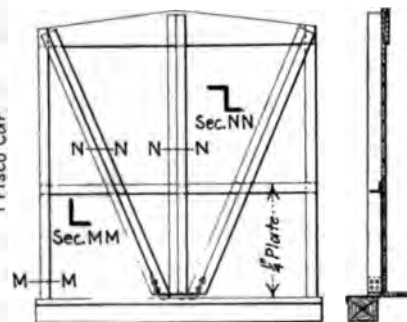
FIG. 25 STEEL END FRAMING, M. C. B. RECOMMENDED DESIGN WITH SINGLE Z-BAR CENTER POST; DIAGONAL BRACES RUN FROM END SILL AT CENTER TO END PLATE AND \frac{1}{4} -IN. END REINFORCING PLATE AT BOTTOM
