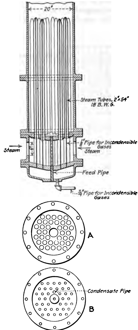
FIG. 6 38 COPPER HEATING TUBES 2 IN. BY 54 IN. BY 18 BIRMINGHAM WIRE GAGE. TOTAL HEATING SURFACE 86.21 SQ. FT.
