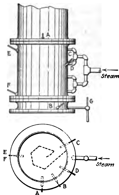
FIG. 8 DIAGRAM SHOWING LOCATION OF THERMOMETERS CALANDRIA E
