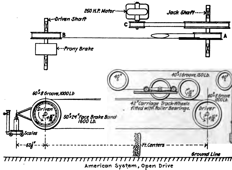
FIG. 3 GENERAL PLAN OF AMERICAN OPEN DRIVE SYSTEM
