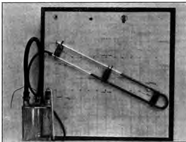
FIG. 28 INCLINED MANOMETER
