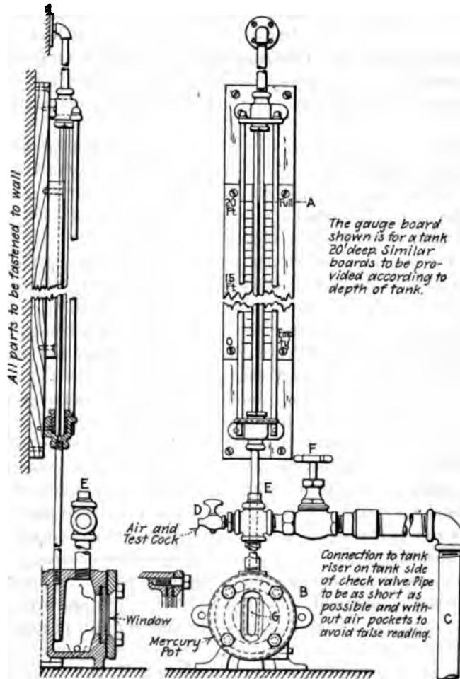
FIG. 16 DETAILS OF MERCURY GAGE FOR INDICATING WATER LEVEL IN TANK
