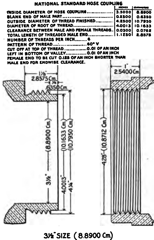
FIG. 3 DETAILS OF 3 1/2-IN. COUPLING
