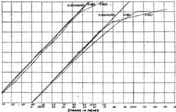
3 CURVES OF TANGENTIAL EXTENSION, SOLID SHEETS, AT MIDDLE LENGTH OF COURSES C AND D , RIGHT AND LEFT SIDES OF BOILER
