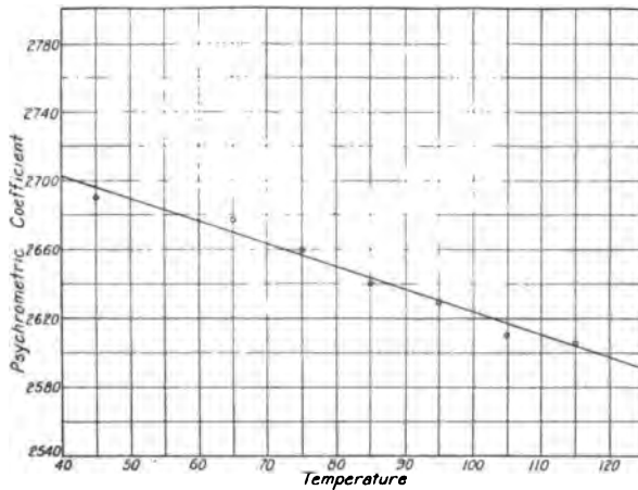
FIG. 7 PSYCHROMETRIC COEFFICIENT
