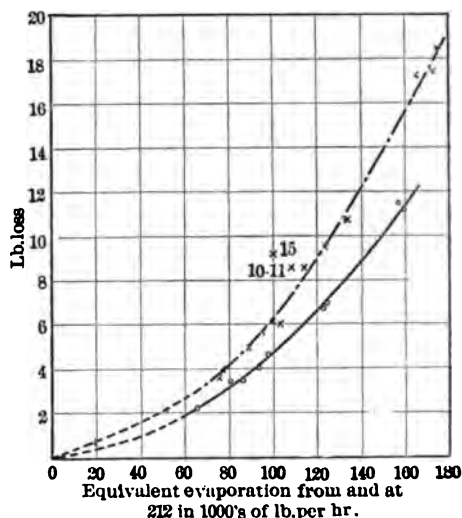
FIG. 12 LOSS OF PRESSURE THROUGH SUPERHEATER AND EQUIVALENT EVAPORATION Points 15 and 10-11 include banking
