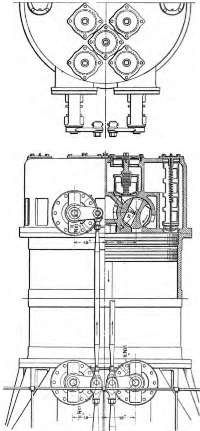
Fig. 16 BLOWING CYLINDER WITH COMBINATION INLET AND OUTLET V A (MESTA)
