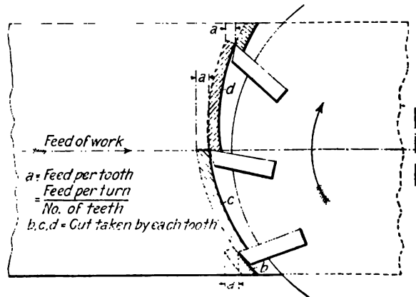
FIG. 45 ACTION OF A FACE CUTTER
