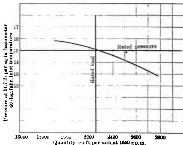
FIG. 6 FACTORY TEST. SHOWING PRESSURE PLOTTED AGAINST QUANTITY OF AIR. 1650 R.P.M.
