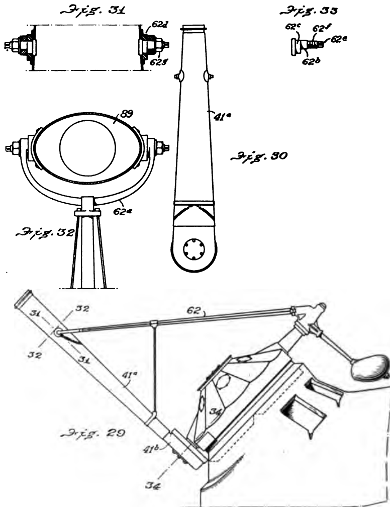
FIGS. 29 TO 33 DIAGRAMS SHOWING ONE OF THE MANY POSSIBLE MODIFICATIONS OF DECLINATION CONTROL
