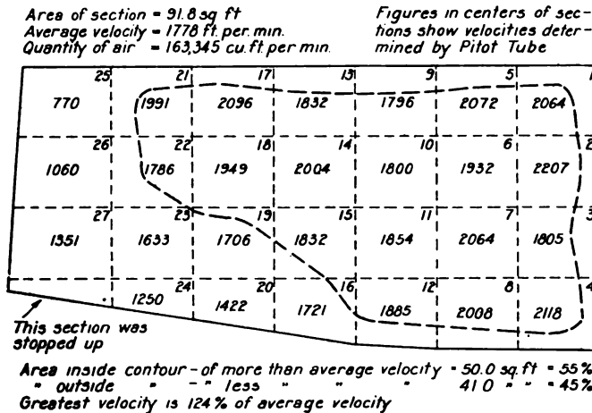
FIG. 14 SECTION AND VELOCITIES IN AIRWAY, FAN TEST No. 10
