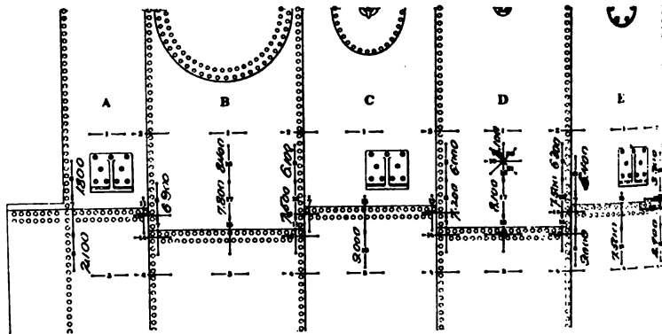
FIG. 38 TANGENTIAL STRESSES, LB. PER SQ. IN., AT 90 LB. BOILER PRESSURE. RESULTS BASED ON RESILIENCES. RIGHT SIDE OF BOILER. NORMAL COMPUTED STRESS, 8640 LB. PER SQ. IN.
