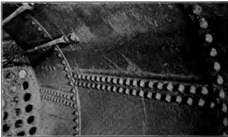
FIG. 4 INTERIOR VIEW OF BOILER NO. 4084 AFTER 295 LB. PRESSURE SHOWING SCALE DISTURBED IN VICINITY OF THE LONGITUDINAL SEAMS
