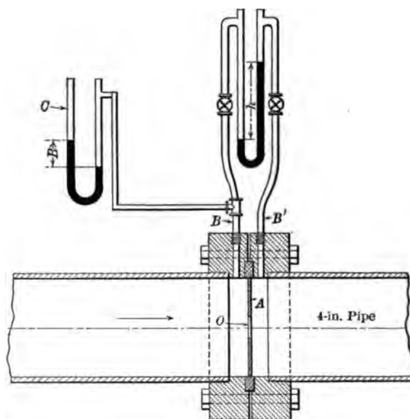
FIG. 13 STANDARDIZED ORIFICE HELD BETWEEN TWO FLANGES IN FUEL SUPPLY LINE
