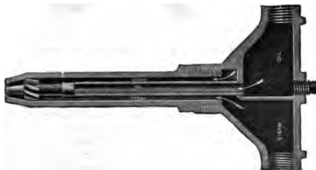
FIG. 5 GEM OIL BURNER
