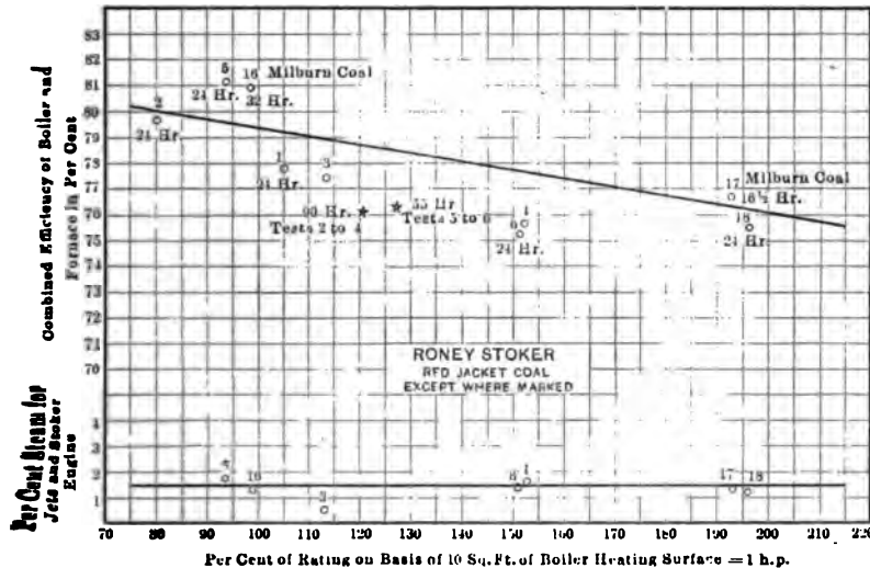
FIG. 4 RESULTS OF TESTS OF BOILER WITH RONEY STOKER
