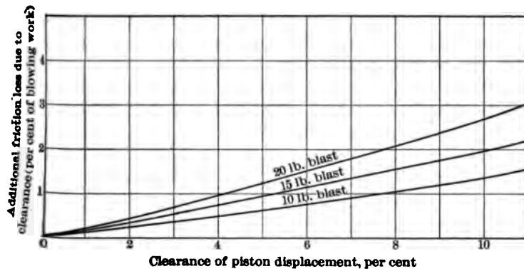
FIG. 33 ADDITIONAL FRICTION LOSS DUE TO CLEARANCE IN BLOWING ENGINES. BASED ON 85 PER CENT MECHANICAL EFFICIENCY OF ENGINE WITHOUT CLEARANCE
