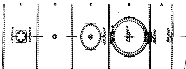
FIG. 46 TANGENTIAL STRESSES, LB. PER SQ. IN., AT 270 LB. BOILER PRESSURE. RESULTS BASED ON RESILIENCES. TOP OF BOILER. NORMAL COMPUTED STRESS, 25,920 LB. PER SQ. IN. GAGED LENGTHS ON WHICH DECIDED PERMANENT SETS OCCURRED, INDICATED BY A STAR
