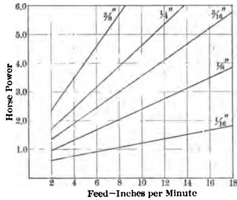
FIG. 35 TESTS OF SPIRAL NICKED MILLING CUTTER 3 1/2 IN. DIAMETER, 14 TEETH, AND ABOUT 1/4 IN. PITCH. CUTTING MACHINE STEEL: 0.50 MANGANESE, 20 CARBON, 55,000 LB. TENSILE STRENGTH. WIDTH OF CUT 6 IN., REDUCED TO BASIS OF 1 IN.
