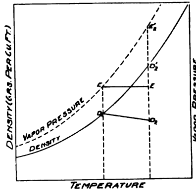
FIG. 3 TEMPERATURE-DENSITY DIAGRAM
