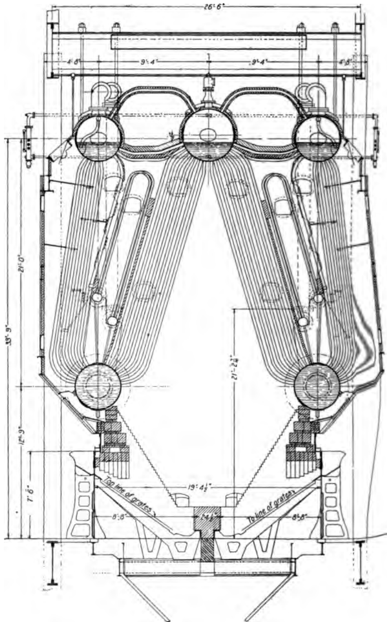
FIG. 2 LONGITUDINAL SECTION OF BOILER FITTED WITH RONNEY STOKER
