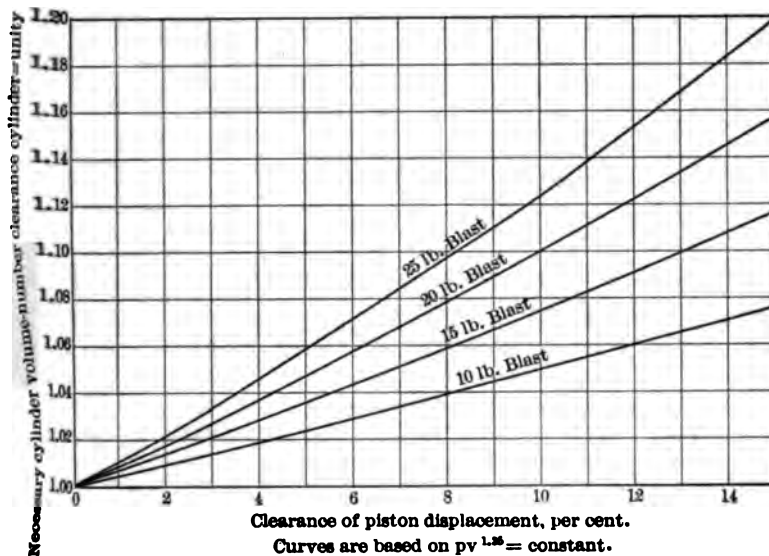
FIG. 30 INFLUENCE OF VOLUME OF CLEARANCE SPACE UPON PISTON DISPLACEMENT OF BLOWING ENGINES
