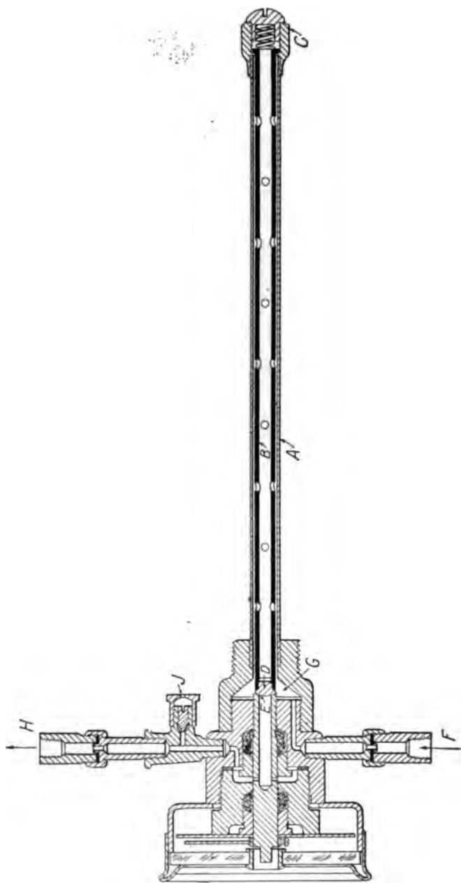
FIG. 12 DEWPOINT THERMOSTAT
