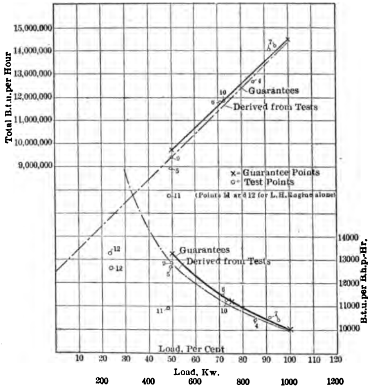
FIG. 2 ECONOMIES AND GUARANTEES, 1000-Kw. ELECTRIC UNIT
