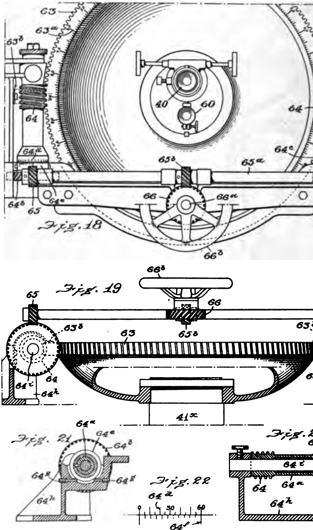
FIGS. 18 TO 22 VARIOUS VIEWS OF DECLINATION WORMWHEEL AND ITS CONTROL BY The form of the wheel and its connection to the arbor is not ideal, but may be very in any later work.
