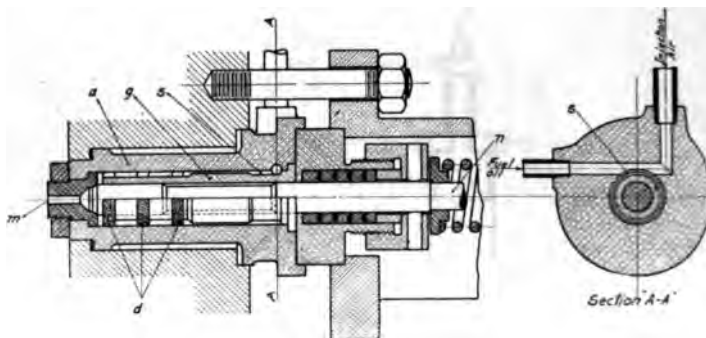
FIG. 14 ATOMIZER OF TYPE FH DE LA VERGNE ENGINE
