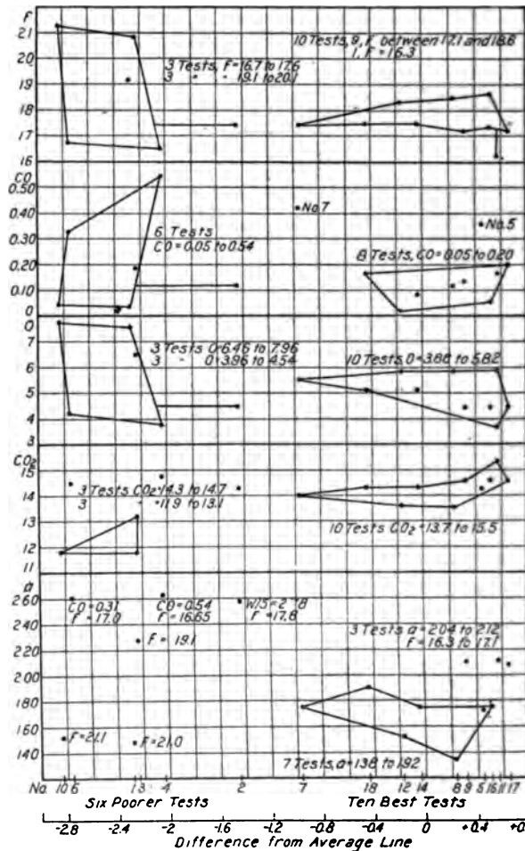
FIG. 25 RELATION OF THE VARIATION OF EFFICIENCY TO f , CO , O
