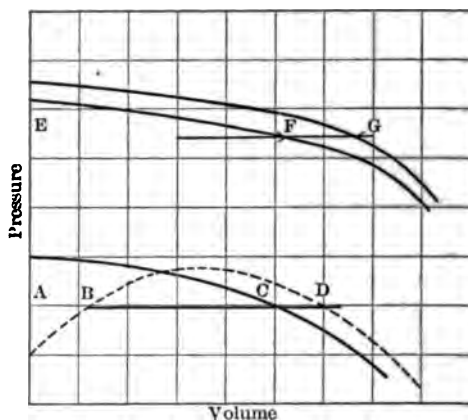
FIG. 8 CHARACTERISTICS REQUIRED FOR PARALLEL OPERATION OF BLOWERS
