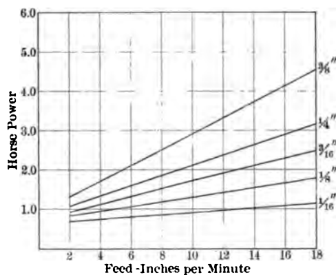
FIG. 39 TESTS OF HELICAL MILLING CUTTER 3\frac{7}{8} IN. DIAMETER, 4\frac{1}{2} IN. LEAD, 10 IN. PITCH. CUTTING CAST IRON, CORRECTED FOR HARDNESS. WIDTH OF CUT 6 IN., REDUCED TO BASIS OF 1 IN.
