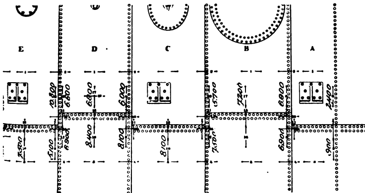
FIG. 41 TANGENTIAL STRESSES, LB. PER SQ. IN., AT 90 LB. BOILER PRESSURE. RESULTS BASED ON RESILIENCES. LEFT SIDE OF BOILER. NORMAL PUT STRESS, 8,640 LB. PER SQ. IN.
