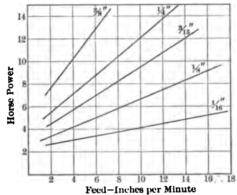
8 TESTS OF SPIRAL NICKED MILLING CUTTER 6 IN. IN DIAMETER; TEETH AND ABOUT 1\frac{1}{8} IN. PITCH. CUTTING CAST IRON, CORRECTED FOR HARD- WIDTH OF CUT 6 IN.
