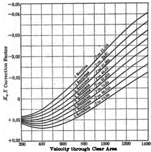
FIG. 38 CORRECTION FACTORS FOR COEFFICIENT OF HEAT TRANSMISSION
