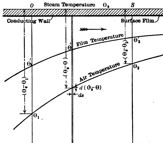
FIG. 29 IDEAL DIAGRAM ILLUSTRATING THE THEORY OF HEAT TRANSMISSION
