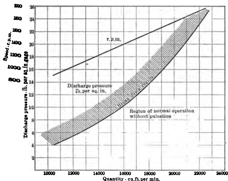
FIG. 5 CURVE OF BREAKDOWN POINTS FROM FACTORY TESTS. PRESSURE AND R.P.M. PLOTTED AGAINST CU. FT. PER MIN.
