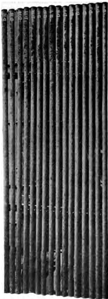
FIG. 7 APPEARANCE OF TUBES, BOILER NO. 4084, AFTER DISMANTLING. HORIZONTAL ROW D, FOURTH FROM TOP
