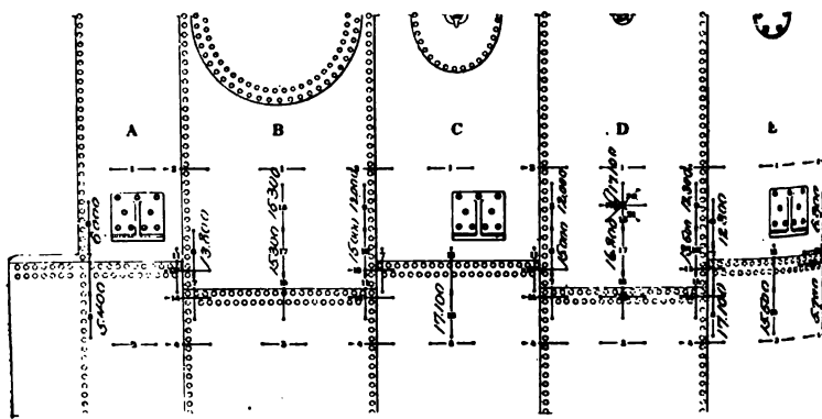
FIG. 39 TANGENTIAL STRESSES, LB. PER SQ. IN., AT 180 LB. BOILER PRESSURE. RESULTS BASED ON RESILIENCES. RIGHT SIDE OF BOILER. NORMAL COMPUTED STRESS, 17,280 LB. PER SQ. IN.
