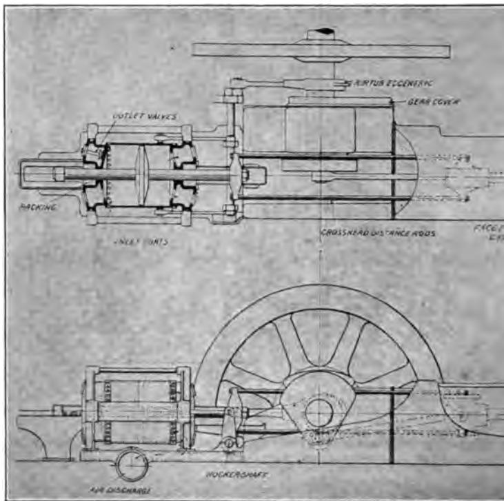
FIG. 15a BLOWING TUB WITH MOVABLE CYLINDER (SLICK DESIGN) 1 WESTINGHOUSE MACHINE COMPANY
