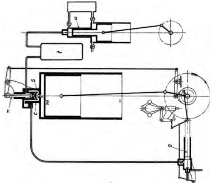
FIG. 16 DIESEL ENGINE WITH "OPEN" INJECTION NOZZLE
