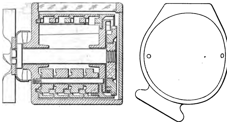
FIG. 5 VEEDER CYCLOMETER WITH SECTION VIEW
