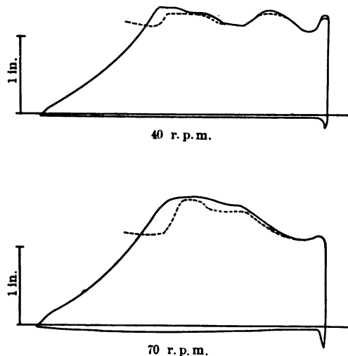
FIG. 17 INDICATOR CARDS TAKEN FROM ENGINE SHOWN IN FIG. 16
