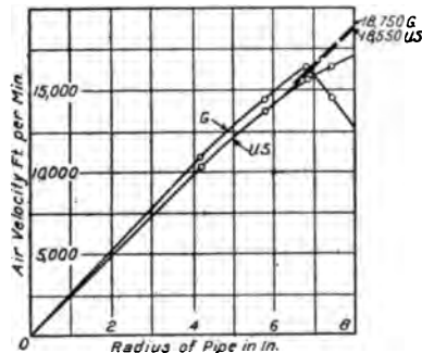
FIG. 17 RADIUS OF PIPE AND AIR VELOCITY DIAGRAM
