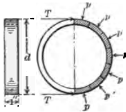
FIG. 1 ANNULUS OF UNIT LENGTH AT THE MIDDLE OF A LONG CIRCULAR TUBE
