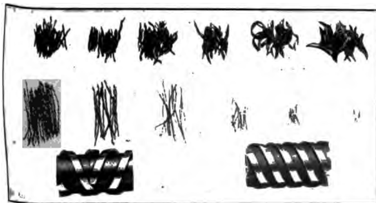
FIG. 20 HELICAL CUTTERS, SINGLE AND INTERLOCKED, AND CHIPS PRODUCED BY THEM
