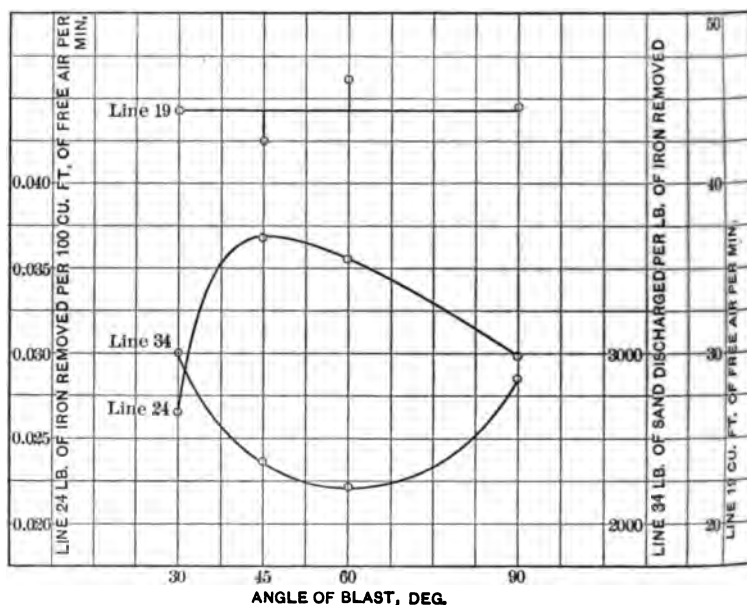
FIG. 8 RESULTS OF TESTS IN RELATION TO ANGLE OF BLAST
