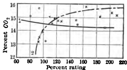
FIG. 16 PER CENT RATING AND PER CENT \text{CO}_2 Point 15 includes 7\frac{1}{2} hours banking. Curve 1 indicates Roney Stoker, Curve 2 Taylor Stoker
