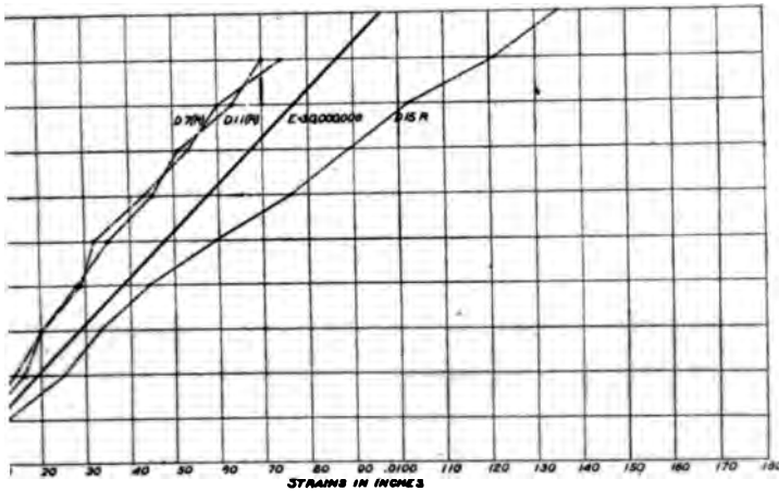
26 CURVE OF TANGENTIAL RESILIENCE, ACROSS LONGITUDINAL SEAM, D, RIGHT SIDE OF BOILER, AT MIDDLE OF COURSE AND NEAR GIRTH
