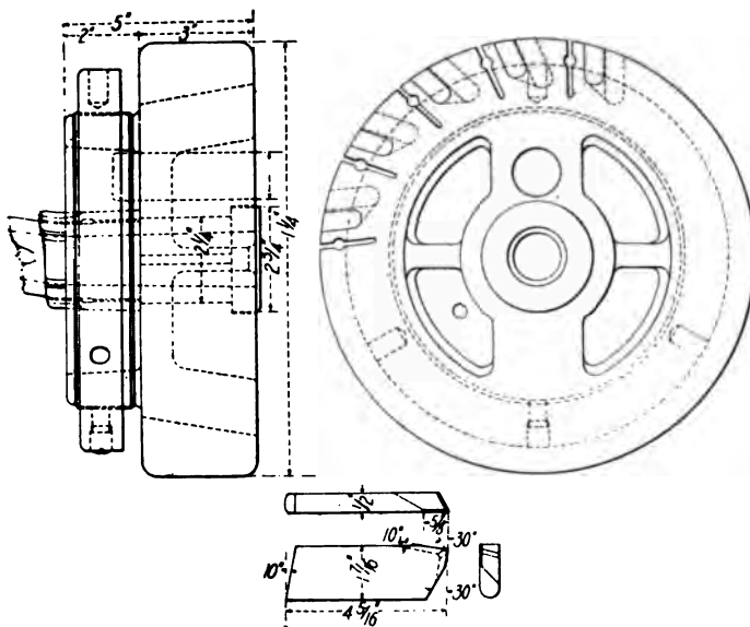
FIG. 50 PRESENT STYLE INSERTED TOOTH FACE CUTTER
