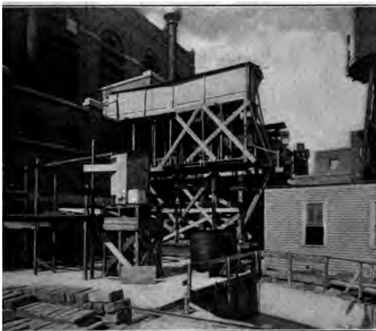
FIG. 8 SPECIAL APPARATUS FOR WEIGHING FEEDWATER
