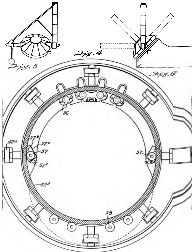
FIG. 4 SECTION THROUGH THE TURRET INDICATED BY LINE 4—4, FIG. 1
