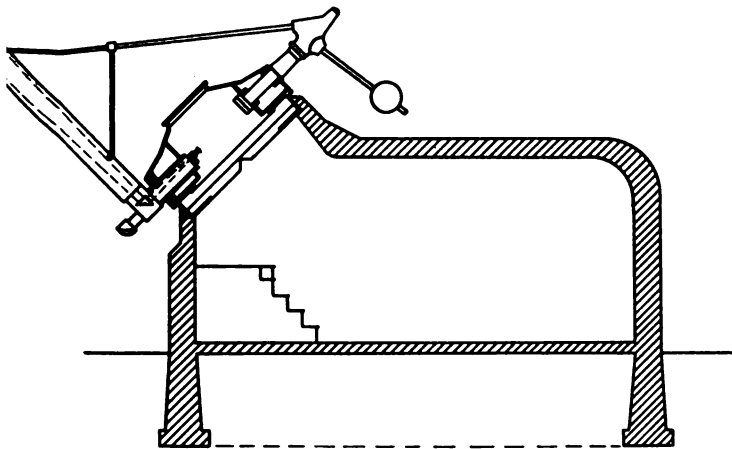
FIG. 3A TURRET EQUATORIAL Object glass, 10 in. in diameter with 15:1 focal length, 2½-in. prism at bend, which is approximately distance from eyepiece to objective. Actual size of beam of light is 2½ in. at this point, or less in the area of objective.
