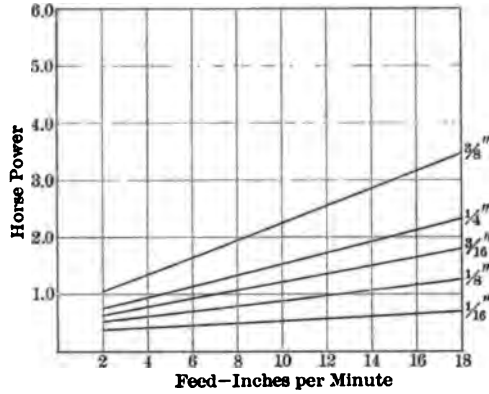
FIG. 34 TESTS OF HIGH-POWER FACE MILLING CUTTER 8 IN. DIAMETER, 14 IN. TEETH. CUTTING CAST IRON, CORRECTED FOR HARDNESS. WIDTH OF CUT 2 IN. REDUCED TO BASIS OF 1 IN.
