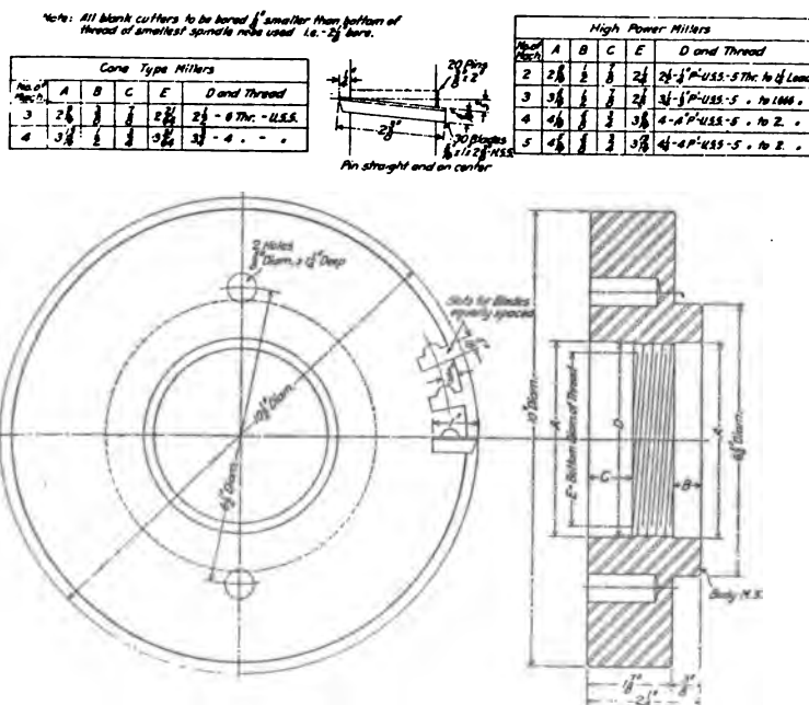
FIG. 17 FACE MILL OF OLDER TYPE
