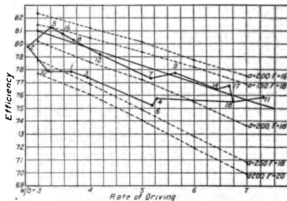
FIG. 24 EFFICIENCY CORRESPONDING TO DIFFERENT VALUES OF f AND a
