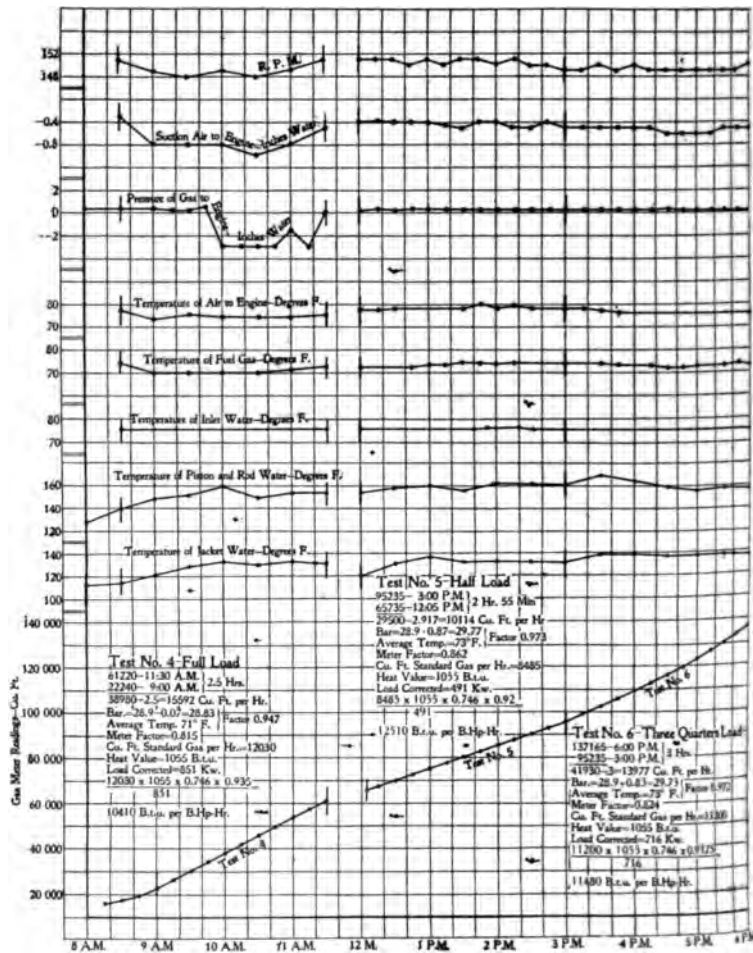
FIG. 11 SPECIMEN TEST LOG AND COMPUTATIONS
