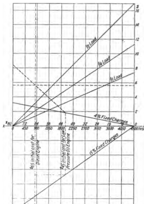
FIG. 37 COMPARISON BETWEEN DIESEL ENGINE AND LOW-PRESSURE OIL ENGINE
