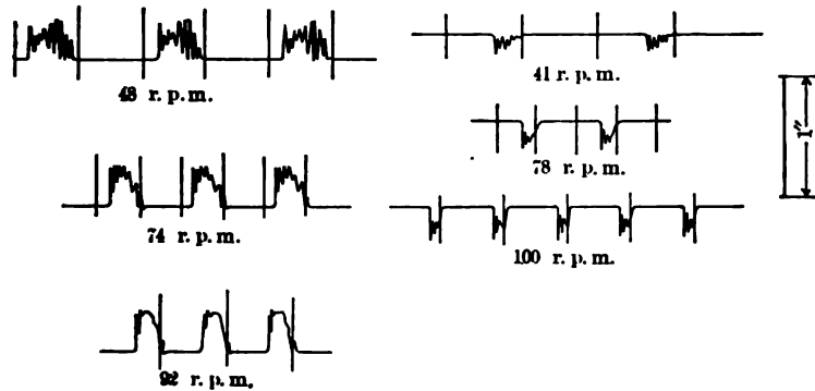
FIG. 26 VALVE MOTION DIAGRAMS TAKEN FROM INLET VALVE SHOWN IN FIG. 25
