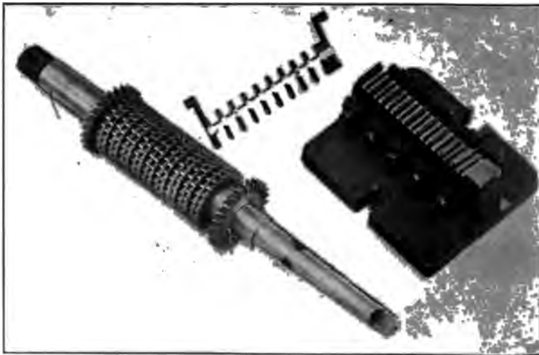
FIG. 22 MILLING FIXTURES AND GANG CUTTERS FOR A 48 AND 48 A
