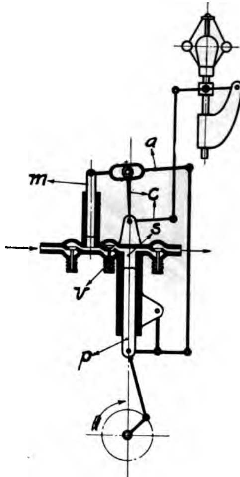
FIG. 31 DIAGRAMMATIC VIEW OF OIL PUMP OF ATLAS DIESEL ENGINE
