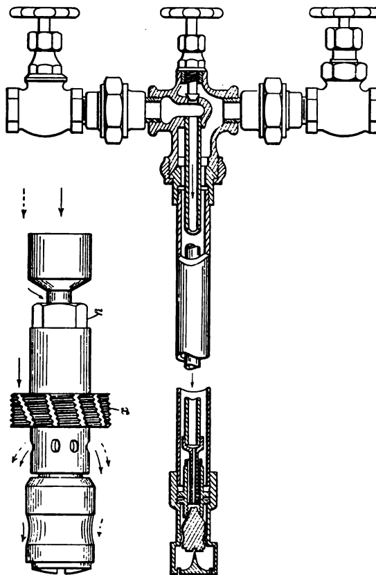
FIG. 10 IMPROVED LITTLE GIANT OIL BURNER
