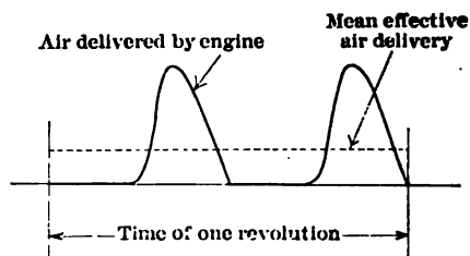
FIG. 28 AIR-WAVE PULSES CAUSED BY RECIPROCATING BLOWERS
