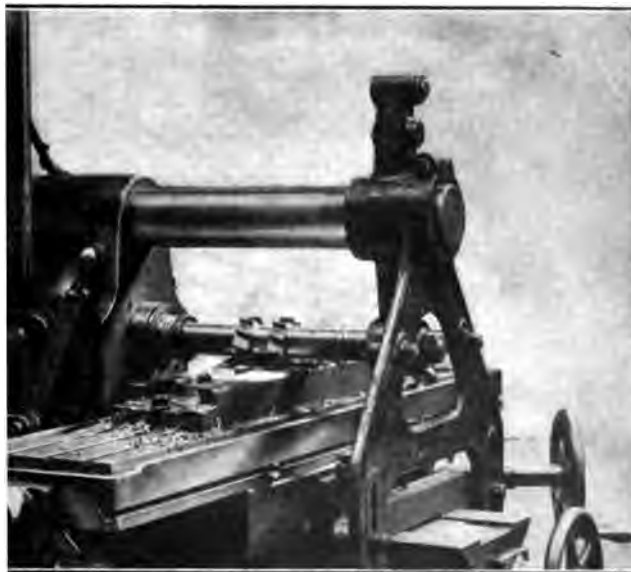
FIG. 27 NEW STYLE GANG AT WORK ON STEEL
