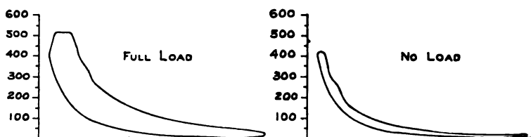
FIG 22 INDICATOR CARDS, TRINKLER-KÖRTING ENGINE
