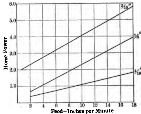
FIG. 36 TESTS OF REGULAR FACE MILLING CUTTER 9\frac{1}{2} IN. DIAMETER, 12 TEETH. CUTTING MACHINE STEEL; 0.50 MANGANESE, 0.20 CARBON, 55,000 LB. TENSILE STRENGTH. WIDTH OF CUT 6 IN., REDUCED TO BASIS OF 1 IN.
