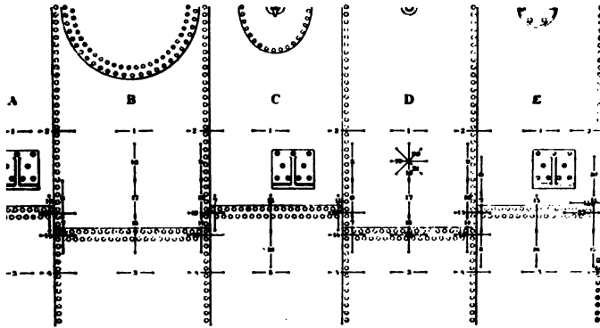
DIAGRAM SHOWING LOCATION OF GAGED LENGTHS, 10 IN. EACH, LAID OFF ON RIGHT SIDE ON BOILER No. 4092
