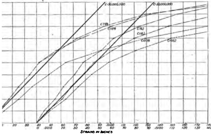
22 CURVES OF TANGENTIAL EXTENSION, ACROSS LONGITUDINAL SEAMS, OF LENGTH OF COURSE C , AND AT EDGES, RIGHT AND LEFT SIDES ER
