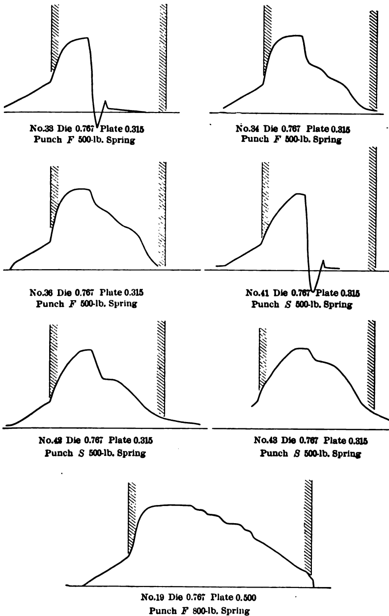
FIG. 6 SPECIMEN DIAGRAMS FROM RECORDER
