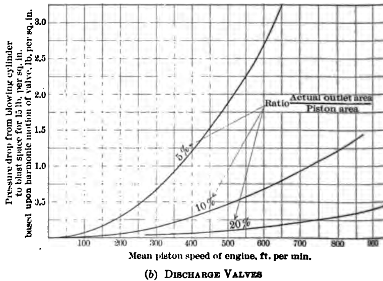
FIG. 5 PRESSURE LOSS IN BLOWING-ENGINE VALVES DUE TO VELOCITY HEAD
