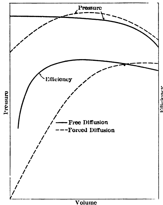
FIG. 7 COMPARISON OF BLOWERS WITH FREE AND FORCED DIFFUSION
