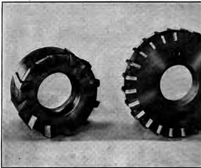
FIG. 18 COMPARISON OF HIGH POWER AND REGULAR FACE
