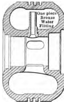
FIG. 4 SECTION OF GAS-ENGINE PISTON; RINGS 1 IN. BY 1 \frac{1}{4} IN.
