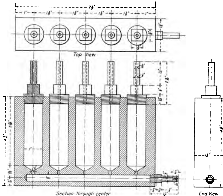
FIG. 6 AUTOMATIC AVERAGING MANOMETER
