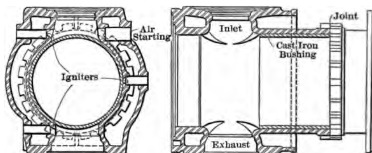
FIG. 1 CROSS-SECTION AND LONGITUDINAL SECTION OF CYLINDER
