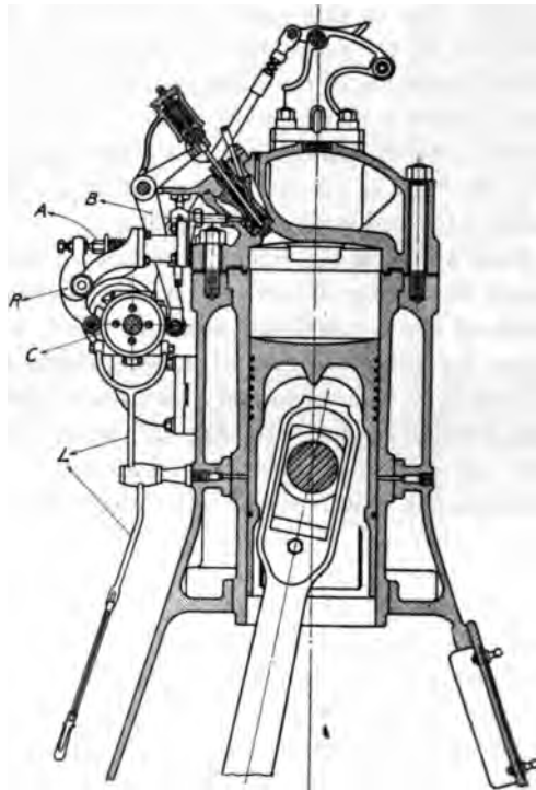
FIG. 29 CROSS-SECTION OF ATLAS DIESEL ENGINE
