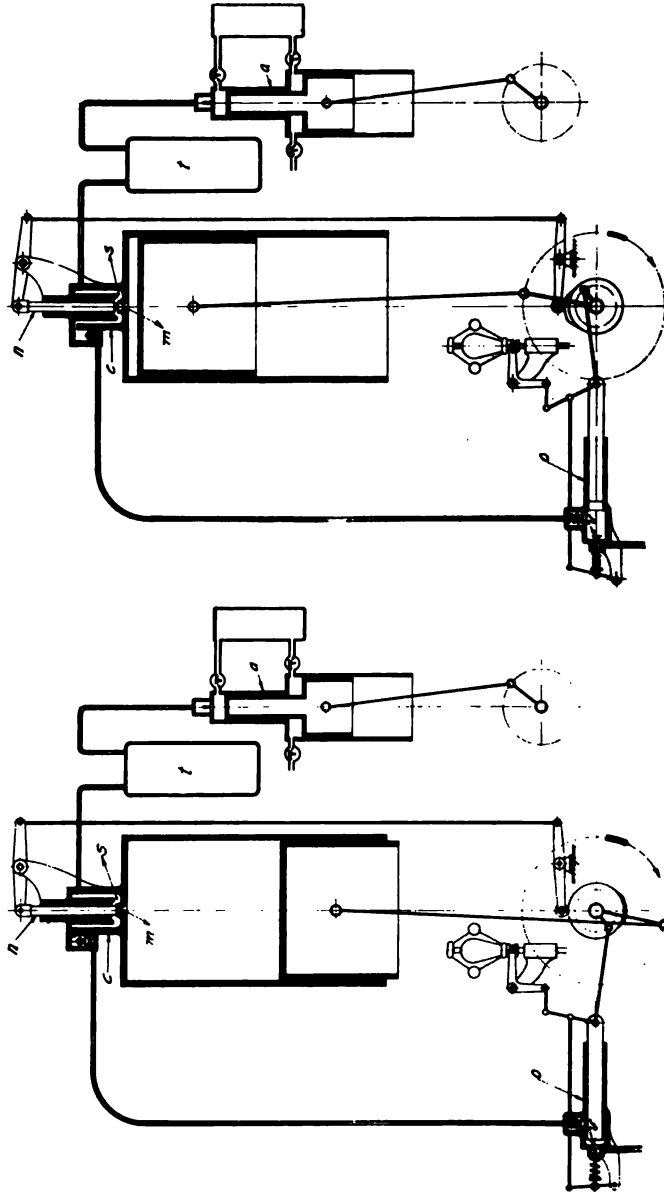
FIG. 4 DIESEL ENGINE WITH "CLOSED" INJECTION NOZZLE
