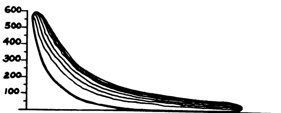
FIG. 32 DIAGRAMS OBTAINED ON OTHER DIESEL ENGINE WITH LOAD SUDDENLY THROWN OFF
