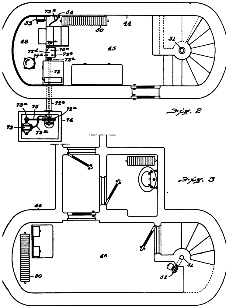
2 FLOOR PLAN OF THE UPPER COMPARTMENT OF OBSERVING ROOM AND THE BOX OUTSIDE THE BUILDING IN WHICH THE MOTOR IS LOCATED FIG. 3 FLOOR PLAN OF LOWER COMPARTMENT AND SUBWAY ENTRANCE
