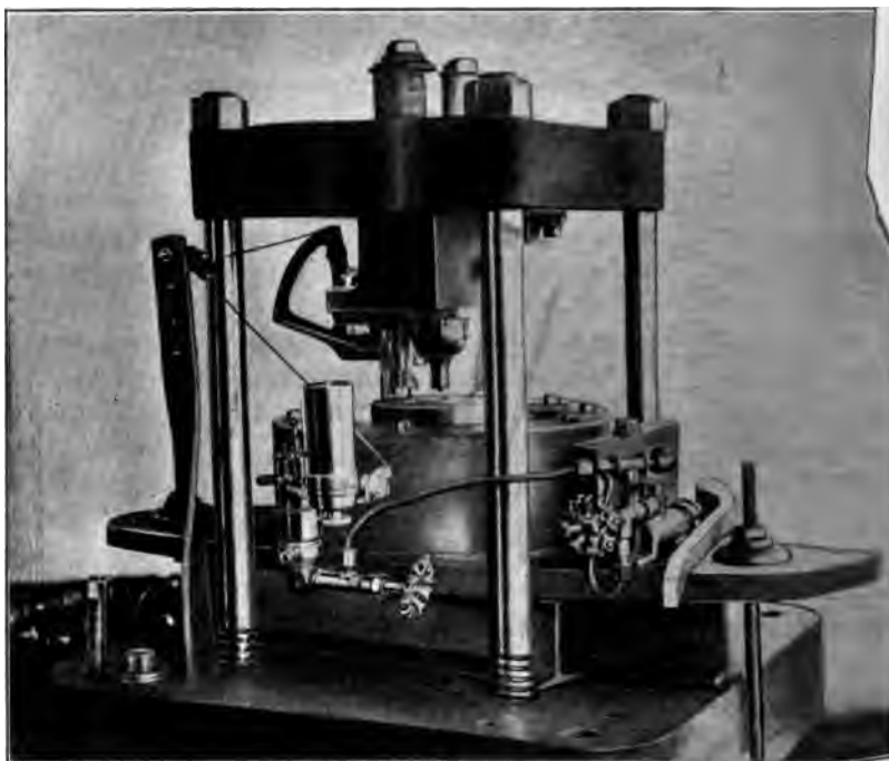
FIG. 1 PRESSURE-RECORDING APPARATUS APPLIED TO TESTING MACHINERY
