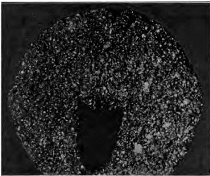
MICROPHOTOGRAPH OF SELF-PASTING CORE WHICH HAS BEEN VENTED WITH A PRESS VENT
