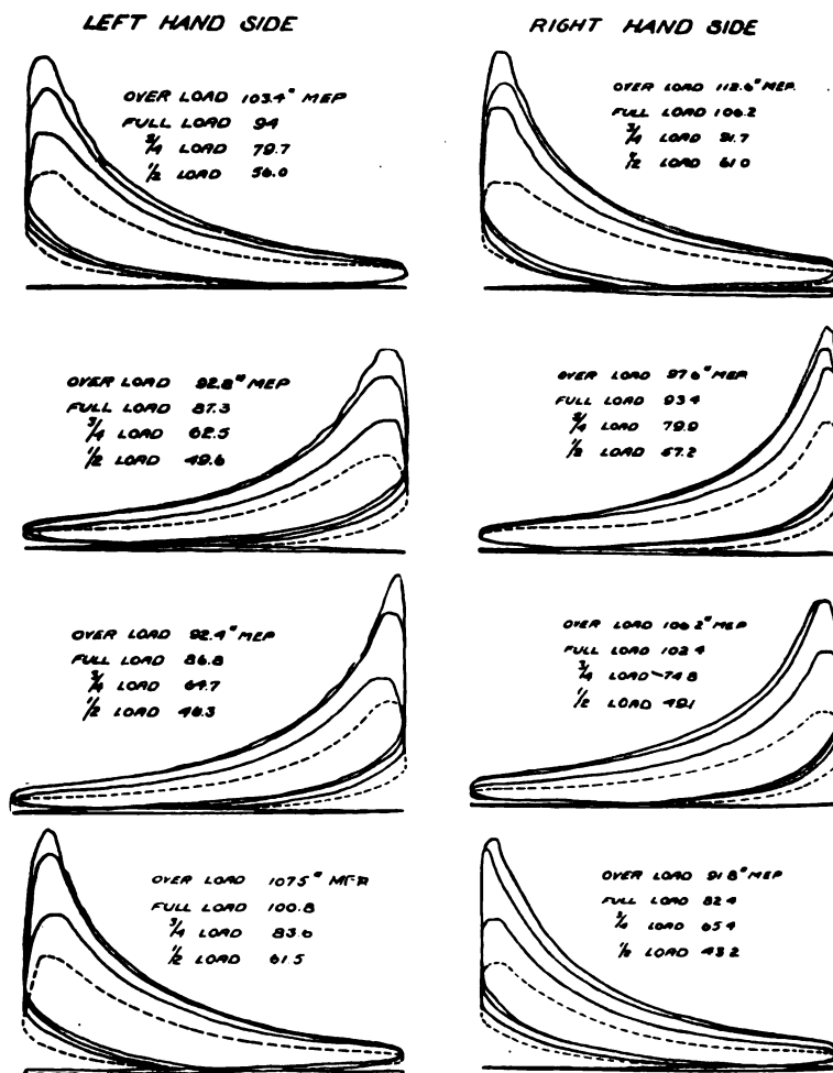
FIG. 8. TYPICAL CARDS TAKEN DURING TEST
