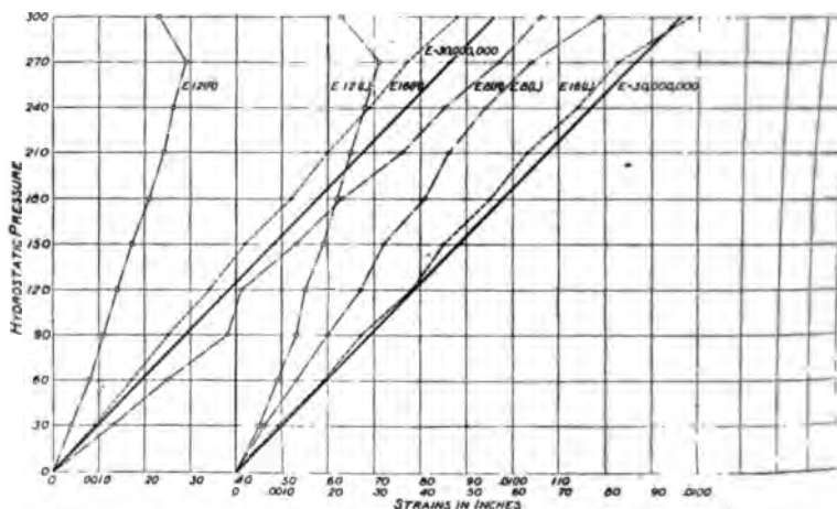
FIG. 20 CURVES OF TANGENTIAL EXTENSION, SOLID SHEETS, END COURSE E , NEAR REAR HEAD, GIRTH SEAM, AND MIDDLE OF LENGTH OF COURSE
