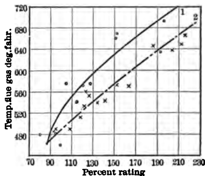
FIG. 15 PER CENT RATING AND FLUE GAS TEMPERATURE Curve 1 indicates Roney Stoker, Curve 2 Taylor Stoker
