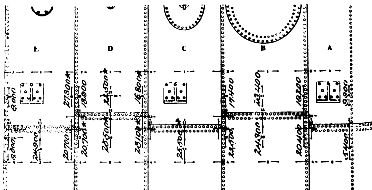
FIG. 43 TANGENTIAL STRESSES, LB. PER SQ. IN., AT 270 LB. BOILER PRESSURE. RESULTS BASED ON RESILIENCES. LEFT SIDE OF BOILER. NORMAL COMPUTED STRESS, 25,920 LB. PER SQ. IN. GAGED LENGTHS ON WHICH DECIDED PERMANENT SETS OCCURRED, INDICATED BY A STAR
