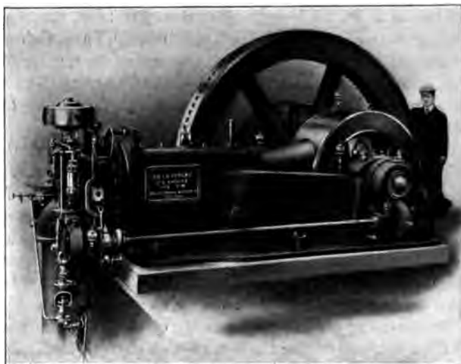
FIG. 38 EXTERIOR VIEW OF 85-H.P. DE LA VERGNE OIL ENGINE, TYPE FH
