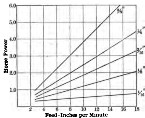
FIG. 38 TESTS OF HELICAL MILLING CUTTER 3\frac{1}{8} IN. DIAMETER, 4\frac{1}{2} IN. LEAD, 10 IN. PITCH. CUTTING MACHINE STEEL: 0.50 MANGANESE, 0.20 CARBON, 100 LB. TENSILE STRENGTH. WIDTH OF CUT 5\frac{1}{2} IN., REDUCED TO BASIS OF 1 IN.
