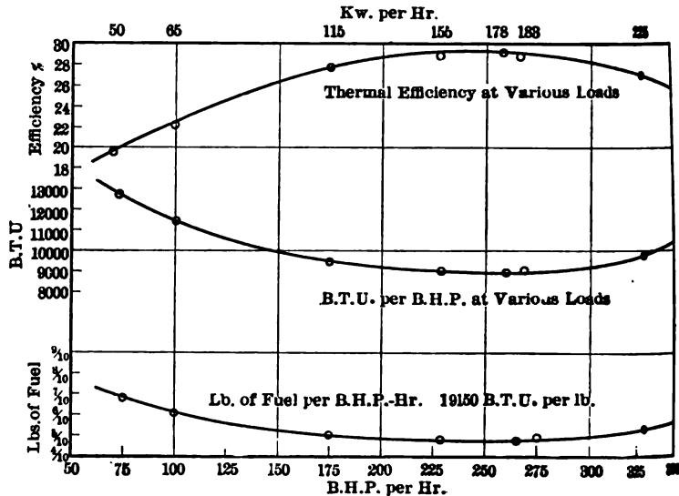
FIG. 43 EFFICIENCY AND FUEL CONSUMPTION CURVES, ATLAS OIL ENGINE, 300 B.H.P.
