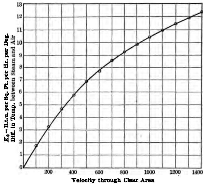
FIG. 36 RATE OF HEAT TRANSMISSION FOR VARIOUS VELOCITIES, VALUES OF K_o FROM TEST CORRECTED TO ABSOLUTE FILM TEMPERATURE OF 625 DEG.
