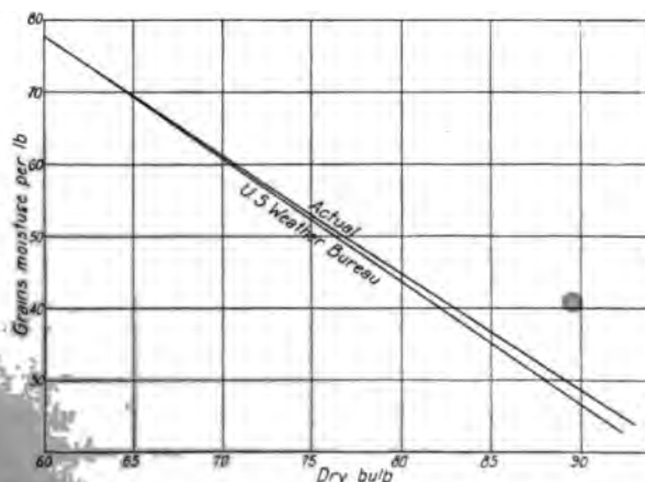
FIG. 5 COMPARISON OF ACTUAL MOISTURE CONTENT OF AIR AT 60 DEG. WET BULB WITH THAT GIVEN IN U. S. WEATHER BUREAU TABLES
