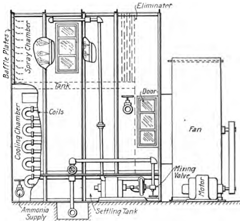
FIG. 8 SECTIONAL VIEW OF DEHUMIDIFIER
