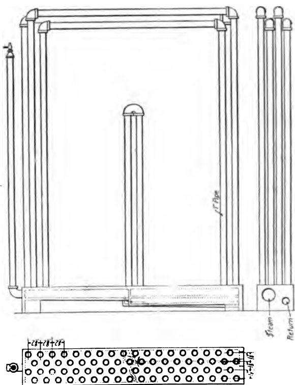
FIG. 30. DETAIL OF HEATER CONSTRUCTION
