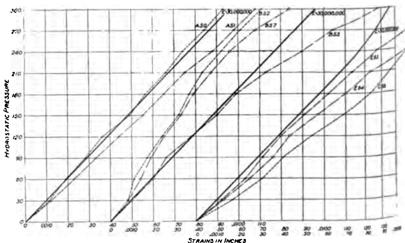
FIG. 21 CURVES OF TANGENTIAL EXTENSION, TOP OF BOILER, NEAR FRONT HEAD, GIRTH SEAMS, DOME AND MANHOLE PATCHES, AND SAFETY-VALVE NOZZLE
