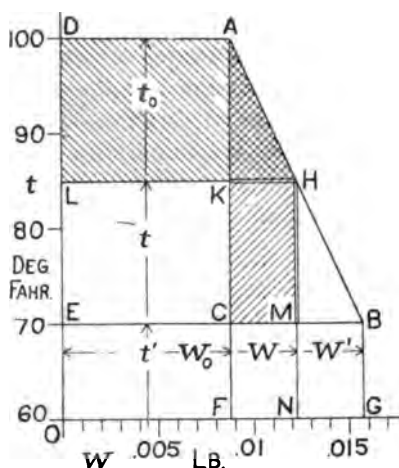
FIG. 14 HEAT OF SUPERHEATED STEAM DIAGRAM
