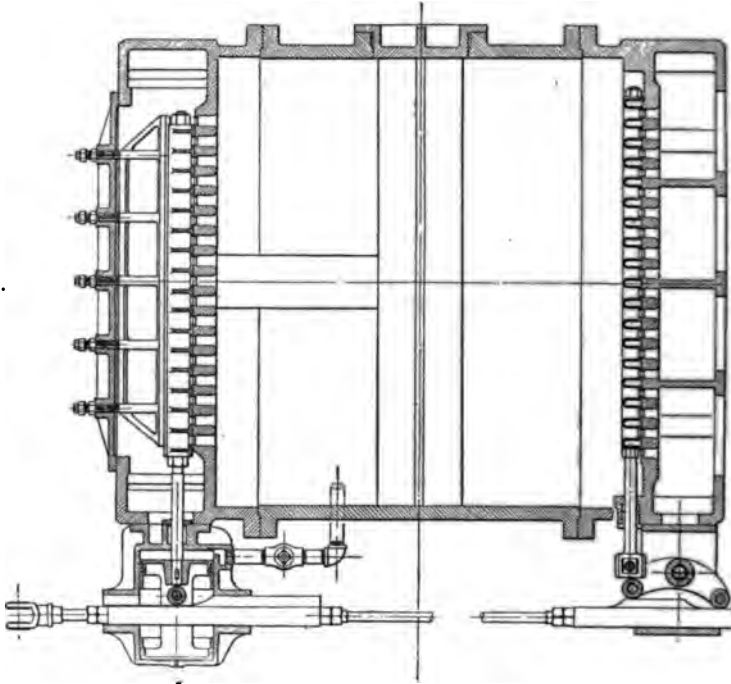
FIG. 13a SECTION THROUGH THE SOUTHWARK VALVE GEAR
