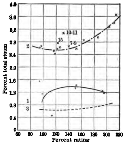
FIG. 17 PER CENT TOTAL STEAM USED AND PER CENT OF RATING
