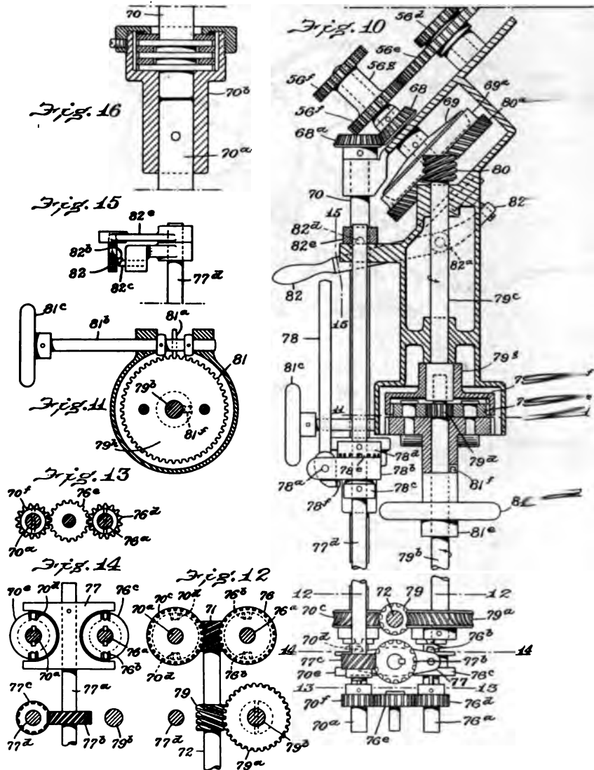
FIG. 10 DIAGRAM SHOWING TRANSMISSION GEARING AND CLUTCHES THAT GIVE THE MOTIONS TO THE TURRET. IT EXTENDS FROM THE TOP TO THE BOTTOM OF THE PAGE
