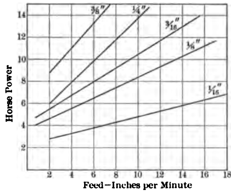
7 TESTS OF SPIRAL NICKED MILLING CUTTER 3 \frac{1}{2} IN. IN DIAMETER; TEETH AND ABOUT \frac{1}{8} IN. PITCH. CUTTING CAST IRON, CORRECTED FOR HARD- WIDTH OF CUT 6 IN.
