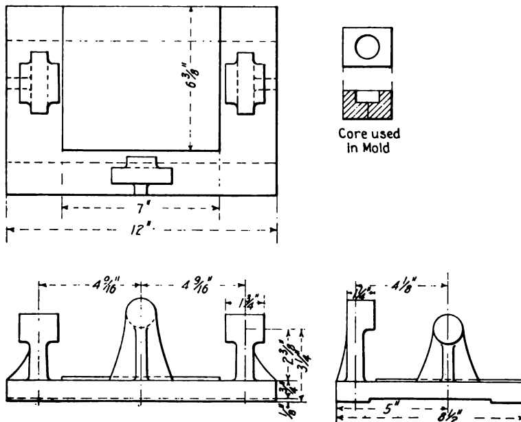
FIG. 45 MACHINE SHOP JIG
