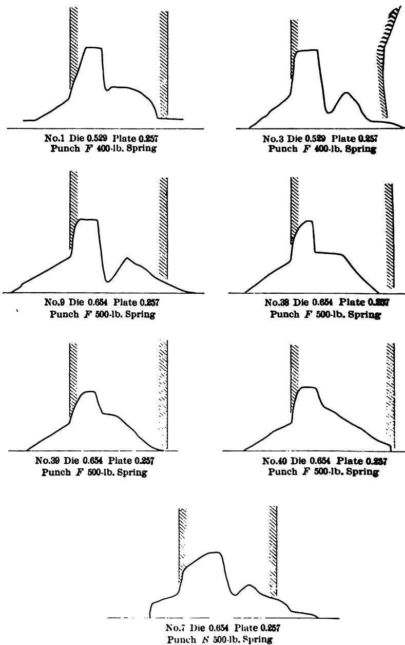
FIG. 5 SPECIMEN DIAGRAMS FROM RECORDER
