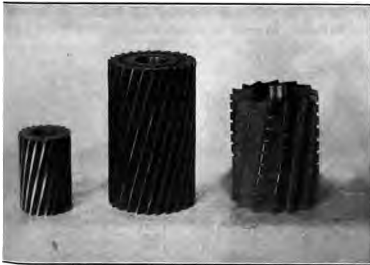
FIG. 4 COMPARISON OF OLD AND NEW STYLE SPIRAL MILLS
