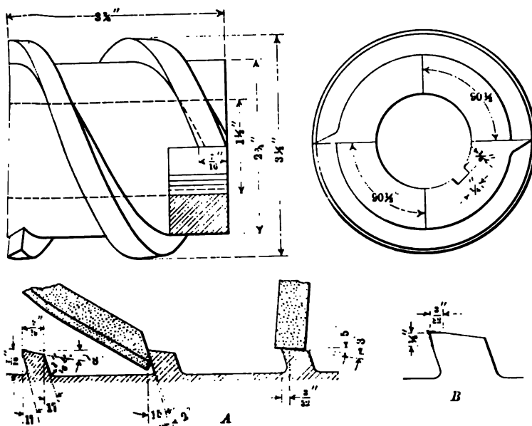
FIG. 19 DETAILS OF NEW TYPE OF HELICAL CUTTER
