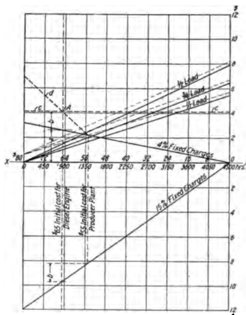
FIG. 33 COMPARISON BETWEEN THE DIESEL ENGINE AND GAS PRODUCER PLANT
