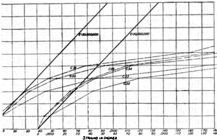
27 CURVES OF TANGENTIAL EXTENSION, HAND-RIVETED SECTION, COURSE C, TOP OF BOILER
