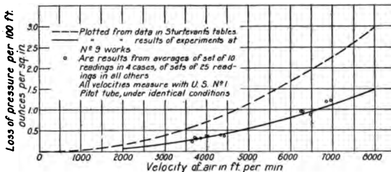
FIG. 11 CURVES OF LOSS OF PRESSURE DUE TO FRICTION IN 24-IN. PIPE
