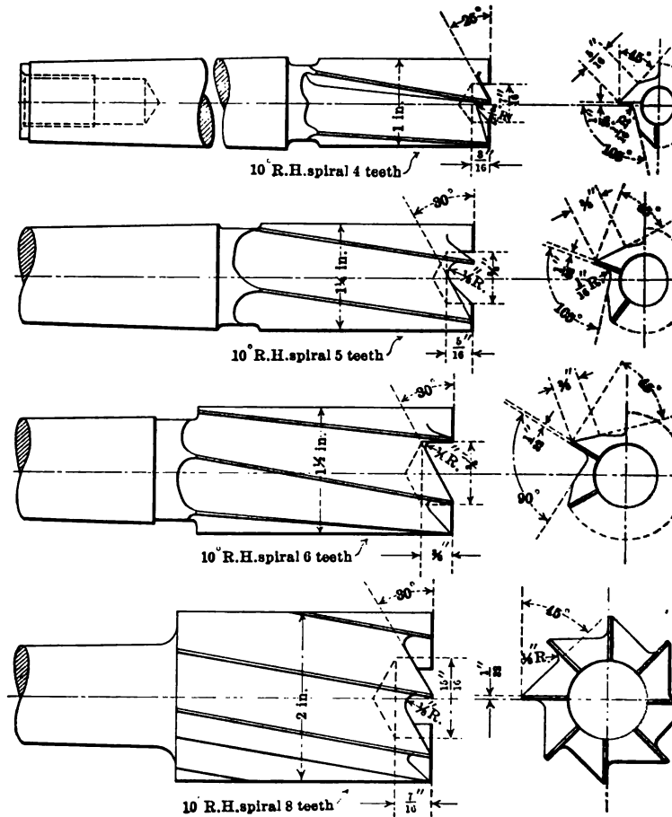
FIG. 11 NEW TYPE OF TAPER SHANK END MILLS
