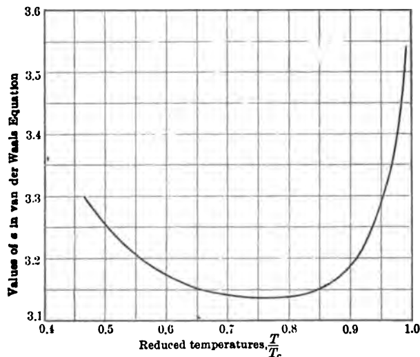
FIG. 4 CURVE SHOWING VARIATION OF g IN VAN DER WAALS' EQUATION FOR SATURATED STEAM
