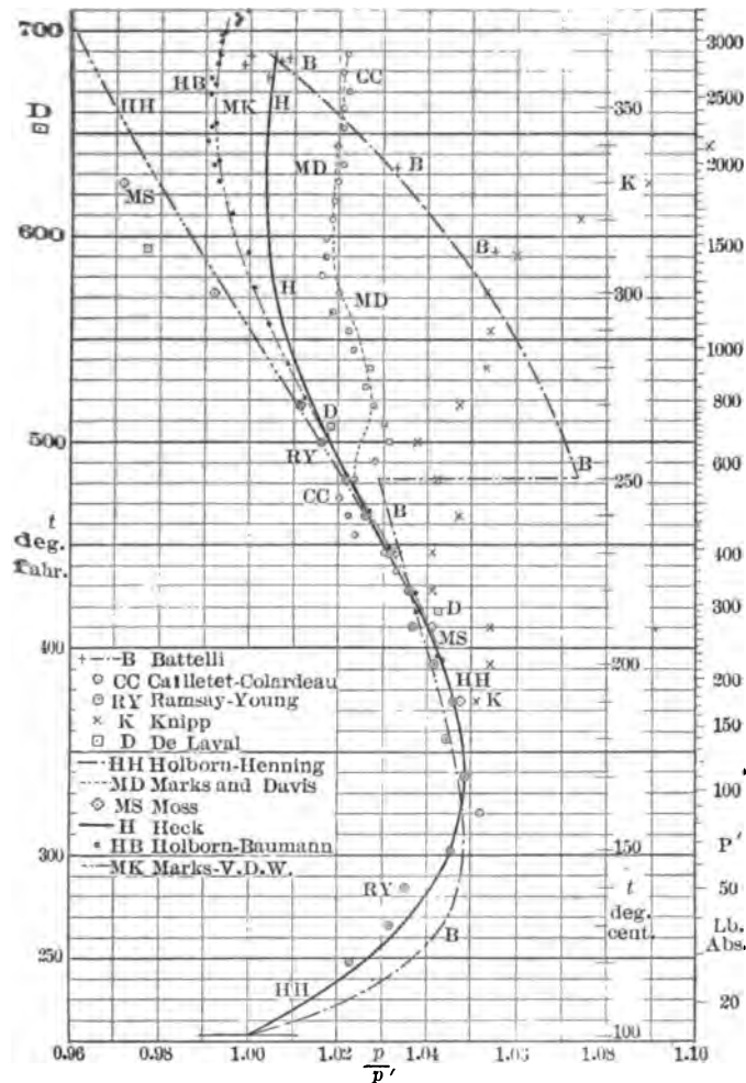
FIG. 6 COMPARISON OF DATA RELATING TO THE PRESSURE OF STEAM AT HIGH TEMPERATURES
