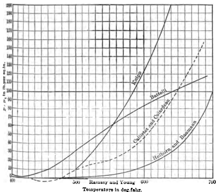
FIG. 1 CURVES SHOWING DEVIATION OF PRESSURE p OBSERVED BY VARIOUS INVESTIGATORS FROM PRESSURE p_t CALCULATED FROM MODIFIED THIESEN EQUATION FOR TEMPERATURE ABOVE 400 DEG. FAHR.
