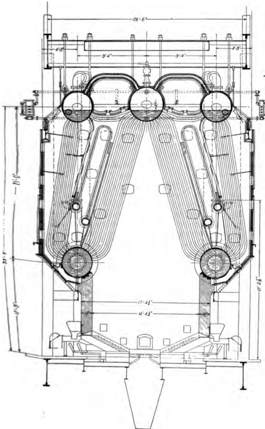
FIG. 3 LONGITUDINAL SECTION OF BOILER FITTED WITH TAYLOR STOKER
