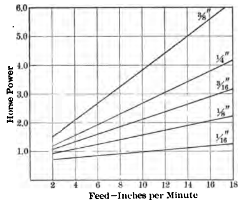
31 TESTS OF END MILLING CUTTER 3 IN. DIAMETER, 14 TEETH. CUT- FAST IRON, CORRECTED FOR HARDNESS. WIDTH OF CUT 2 1/4 IN. REDUCED TO OF 1 IN.
