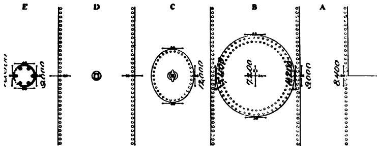
FIG. 44 TANGENTIAL STRESSES, LB. PER SQ. IN., AT 90 LB. BOILER PRESSURE. RESULTS BASED ON RESILIENCES. TOP OF BOILER. NORMAL COMPRESSION STRESS, 8,640 LB. PER SQ. IN.
