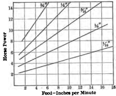
FIG. 6 TESTS OF SPIRAL NICKED MILLING CUTTER 3 \frac{3}{4} IN. IN DIAMETER; TEETH AND ABOUT \frac{1}{8} IN. PITCH. CUTTING CAST IRON CORRECTED FOR HARD- 38. WIDTH OF CUT 6 IN.
