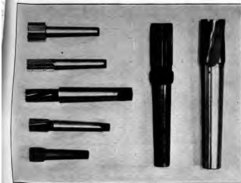
FIG. 12 COMPARISON OF OLD AND NEW STYLE END MILLS
