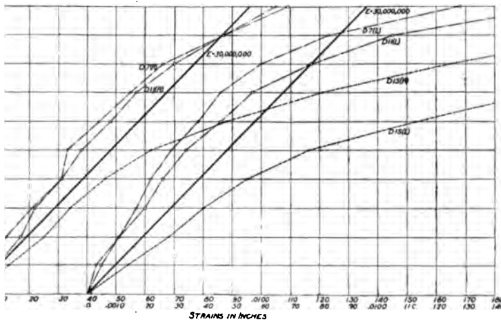
23 CURVES OF TANGENTIAL EXTENSION, ACROSS LONGITUDINAL SEAMS, OF LENGTH OF COURSE D , AND AT EDGES, RIGHT AND LEFT F BOILER
