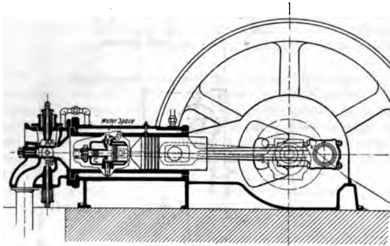
FIG. 39 LONGITUDINAL SECTION OF OIL ENGINE
