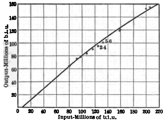
FIG. 13 INPUT AND OUTPUT RONEY STOKER Points 2-4 and 5-6 include banking
