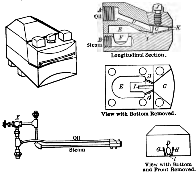
FIG. 8 HAMMEL OIL BURNER
