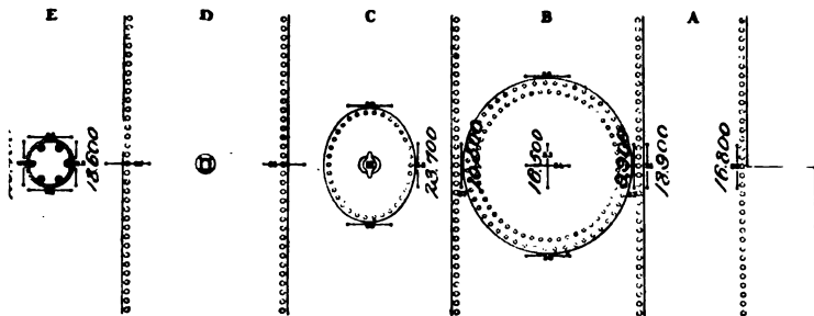
FIG. 45 TANGENTIAL STRESSES, LB. PER SQ. IN., AT 180 LB. BOILER PRESSURE. RESULTS BASED ON RESILIENCES. TOP OF BOILER. NORMAL COMPRESSION STRESS, 17,280 LB. PER SQ. IN.
