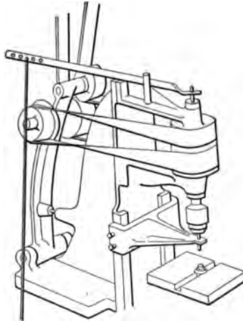
FIG. 2 VERTICAL POWER TAPPING MACHINE
