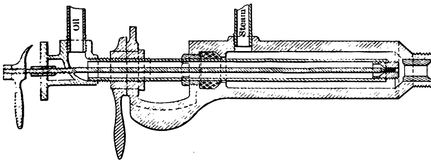
FIG. 9 KIRKWOOD OIL BURNER
