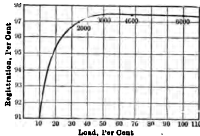
FIG. 9 CALIBRATION CURVE, WATT-HOUR METER
