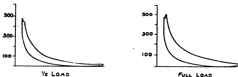
FIG. 12 INDICATOR CARDS, TYPE FH DE LA VERGNE ENGINE
