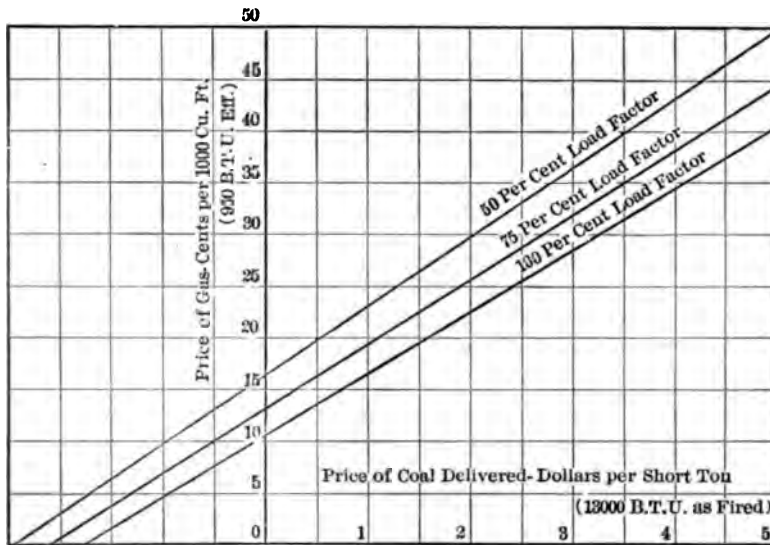
FIG. 14 EQUALIZATION CHART, COAL AND NATURAL GAS
