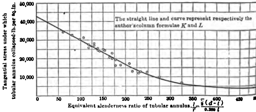
FIG. 6 PLOTTED RESULTS OF THE AUTHOR'S EXPERIMENTS ON COLLAPSING PRESSURES OF LAP-WELDED STEEL TUBES
