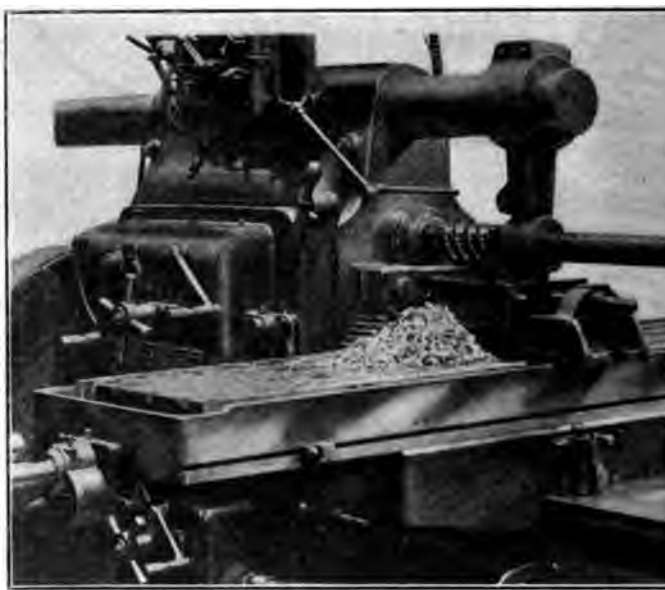
FIG. 21 HELICAL CUTTER AT WORK ON STEEL TEST PIECE
