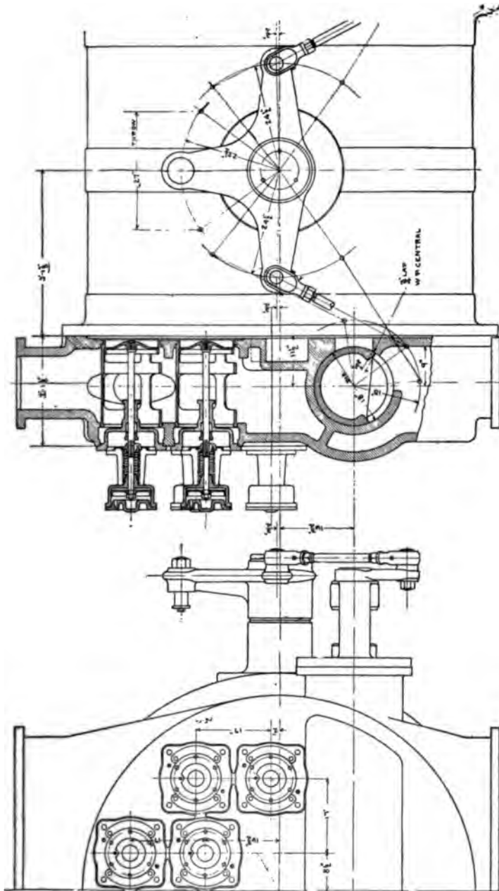
FIG 12 ORIGINAL MESTA VALVE GEAR
