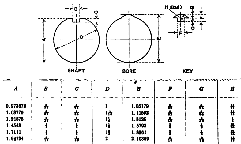
FIG. 5 SHAPE AND DIMENSIONS OF KEYS USED FOR MILLING-CUTTER ARBORS
