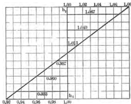
FIG. 3 DIAGRAM SHOWING INTERMEDIATE TEMPERATURES FOR A STEAM TURBINE
