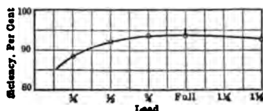
FIG. 4 PROBABLE GENERATOR EFFICIENCY CURVE
