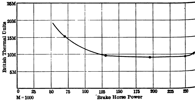
FIG. 44 CONSUMPTION B.H.P. CURVES
