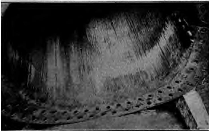
3 INTERIOR OF DOME SHOWING LINES ALONG WHICH SCALE WAS DISTURBED AFTER PRESSURE OF 266 LB. ON SHELL
