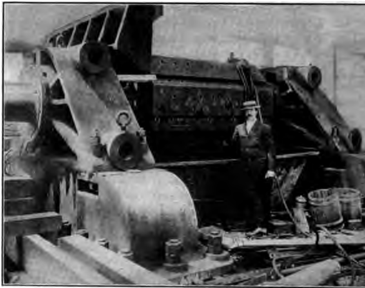
FIG. 11 GIANT ROLLS DURING ERECTION AT THE PLANT OF THE U. S. CRUSHED STONE COMPANY, CHICAGO
