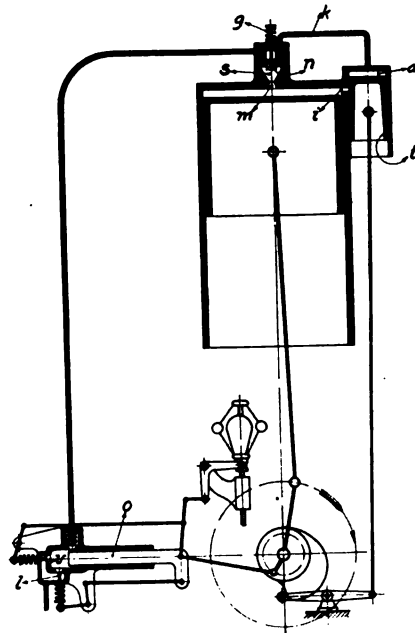
FIG. 27 SETZ OIL ENGINE WITH AUXILIARY INJECTION AIR PISTON
