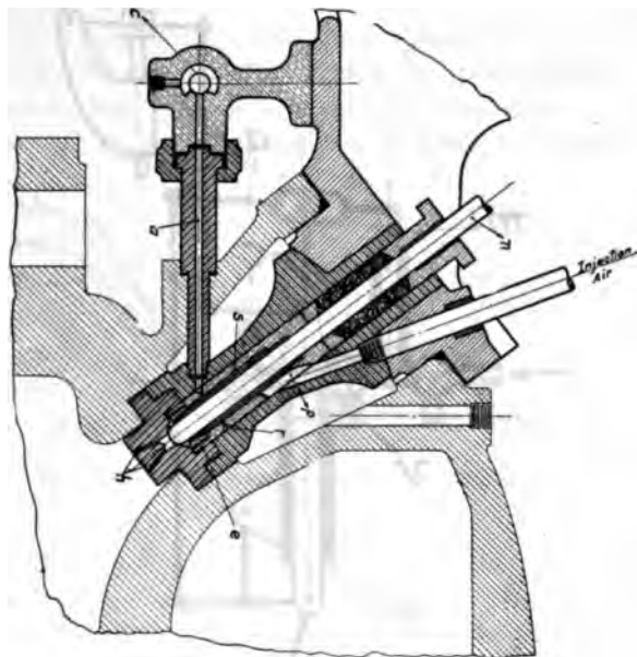
FIG. 30 INJECTION VALVE OF ATLAS DIESEL ENGINE
