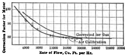
FIG. 10 GAS METER CALIBRATION CURVES
