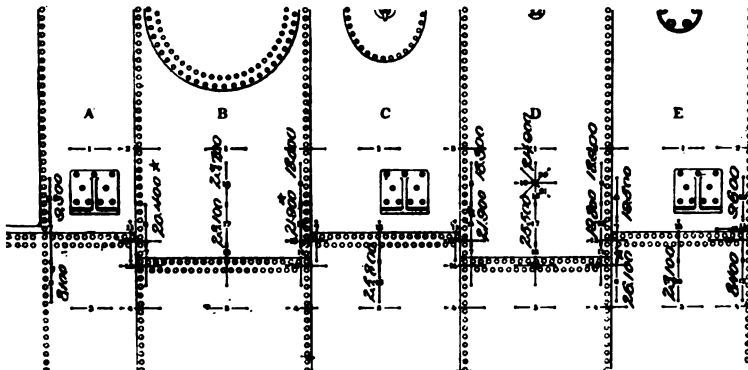
FIG. 40 TANGENTIAL STRESSES, LB. PER SQ. IN. AT 270 LB. BOILER PRESSURE. RESULTS BASED ON RESILIENCES. RIGHT SIDE OF BOILER. NORMAL PUT STRESS, 25,920 LB. PER SQ. IN. GAGED LENGTHS ON WHICH DECIDED MANENT SETS OCCURRED, INDICATED BY A STAR
