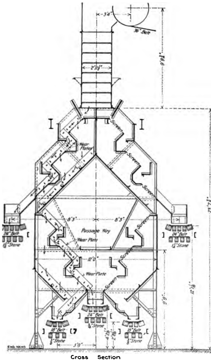
FIG. 12 SECTIONAL VIEW OF EDISON SIZING SCREEN
