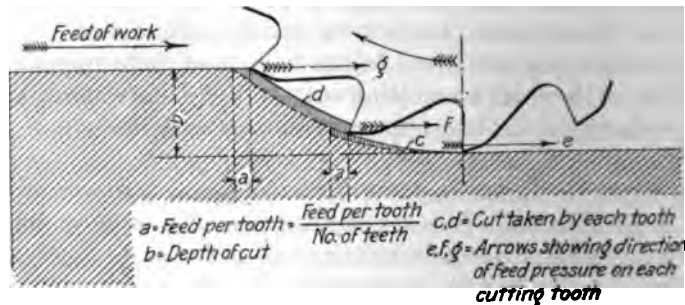
FIG. 44 ACTION OF A SIDE CUTTER
