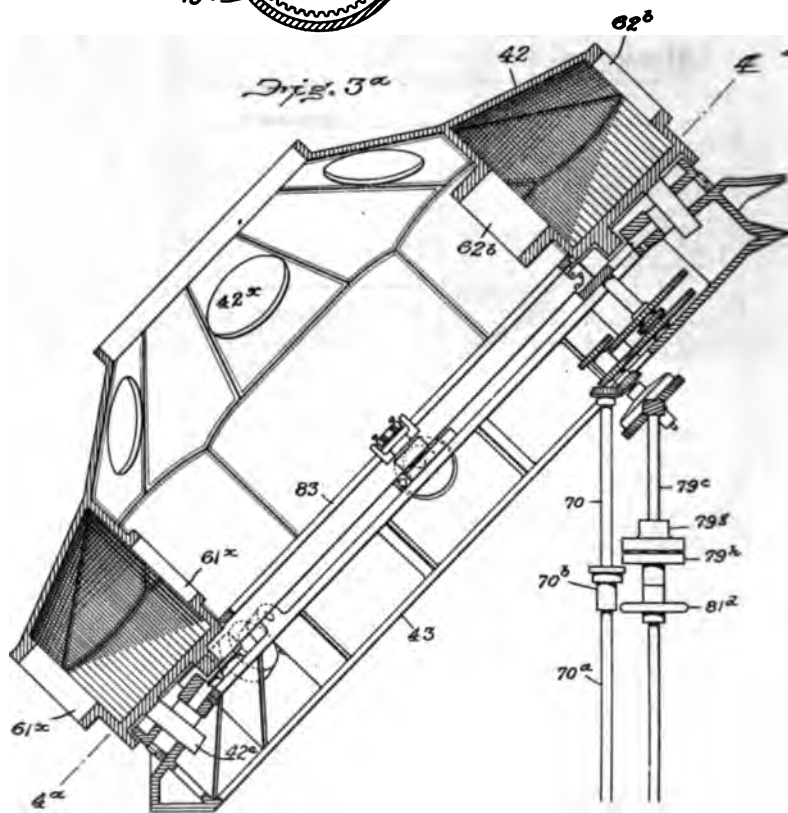
FIG. 3a LONGITUDINAL VERTICAL SECTION THROUGH THE TURRET FIG. 11a ORIGINAL FORM OF DIFFERENTIAL MOTION FOR MANUALLY VARYING THE ADVANCE OF DOME AS IT IS TURNED BY MOTOR TO FOLLOW A STAR This has been superseded by Fig. 11, but may be reinstated again.
