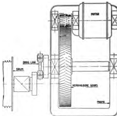
FIG. 14 ELECTRIFICATION OF MINE HOIST FORMERLY STEAM DRIVE.
