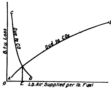
FIG. 18 RELATION BETWEEN AMOUNT OF AIR SUPPLY AND B.T.U. LOSS
