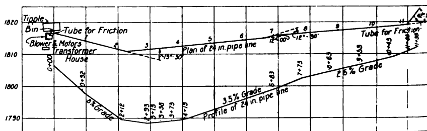
FIG. 1 PLAN AND PROFILE OF EXPERIMENTAL PIPE LINES
