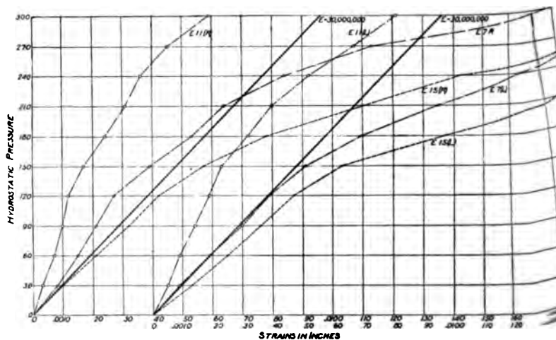
FIG. 25 CURVES OF TANGENTIAL EXTENSION, ACROSS LONGITUDINAL SEAM AND SOLID SHEETS, END COURSE E, EXTENSIONS NEAR REAR HEAD AND GIRTH SEAM MIDDLE OF LENGTH OF COURSE
