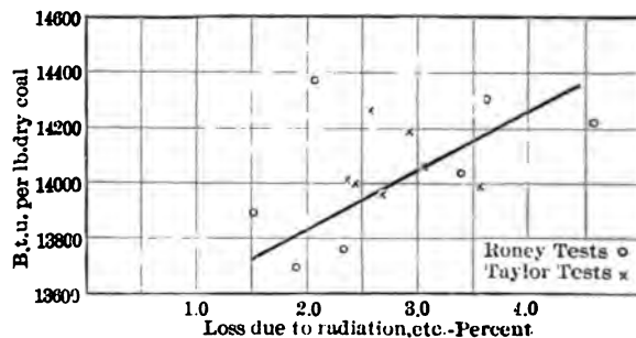
FIG. 21 RELATION OF RADIATION LOSS TO B.T.U. OF COAL
