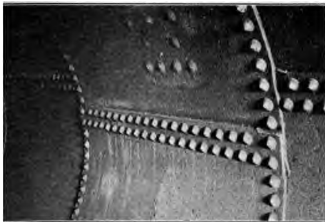
INTERIOR VIEW OF BOILER NO. 4084 AFTER 295 LB. PRESSURE SCALE DISTURBED IN VICINITY OF THE LONGITUDINAL SEAM AND PORTING LUG
