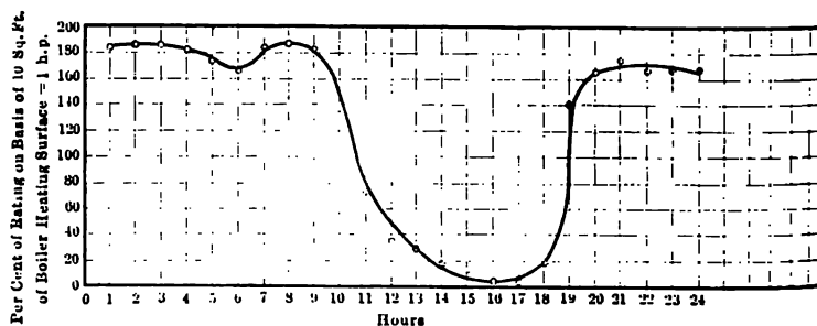
FIG. 6 CAPACITY OF BOILER WITH TAYLOR STOKER FOR EACH HOUR OF A TEST WHERE THE FIRES WERE BANKED FOR 7\frac{1}{2} HOURS
