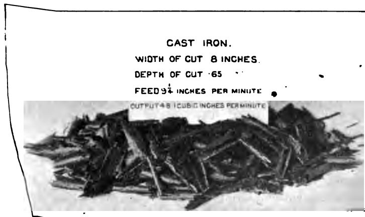
FIG. 47 EXAMPLE OF HEAVY MILLING PERFORMED BY NO. 22 SINGLE PULLEY PLAIN MILLING MACHINE
