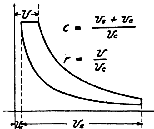
FIG. 35 IDEAL INDICATOR DIAGRAM OF DIESEL ENGINE
