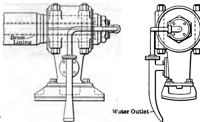
FIG. 7 VIEW SHOWING WATER CONNECTION TO TAIL ROD
