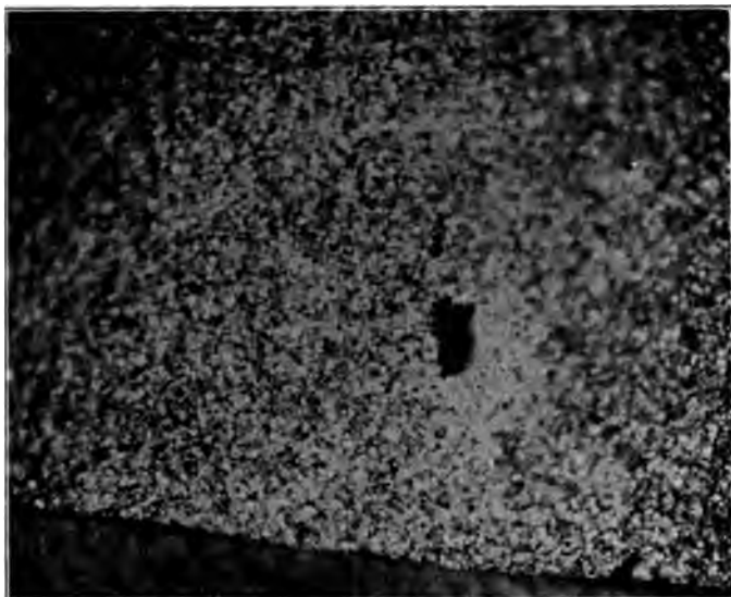
1 MICROPHOTOGRAPH OF CORE SHOWING HOLE WHERE UNBONDED SAND FLOWED OUT
