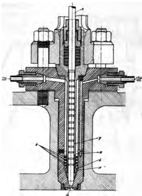
Fig. 6. TYPICAL ATOMIZER USED ON EUROPEAN DIESEL ENGINES
