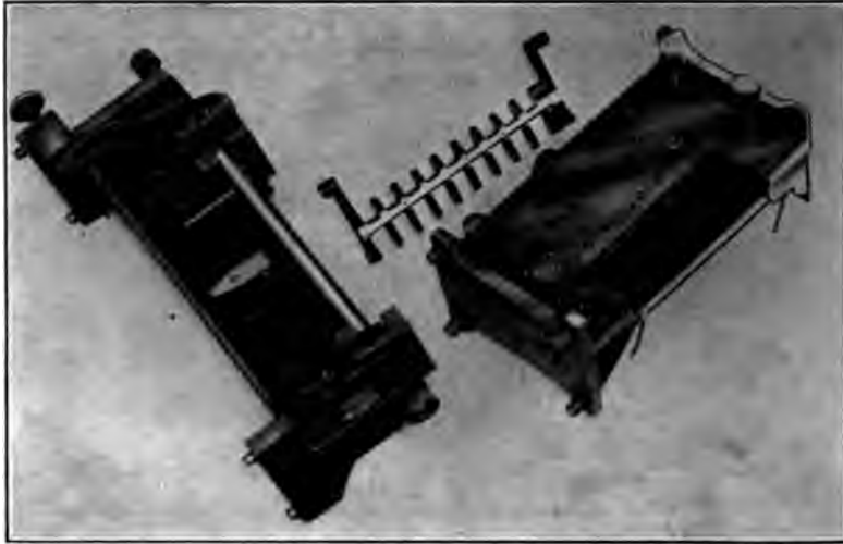
FIG. 21 ASSEMBLING DRILL JIG AND DRILL JIG FOR A 48 AND 48 A
