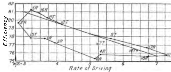
FIG. 22 RELATION OF EFFICIENCY TO RATE OF DRIVING
