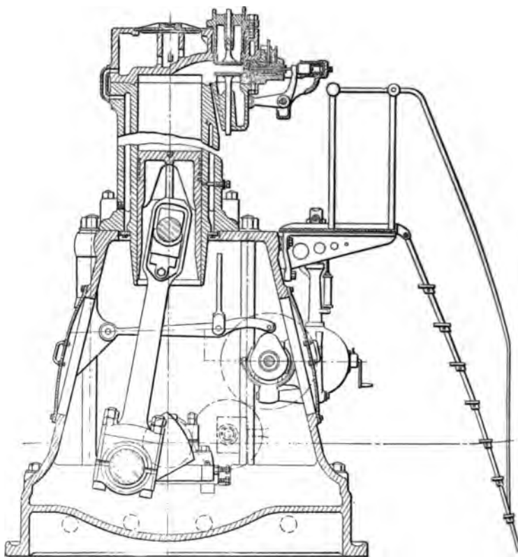
FIG. 7 CROSS-SECTION OF AMERICAN DIESEL ENGINE
