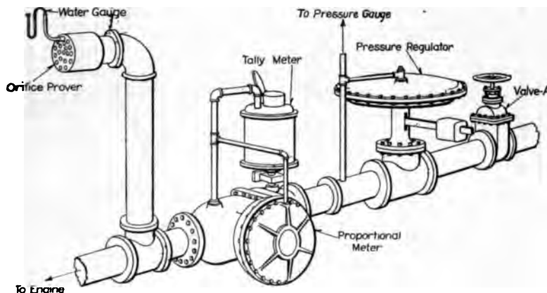
FIG. 5 DIAGRAM OF CONNECTIONS FOR PROVING METER BY STANDARD ORIFICES. PROVER REMOVED DURING PROGRESS OF TESTS AND CONNECTION SEALED BY BLANK FLANGE
