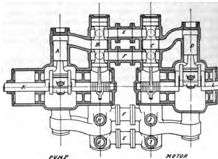
FIG. 2 SECTIONAL ELEVATION OF PUMP AND MOTOR
