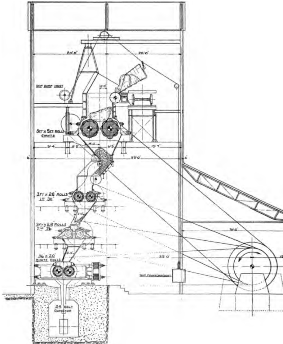
FIG. 3 SECTIONAL VIEW OF THE CRUSHING PLANT OF THE EDISON PORTLAND CEMENT COMPANY
