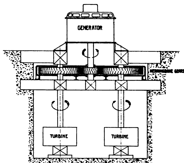
FIG. 9 DIAGRAM OF GEAR CONNECTION BETWEEN HYDRAULIC TURBINES AND AN ELECTRIC GENERATOR
