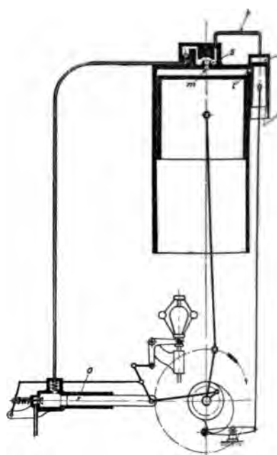
FIG. 19 OIL ENGINE WITH AUXILIARY INJECTION AIR PISTON
