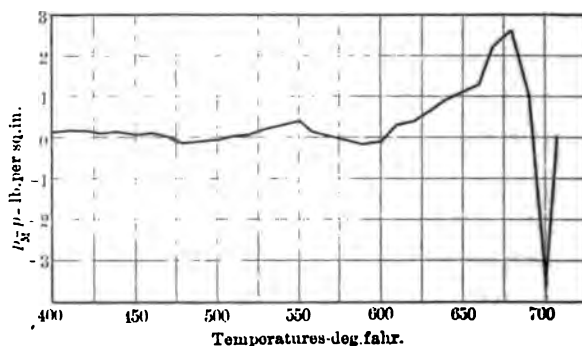
FIG. 5 CURVE SHOWING DIFFERENCE BETWEEN CALCULATED PRESSURE p_g AND OBSERVED PRESSURE p FOR TEMPERATURE RANGE FROM 400 DEG. FAHR. TO THE CRITICAL TEMPERATURE
