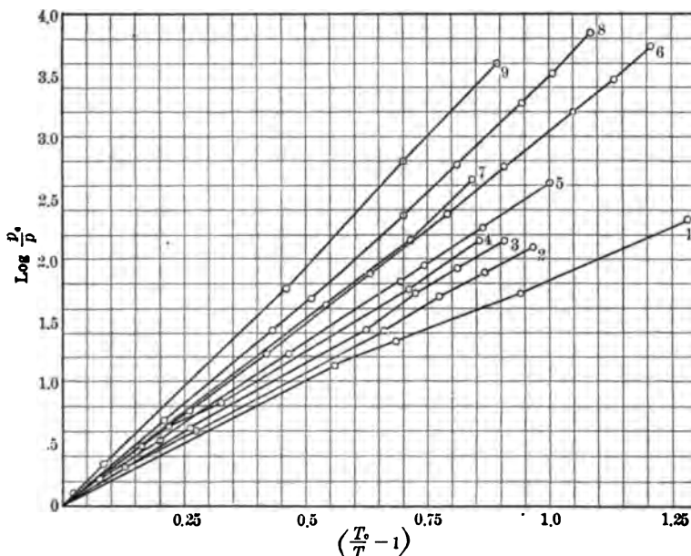
FIG. 3 CURVES SHOWING APPLICABILITY OF VAN DER WAALS EQUATION TO (1) HYDROGEN, (2) ARGON, (3) KRYPTON, (4) OXYGEN, (5) CARBON BI-SULPHIDE, (6) FLUORBENZOL, (7) ETHER, (8) PROPYLACETATE, (9) ETHYL ALCOHOL, TAKEN FROM NEERNST
