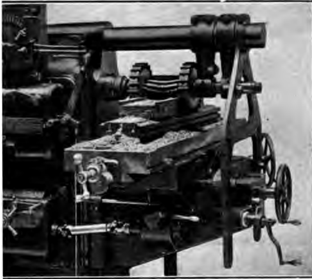
1. 26 WIDE-SPACE GANG ROUGHING VISE HOUSINGS
