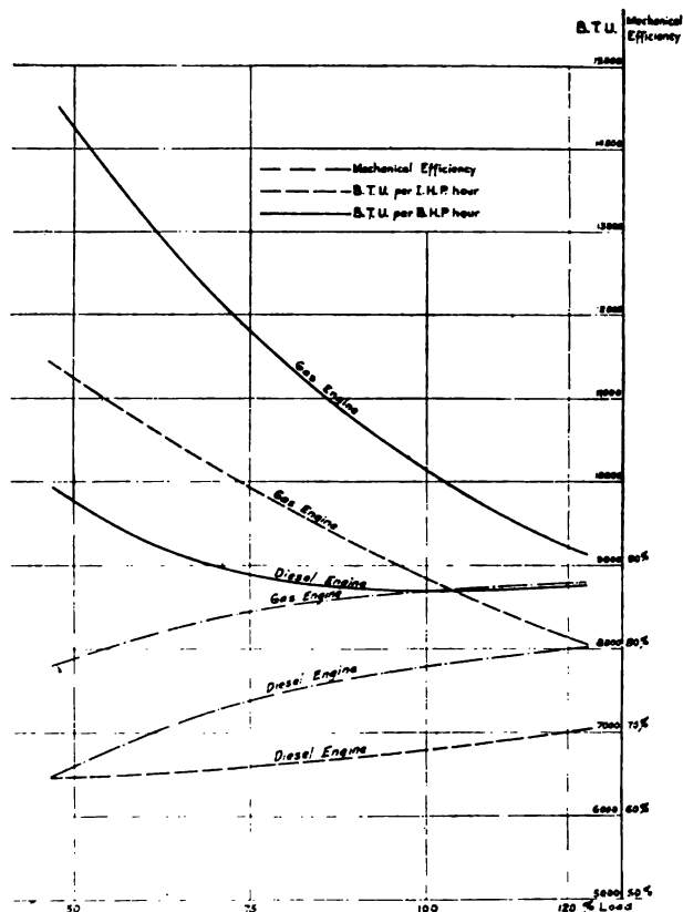
FIG. 34 MECHANICAL EFFICIENCIES AND B.T.U. CONSUMED IN GAS AND DIESEL ENGINES
