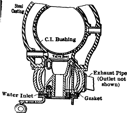
FIG. 2 CROSS-SECTION OF CYLINDER THROUGH IGNITER HOLES
