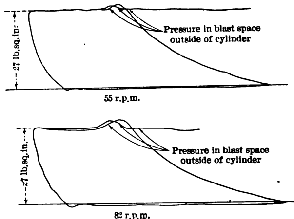
FIG. 23 INDICATOR CARD TAKEN FROM CYLINDER WITH VALVES SHOWN IN FIG. 20
