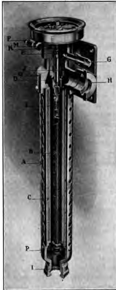
FIG. 13 METALLIC DIFFERENTIAL THERMOSTAT
