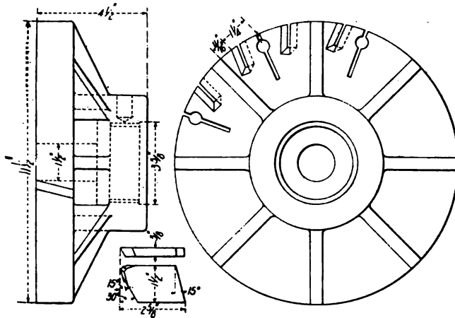
FIG. 49 EARLY INSERTED TOOTH FACE CUTTER, FEBRUARY 1903
