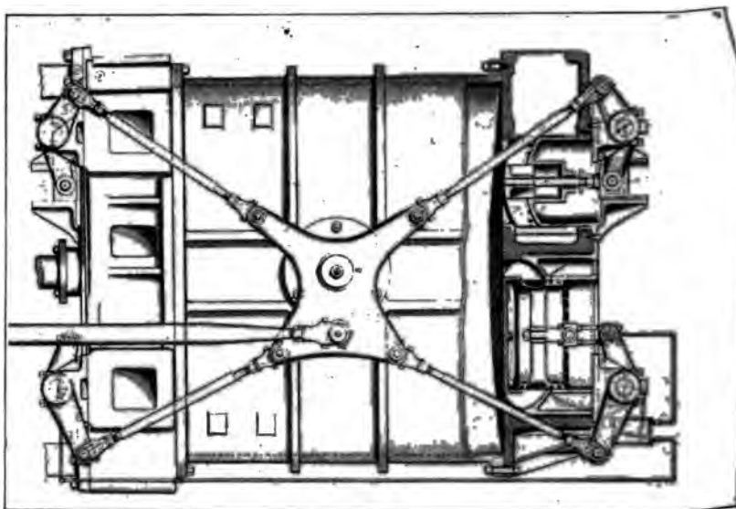
FIG. 7 VALVE GEAR BUILT BY WM. TOD COMPANY
