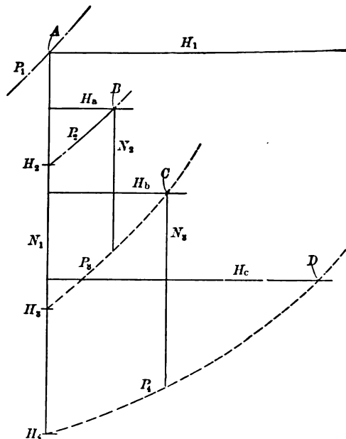
FIG. 2 SHOWING USE OF MOLLIER'S DIAGRAM
