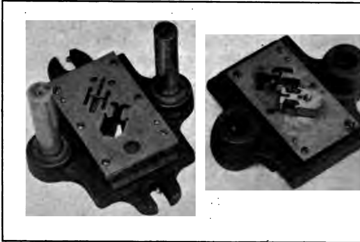
FIG. 9 TWO-STEP PROGRESSIVE BLANKING DIE FOR 50 I
