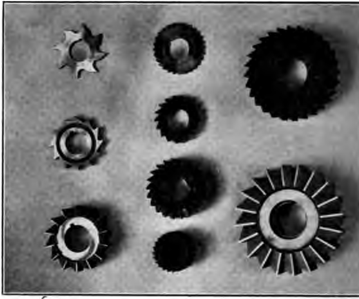
FIG. 15 COMPARISON OF SIDE MILLS AND SLOTTING MILLS
