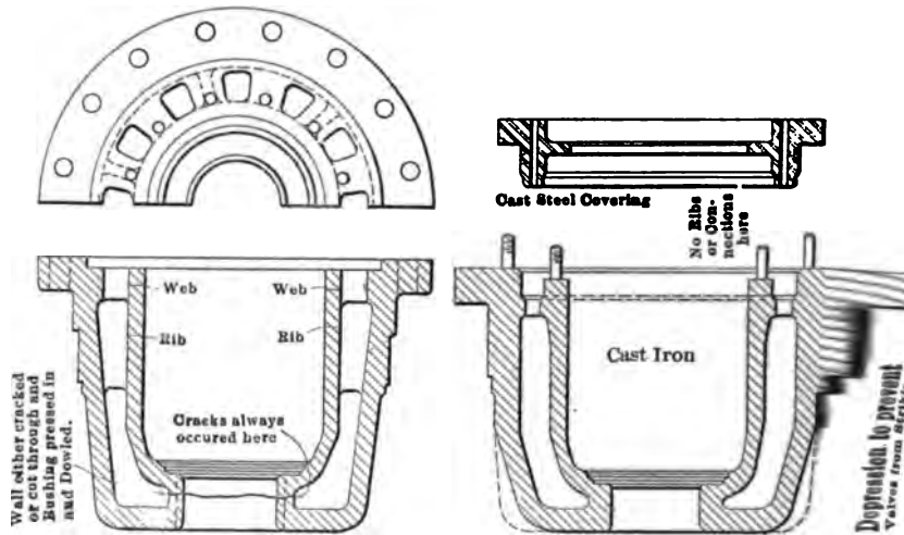
[FIG. 8 SECTION OF ORIGINAL CYLINDER HEAD
