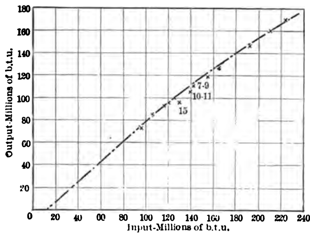
FIG. 14 INPUT AND OUTPUT TAYLOR STOKER Points 15, 10-11, 7-9 include banking
