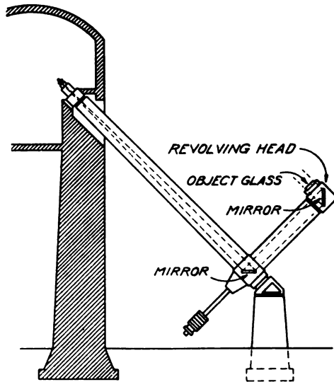
FIG. 1A DIAGRAMMATIC SKETCH OF THE LOEWY EQUATORIAL COUDÉ Object glass, 23 in. in diameter with 25:1 focal length; largest diameter of larger mirror at elbow, 23 in.
