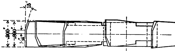
FIG. 43 CUTTER WITH OPPOSITE CORNERS OF ALTERNATE TEETH REMOVED
