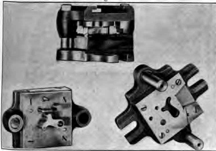
FIG. 8 TYPICAL BLANKING DIE
