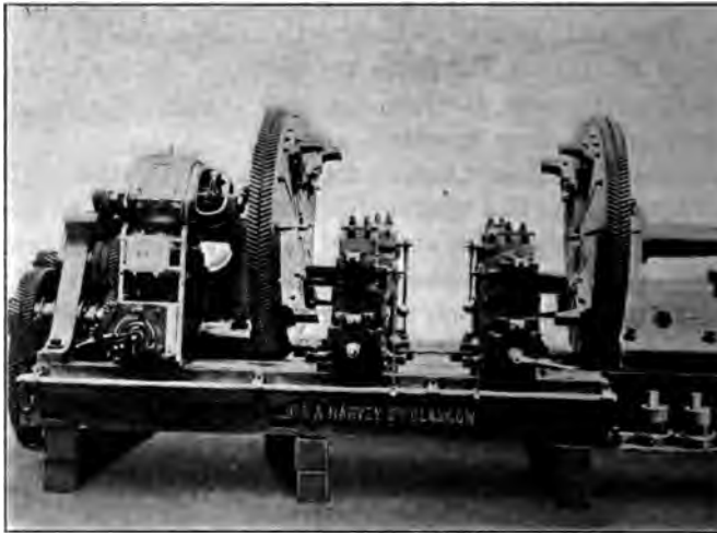
FIG. 10 TIRE-TURNING LATHE WITH HERRINGBONE G
