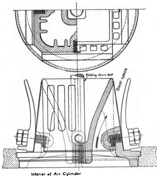
FIG. 15b SLICK AIR VALVE
