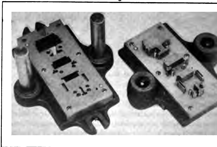
FIG. 10 THREE-STEP PROGRESSIVE BLANKING DIE FOR 51 I
