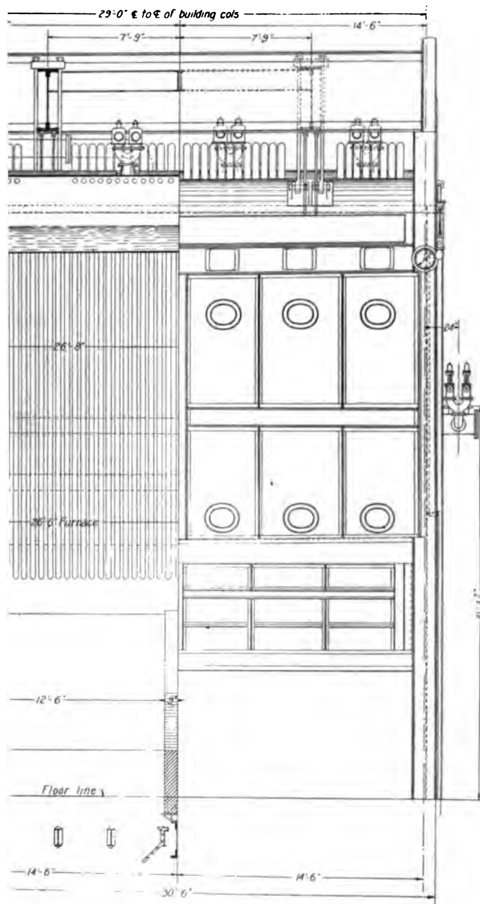
AND HALF-SECTION OF BOILER OF 2365 RATED HORSEPOWER, FITTED WITH RONEY STOKER
