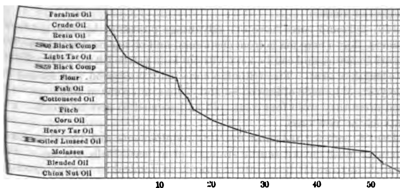
FIG. 26 DIAGRAM SHOWING RELATIVE STRENGTH OF A NUMBER OF BINDERS
