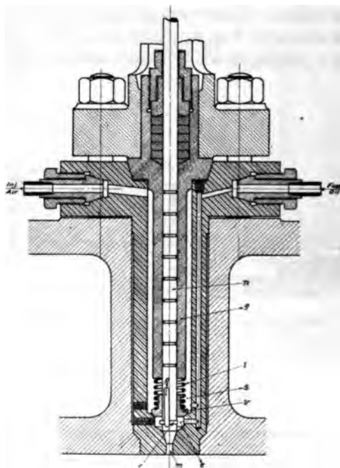
FIG. 9 ATOMIZER OF SABATHÉ ENGINE
