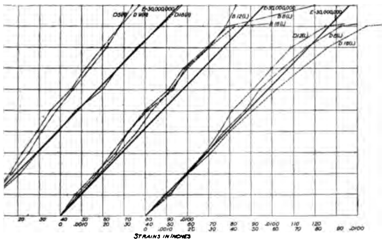
4 CURVES OF TANGENTIAL EXTENSION, SOLID SHEETS, NEAR GIRTH SEAMS AND AT MIDDLE OF LENGTHS OF COURSES
