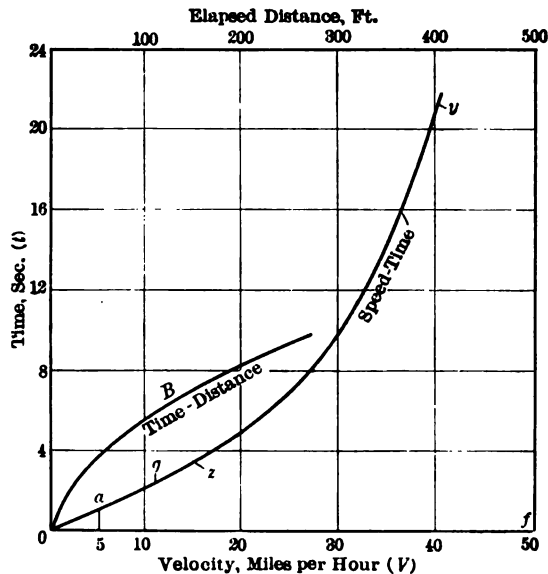
FIG. 4 ACCELERATION CURVES
