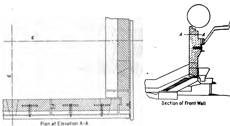
FIG. 20 DETAIL OF NEW SETTING FOR TAYLOR STOKERS
