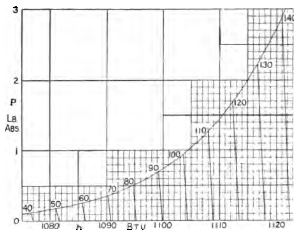
FIG. 13 ISOTHERMAL CHART
