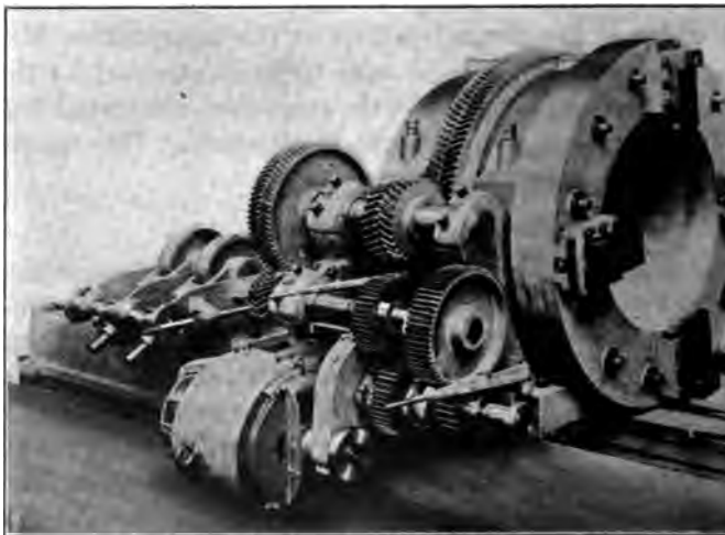
FIG. 11 GUN-BORING LATHE WITH HERRINGBONE GEAR
