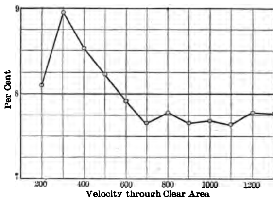
FIG. 32 PERCENTAGE OF ERROR IN AIR MEASUREMENTS AS COMPARED WITH CONDENSATION
