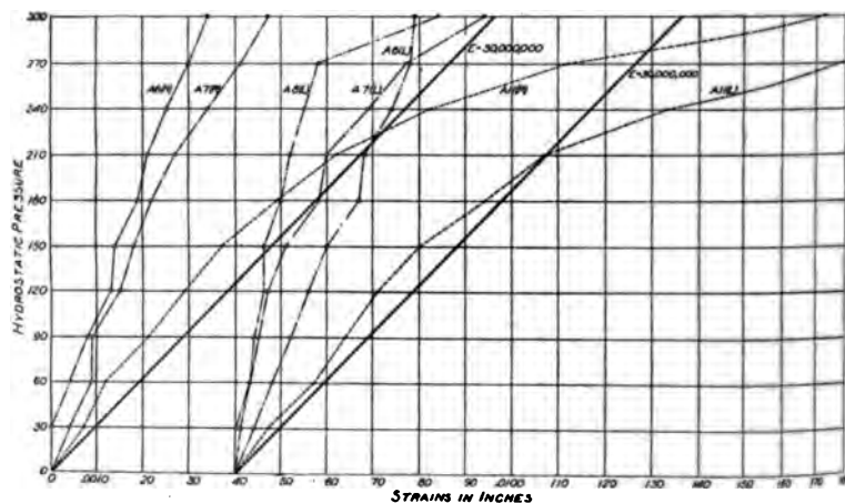
FIG. 24 CURVES OF TANGENTIAL EXTENSION, ACROSS LONGITUDINAL SEAM AND SOLID SHEETS, END COURSE A; EXTENSIONS NEAR FRONT AND GIRTH SEAM
