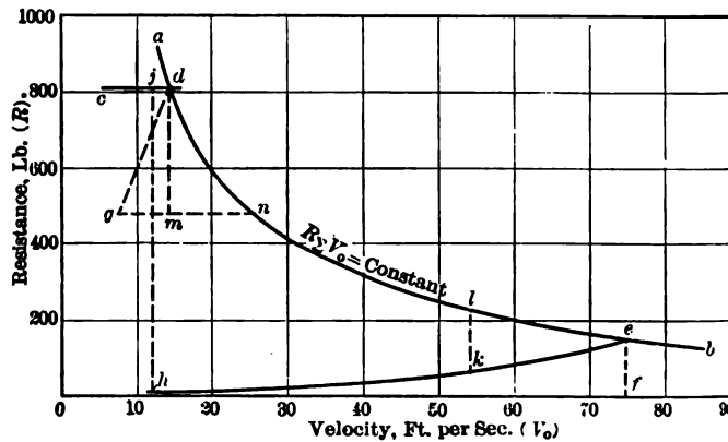
FIG. 3 HEAD-END AND ACCELERATING FORCES
