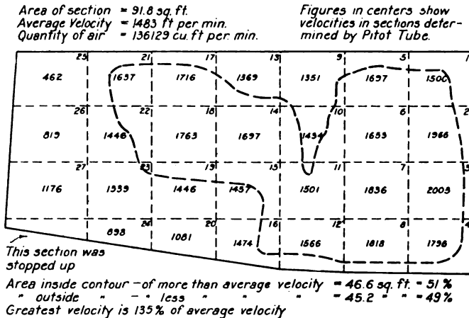
FIG. 13 SECTION AND VELOCITIES IN AIRWAY, FAN TEST No. 9
