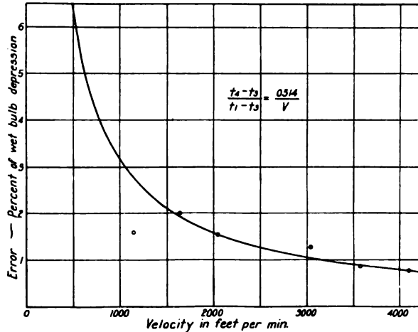
FIG. 6 RADIATION ERROR IN WET BULB OF SLING PSYCHROMETER
