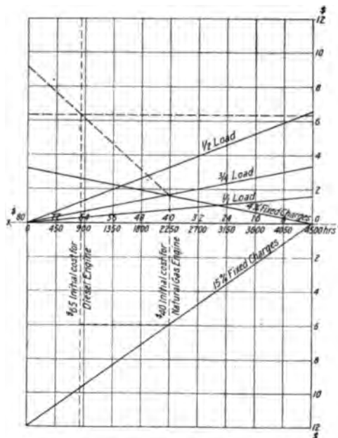
FIG. 36 COMPARISON BETWEEN DIESEL ENGINE AND NATURAL GAS ENGINE
