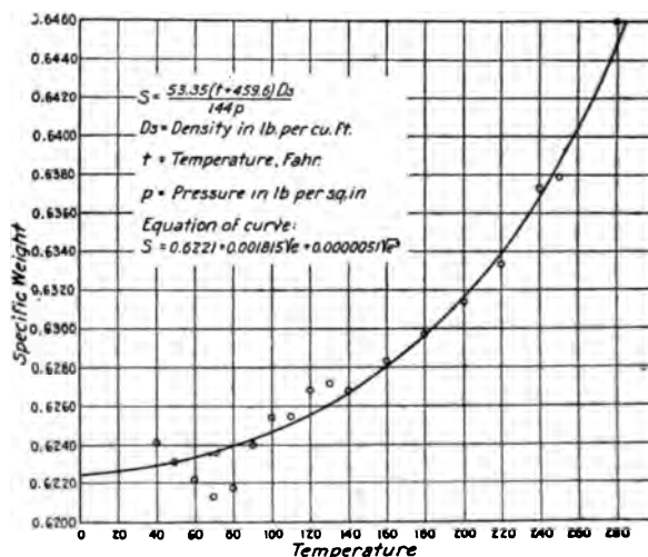
FIG. 4 SPECIFIC WEIGHT OF STEAM
