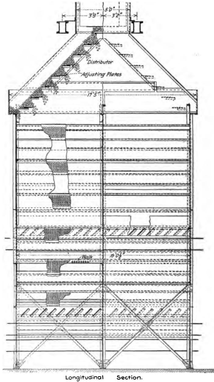
FIG. 13 END ELEVATION OF EDISON SIZING SCREEN
