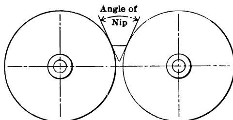
FIG. 17 ANGLE OF NIP ON SMOOTH ROLLS
