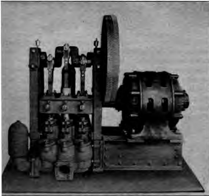
HERRINGBONE GEARS APPLIED TO ELECTRICALLY-DRIVEN TRIPLEX PUMP
