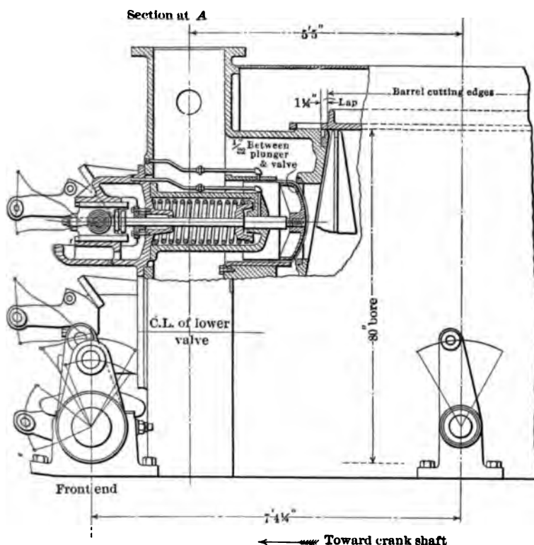
Fig. 14 BLOWING TUB WITH MOVABLE CYLINDER (SLICK DESIGN) BUILT BY ALLIS COMPANY
