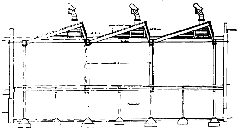
FIG. 1 STANDARD SAW-TOOTH SKYLIGHT IN MILL CONSTRUCTION OVER A DEPARTMENT OF THE FIBRELOID COMPANY'S PLANT, INDIAN ORCHARD, MASS. NOTE THE FLAT ROOF BETWEEN SKYLIGHT AND THE VENTILATORS
