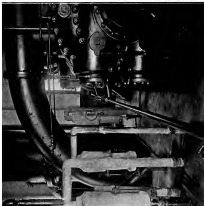
TERS (ON THE LEFT) AND SEPARATING CALORIMETERS USED IN QUALITY OF WET STEAM USED FOR FEED HEATING
