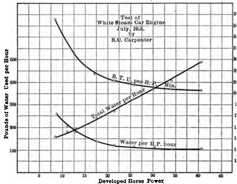
FIG. 11 ECONOMIC RESULTS OF TEST
