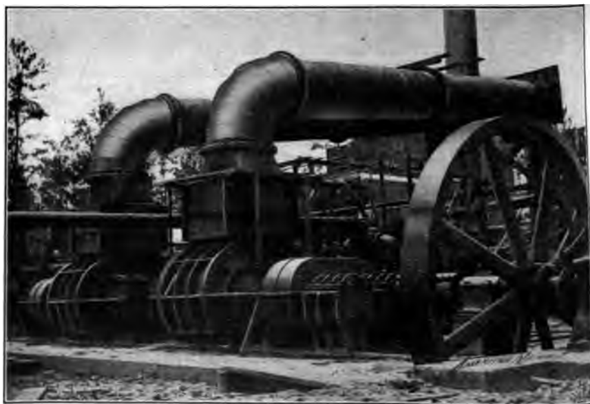
FIG. 4 PUMPING PLANT IN PROCESS OF ERECTION
