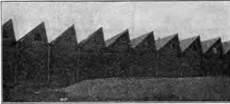
FIG. 4 NEW ENGLAND WEAVING MILL. SAW-TEETH CRITICISED AS TOO HIGH FOR THE SPAN
