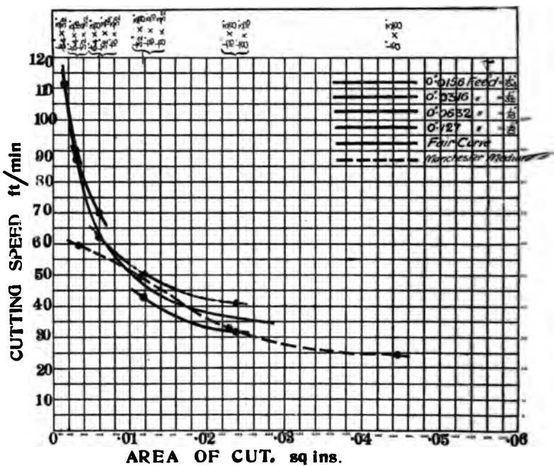
FIG. 2 RESULTS FROM TABLE 76, CAST IRON
