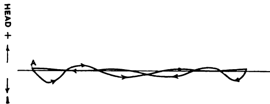
FIG. 1 CARD SHOWING SURGING OF AIR PRESSURE IN PIPES LEADING AIR TO AIR COMPRESSORS
