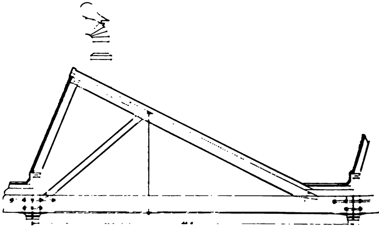
FIG. 4. ELABORATE TRUSSED FORM OF SAW-TOOTH SKYLIGHT
