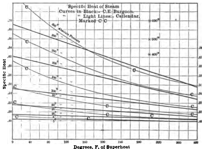
FIG. 13 COMPARISON OF SIBLEY COLLEGE RESULTS WITH THOSE OF PROFESSOR CALLENDER
