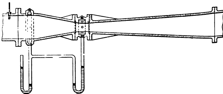
FIG. 1 VENTURI TUBE
