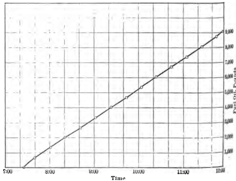
FIG. 15 MAIN PUMPING PLANT, NECHES CANAL CO. August 9, 1906
