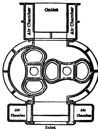
FIG. 3 CROSS-SECTION OF PUMPS
