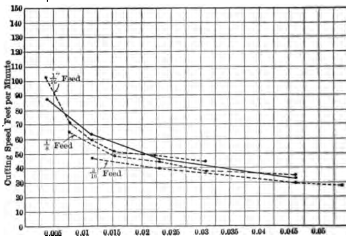
FIG. 1 DIAGRAM SHOWING COMPARATIVE RESULTS OF EXPERIMENTS BY THE MANCHESTER COMMITTEE AND BY F. W. TAYLOR
