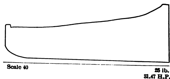
FIG. 7 INDICATOR CARDS OF WORTHINGTON DUPLEX COMPOUND PUMPS TIME 2:45 P. M., SEPTEMBER 7, 1905
