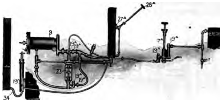
FIG. 5 WATER CIRCULATION SYSTEM
