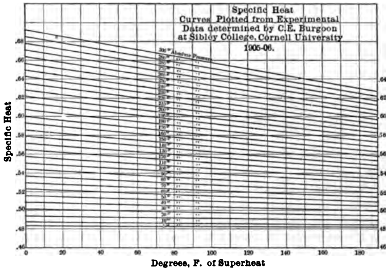
FIG. 12 SPECIFIC HEAT OF SUPERHEATED STEAM
