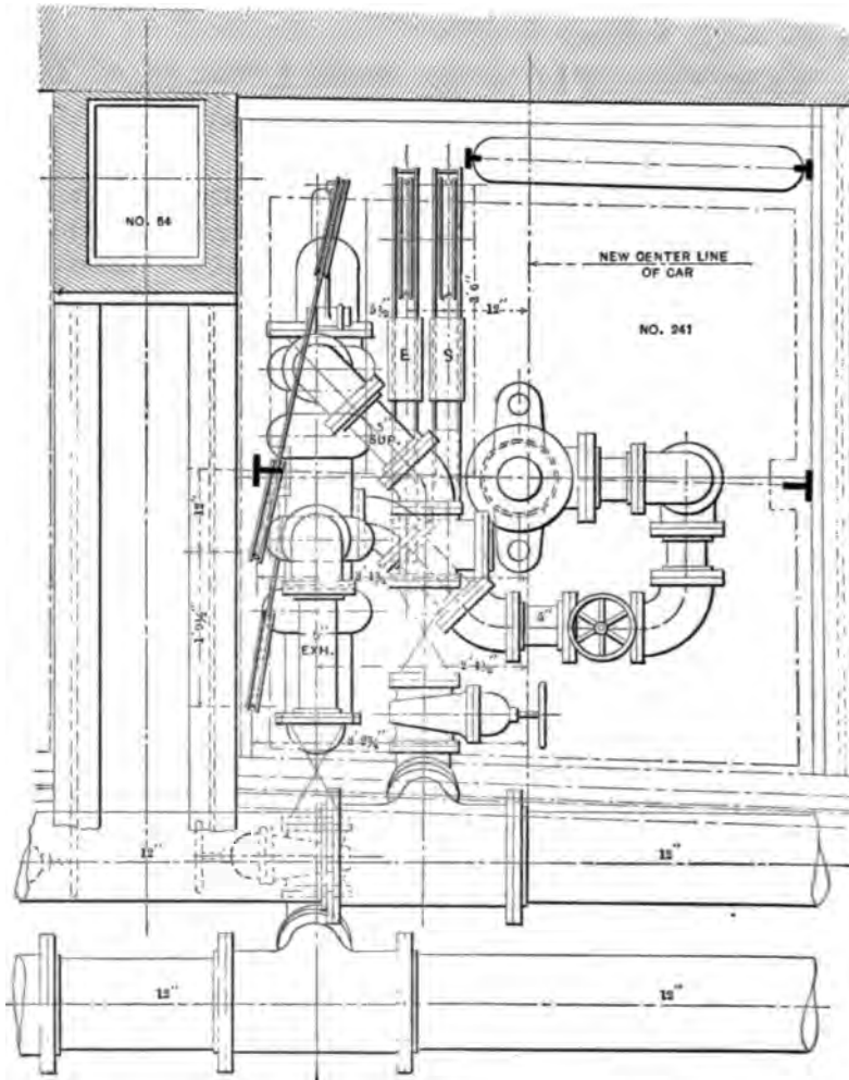
FIG. 1 PLAN OF ELEVATOR SHOWING CONTROLLING VALVE AND AUTOMATIC STOP OPERATING MECHANISM
