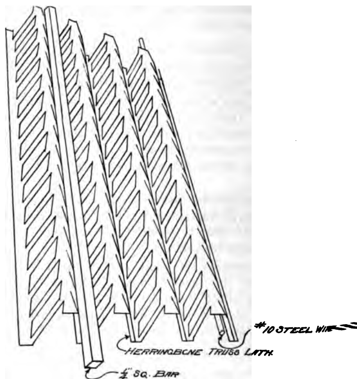
FIG. 1 HERRINGBONE TRUSS LATH
