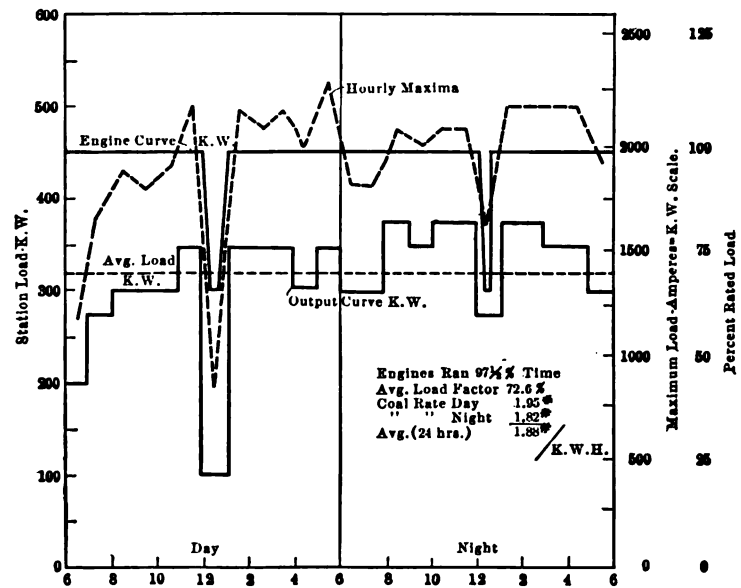
FIG. 3b LOAD DIAGRAM GAS ENGINE PLANT JULY 11, 1905
