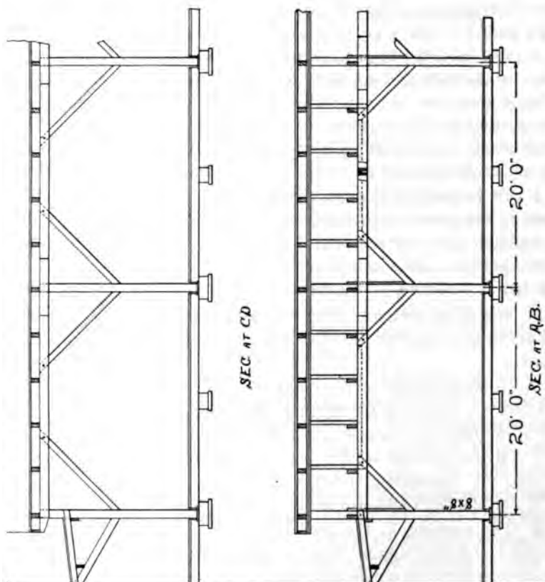
A B AND C D SAW-TOOTH ROOFS USED IN COTTON COMPRESS SHEDS
