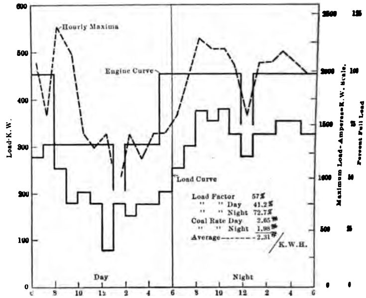
FIG. 3c LOAD DIAGRAM 450 K.W. GAS POWER PLANT JULY 13, 1905
