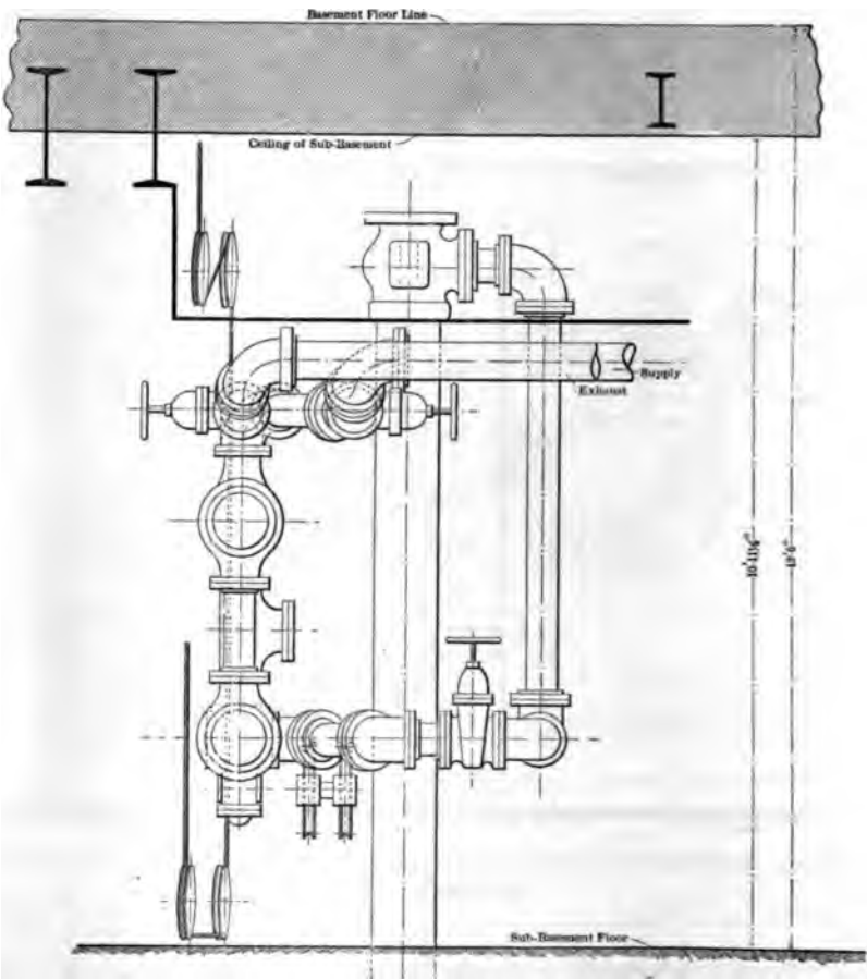
FIG 3 ELEVATION SHOWING PIPING CONNECTIONS
