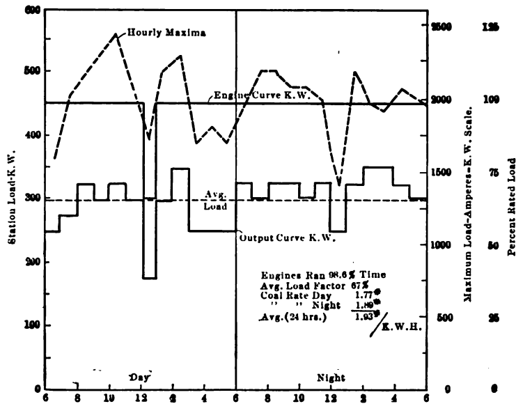
FIG. 3a LOAD DIAGRAM GAS ENGINE PLANT APRIL 13, 1905
