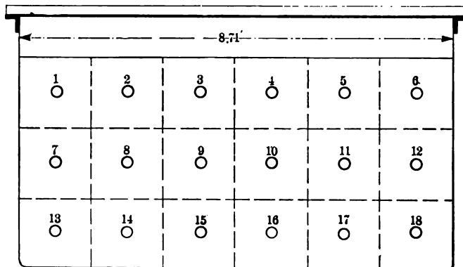
FIG. 9 CROSS-SECTION OF FLUME SHOWING POINTS WHERE VELOCITY WAS OBSERVED BY MEANS OF THE PITOT TUBE
