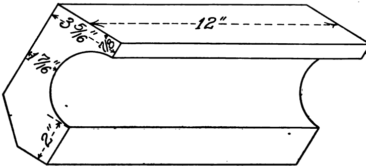
FIG. 2 REFRACTORY TILE FOR FURNACE ROOF
