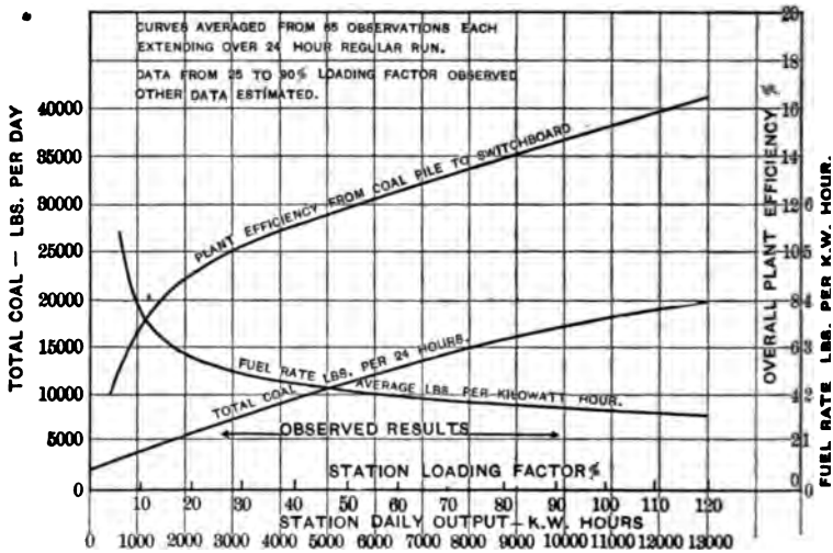
FIG. 1 SUMMARY OF OPERATING RESULTS, GOULD COUPLER CO., DEPEW, N. PRODUCER GAS PLANT
