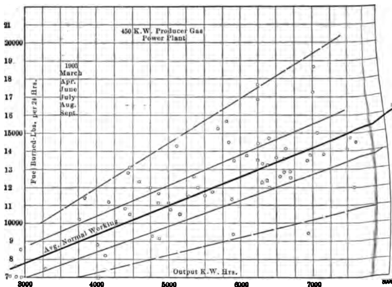
FIG. 5 FULL CONSUMPTION AT VARIOUS OUTPUTS (GRAPHICAL METHOD OF OBTAINING TRUE AVERAGE)
