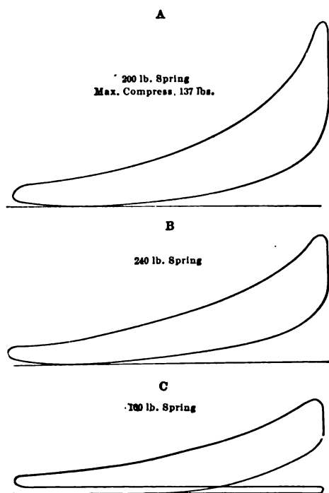
FIGS. 10a, 10b AND 10c TYPICAL INDICATOR CARDS CORRESPONDING TO LOADS IN TABLE 4
