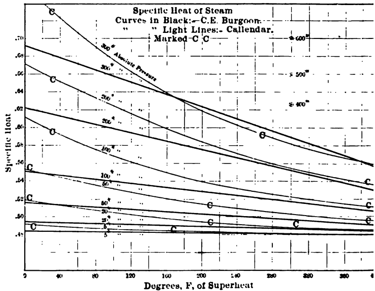
FIG. 13 COMPARISON OF SIBLEY COLLEGE RESULTS WITH THOSE OF PROFESSOR CALLENDER
