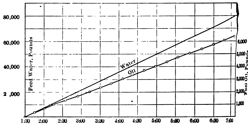
FIG. 14 BOILER TEST, MAIN PUMPING PLANT, NECHES CANAL CO August 8, 1906
