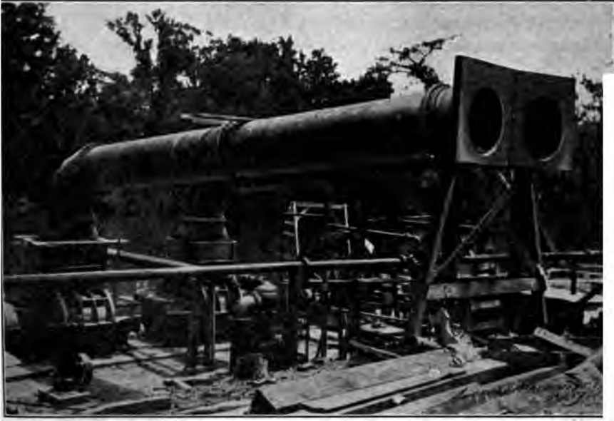
FIG. 5 PUMPING PLANT IN PROCESS OF ERECTION
