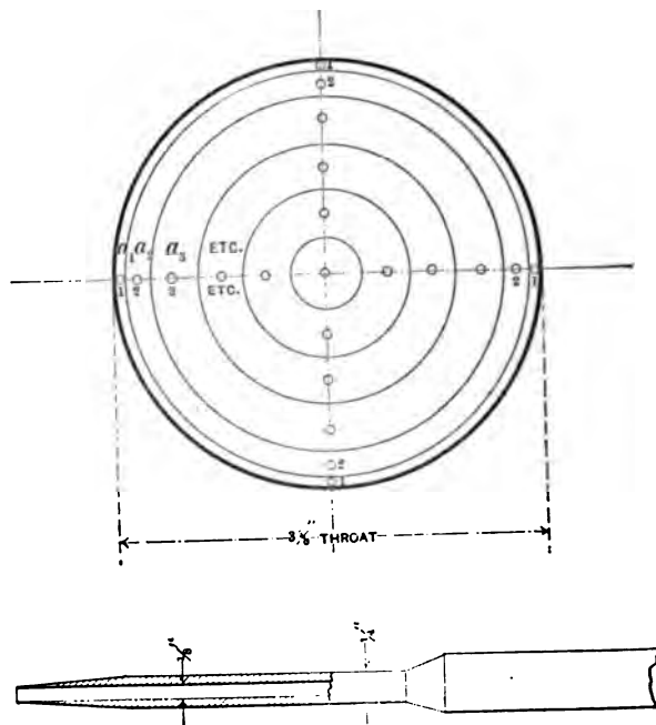
FIG. 3 THROAT CIRCLE AND PITOT TUBE
