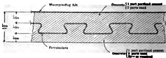
FIG. 1—SECTION OF FERROINCLAVE ROOF AS USED ON SPAN 4' 10 1/4" C. TO C. OF PURLINS
