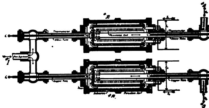
FIG. 1 SUPERHEATING CALORIMETERS FOR DETERMINING THE HEAT OF SUPERHEATED STEAM
