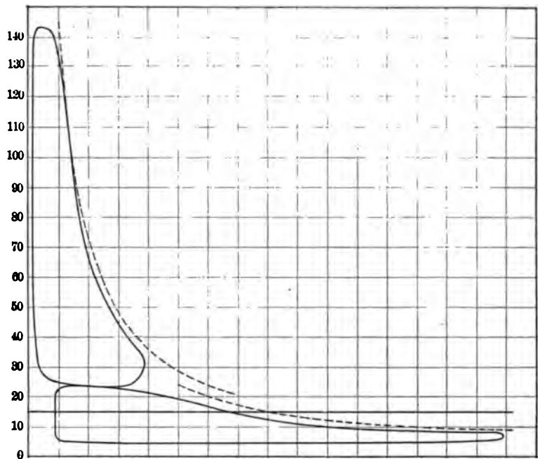
FIG. 12 COMBINED CARDS ENGINE NO. 4 HEAD END Time, 5:30
