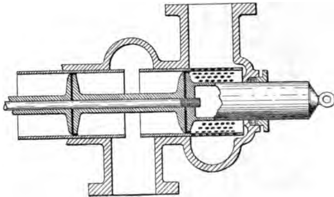
FIG. 2 SIMPLIFICATION OF SUPPLY PART AND ACTUATION AREA OF CONTROLLING VALVE SHOWN FIG. 1
