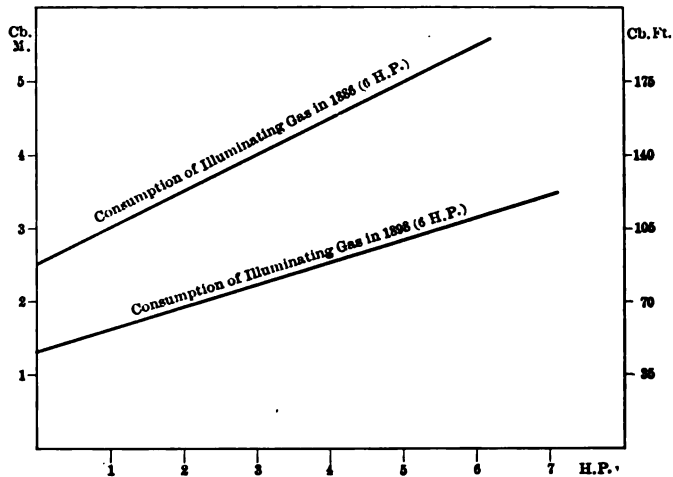
FIG. 8 CONSUMPTION OF KOERTING GAS ENGINE IN 1886 AND 1898
