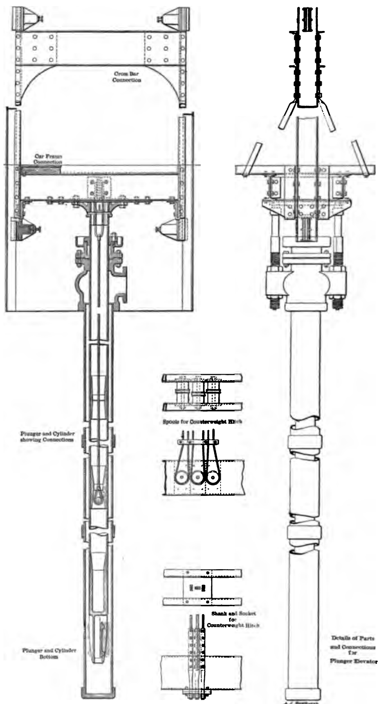
FIG. 5 DETAILS OF PARTS AND CONNECTIONS FOR PLUNGER ELEVATOR
