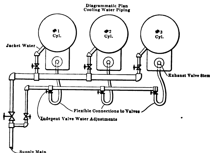
FIG. 11 PLAN COOLING WATER PIPING FOR CYLINDERS AND EXHAUST VALVES
