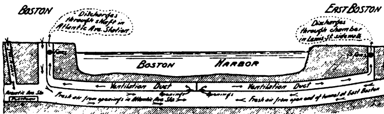
FIG. 7 DIAGRAM (NOT TO SCALE) INDICATING MOVEMENT OF AIR THE LENGTH OF TUNNEL INDICATED IS ABOUT ONE MILE
