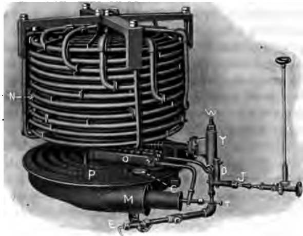
FIG. 1 THE WHITE GENERATOR SHOWING ALSO THE BURNER, VAPORIZER, PILOT LIGHT AND GASOLINE CONNECTIONS WITH EXTERNAL CASING REMOVED
