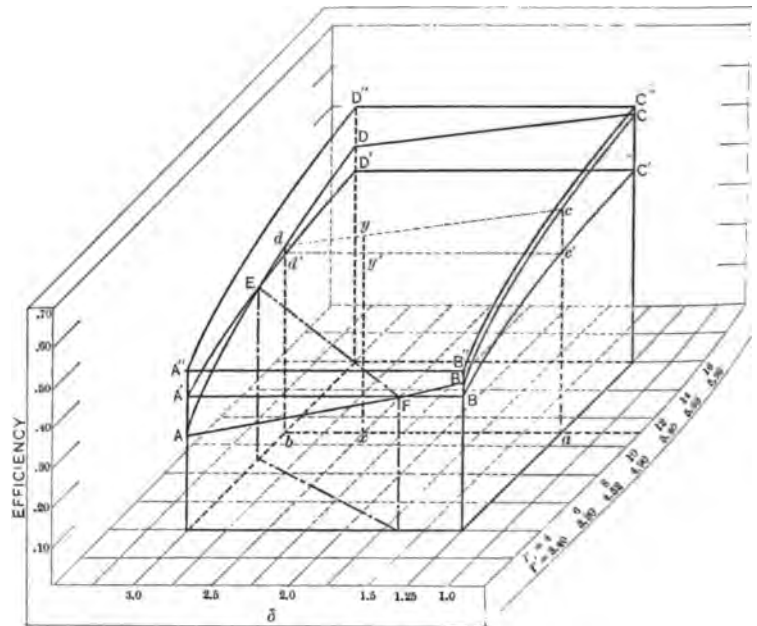
FIG. 1 DIAGRAM SHOWING EFFICIENCIES OF THE OTTO CYCLE
