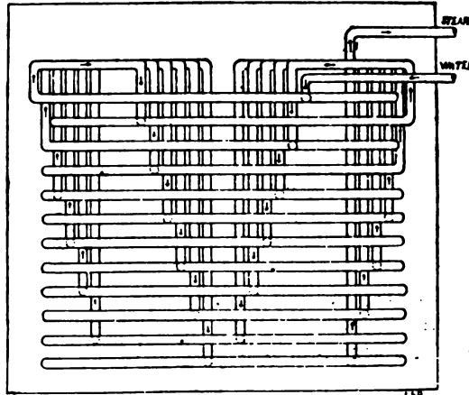
FIG. 2 DIAGRAM OF GENERATOR CIRCULATION
