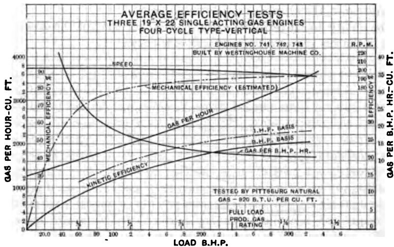
FIG. 9 AVERAGE EFFICIENCY TESTS
