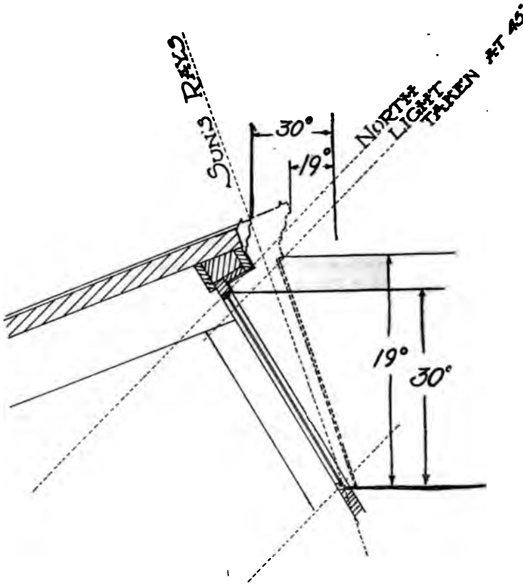
FIG. 1 DIAGRAM ILLUSTRATING APPLICATION OF OVERHANGING CORNICE
