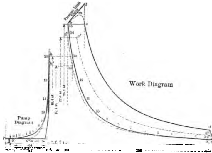
FIG. 2 THEORETICAL WORKING CYCLE OF CONTINUOUS COMBUSTION (WEIDMANN)
