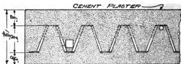
FIG 2 APPLICATION OF HERRINGBONE TRUSS LATH TO LIGHT FIREPROOF ROOF CONSTRUCTION
