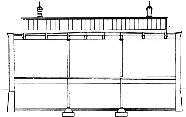
FIG 2 FRONT VIEW OF SAW-TOOTH SKYLIGHT, FIBERLOID COMPANY'S PLANT
