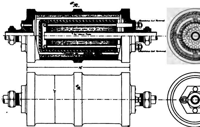
FIG. 2 SUPERHEATING CALORIMETER FOR DETERMINING THE HEAT OF SUPERHEATED STEAM
