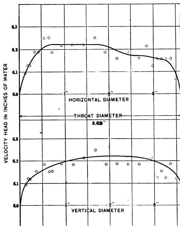
FIG. 6 PITOT TUBE READINGS IN THROAT OF 10" VENTURI TUBE
