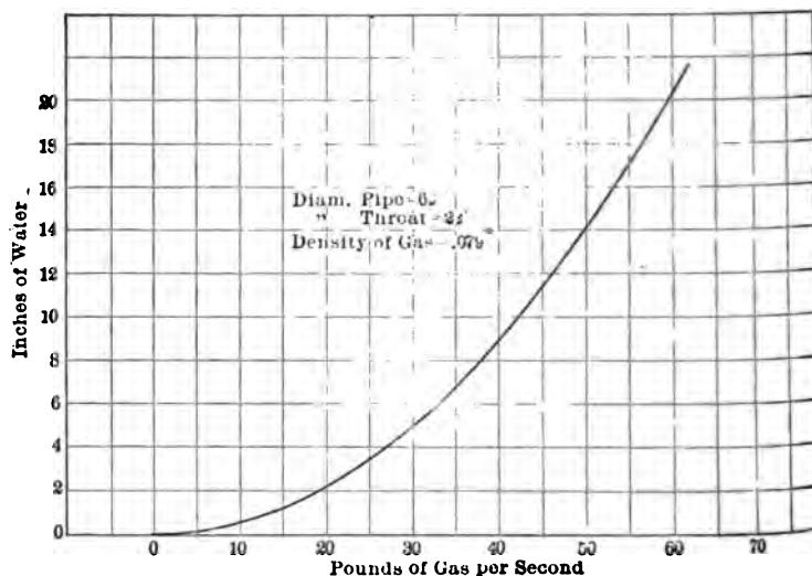
FIG. 11 COMPUTATION CURVE FOR 60" METER
