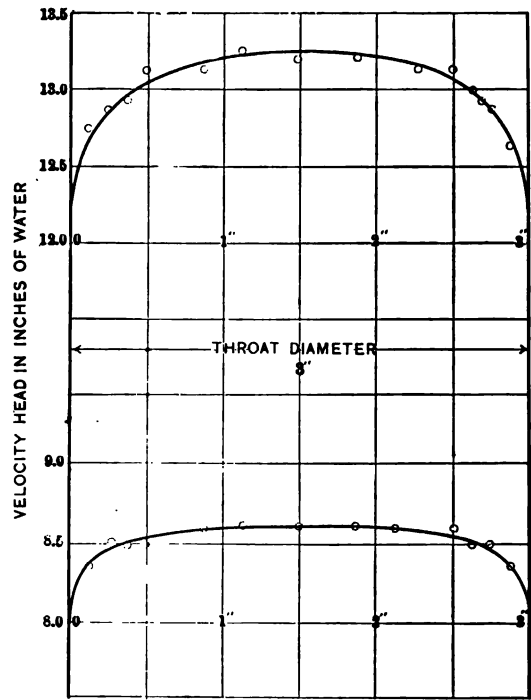
FIG. 8 PITOT TUBE READINGS IN THROAT OF 6" VENTURI TUBE
