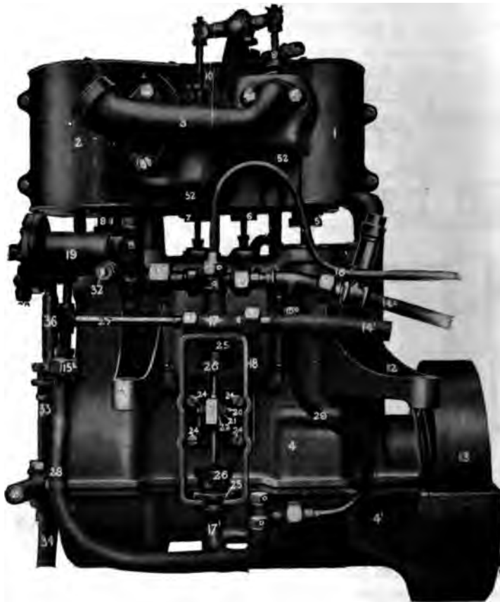
FIG. 7 FRONT VIEW OF ENGINE
