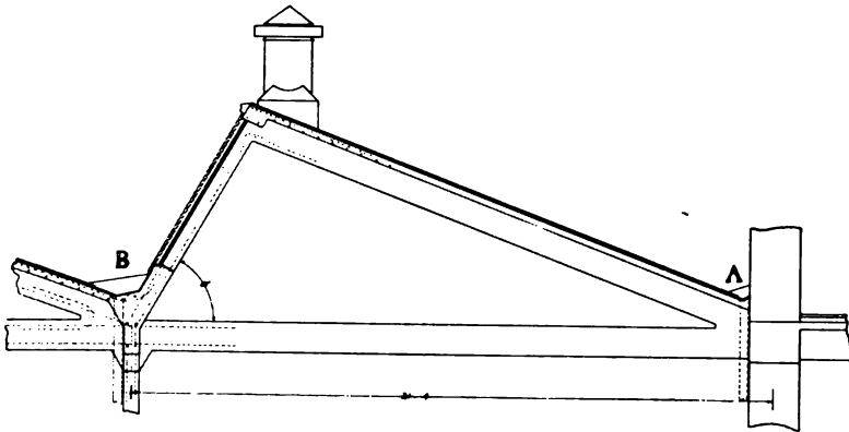
FIG. 5 SAW-TOOTH SKYLIGHT IN REINFORCED CONCRETE, WITH HEAVY CONCRETE BEAM AS BOTTOM CHORD OF TRUSS
