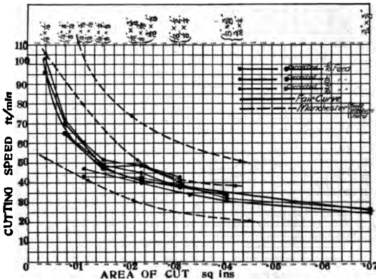
FIG. 1 RESULTS FROM TABLE 70, STEEL
