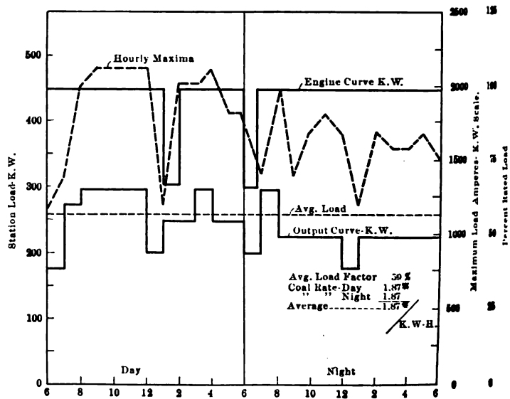
FIG. 3d LOAD DIAGRAM GAS ENGINE PLANT SEPTEMBER 25, 1905
