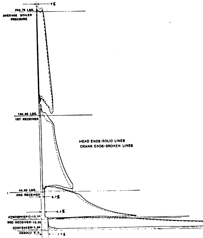
FIG. 4 COMBINED SIMULTANEOUS CARDS FROM HEAD AND CRANK ENDS OF STEAM CYLINDERS VERTICAL SCALE 1"=15 LBS.
