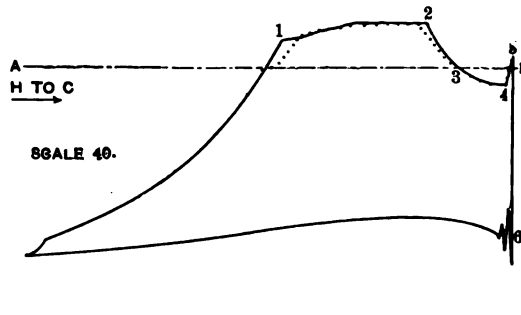
FIG. 3 CARD FROM H. P. AIR CYLINDER FROM DISCHARGE PIPE LINE AND FROM RECEIVER
