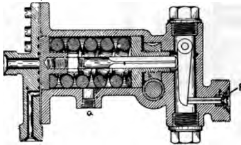
FIG. 4 WATER REGULATOR
