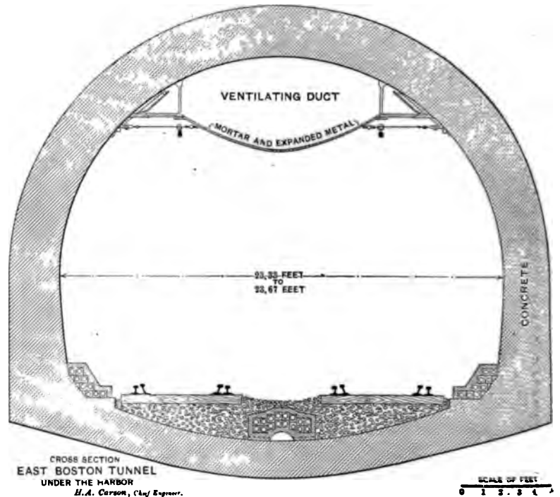
FIG. 6 VENTILATING DUCT
