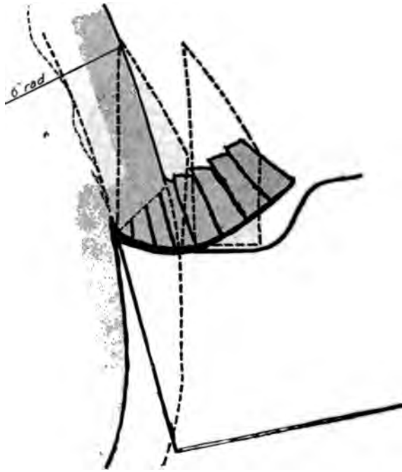
FIG. 2 FORMATION OF CHIP, HIGH SPEED
