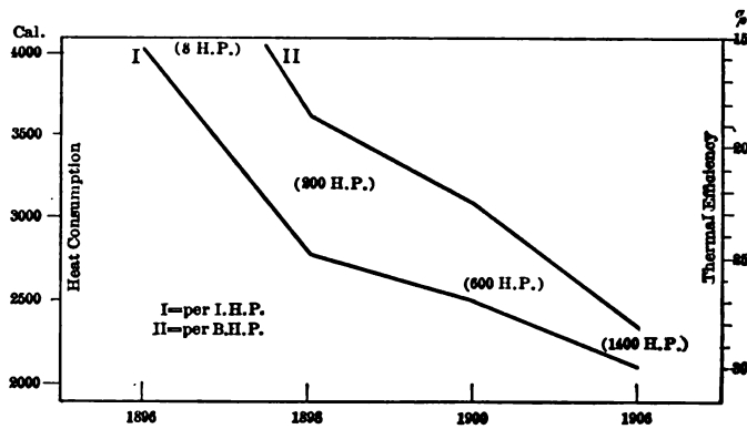
FIG. 5. TABLE SHOWING INCREASING EFFICIENCY OF GAS ENGINES (BELGIUM)
