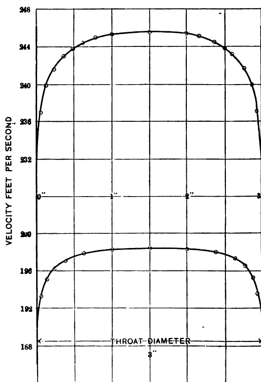
FIG. 10 AVERAGE VELOCITY DIAGRAM IN THROAT OF 6" VENTURI TUBE
