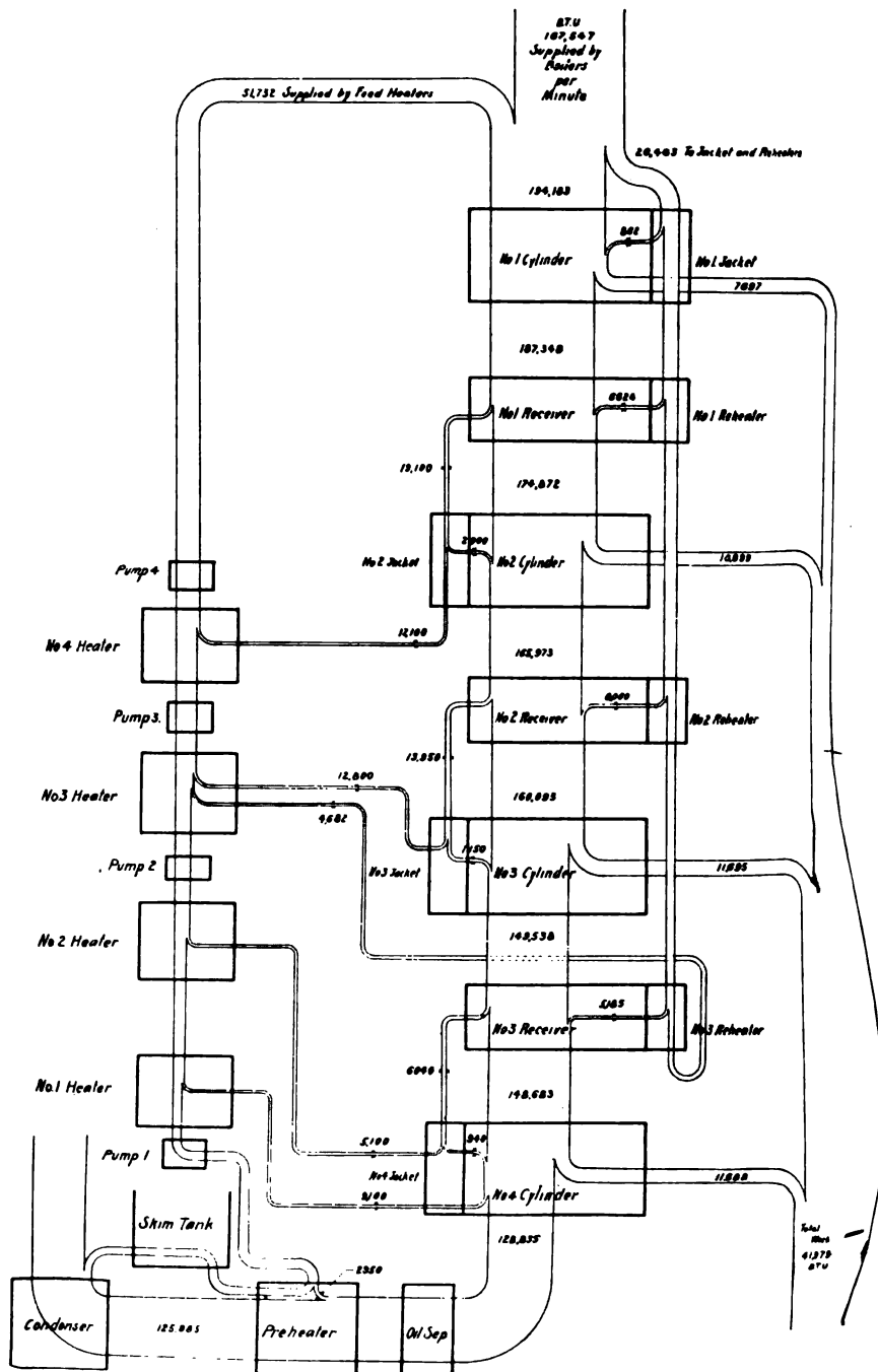
FIG. 2 DIAGRAMMATIC REPRESENTATION OF FLOW OF HEAT THROUGH THE ENGINE (APPROXIMATE DISTRIBUTION)
