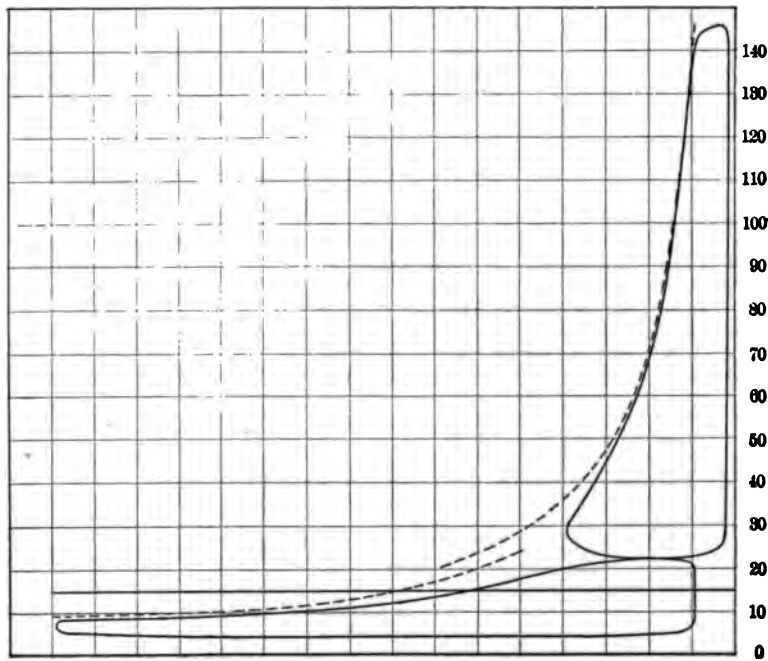
FIG. 13 COMBINED CARDS ENGINE NO. 4 CRANK END Time, 5:30
