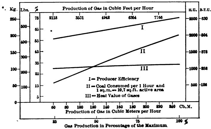
FIG. 6. PERFORMANCE OF DEUTZ DOUBLE ZONE LIGNITE PRODUCER.
