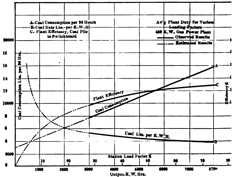
FIG. 6 AVERAGE PLANT DUTY AT VARIOUS LOADING FACTORS
