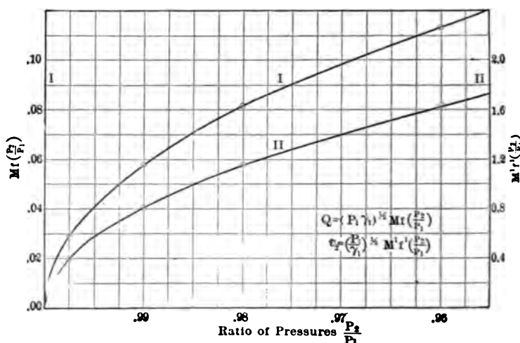
FIG. 5 COMPUTATION CURVES FOR 10" METER
