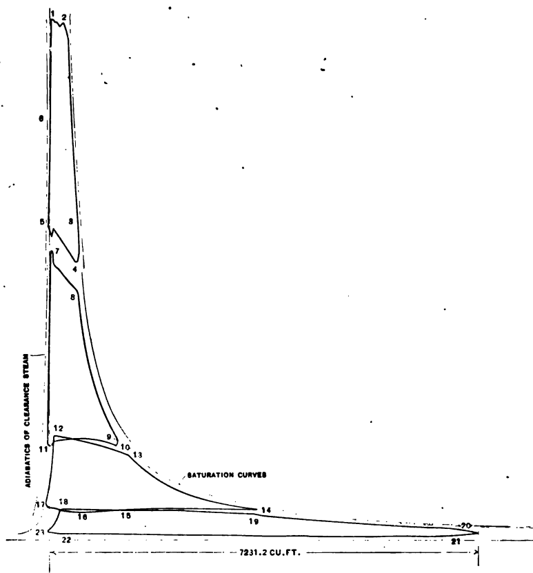
FIG. 3 COMBINED COMPOSITE CARDS SHOWING PRESSURES AND VOLUMES OF CYLINDER FEED PER MINUTE HORIZONTAL SCALE 1"=498 CU. FT. VERTICAL SCALE 1"=15 LBS. PER SQ. IN.
