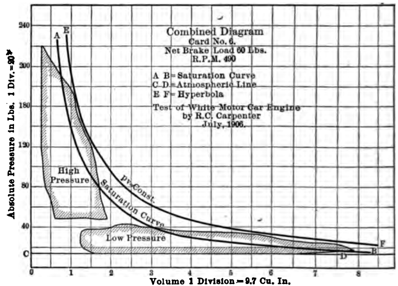
FIG. 16 COMBINED INDICATOR DIAGRAMS
