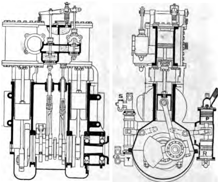
FIG. 6 SECTION AND ELEVATION OF THE ENGINE
