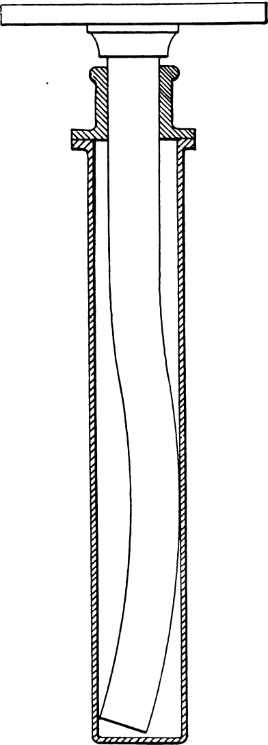
FIG. 5 (NO SCALE) DIAGRAM ILLUSTRATING THE BUCKLIN SLENDER PLUNGERS WHEN LOADED AT THE LOWEF
