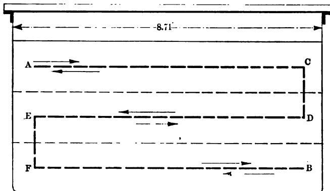
FIG. 7 CROSS-SECTION OF FLUME SHOWING METHOD OF MAKING A TRAVERSE WITH CURRENT METER
