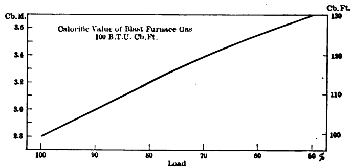
FIG. 4 GAS CONSUMPTION OF OLD TYPE BLAST FURNACE GAS ENGINE FOR ONE EFF. H. P. HOUR AT VARIOUS LOADS
