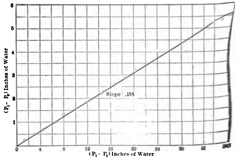
FIG. 9 PRESSURE LOSS IN 6" VENTURI TUBE
