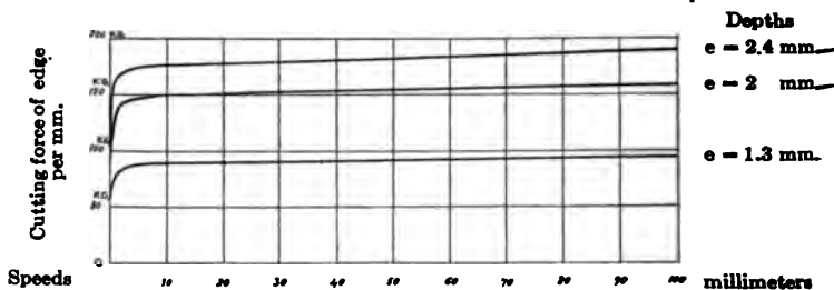
FIG. 2 CUTTING COPPER AT A VARIABLE SPEED, \alpha = 45^\circ , \beta = 5^\circ
