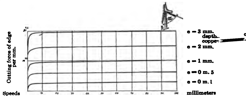
FIG. 1 CUTTING LEAD AT A VARIABLE SPEED, \alpha = 75^\circ , \beta = 5^\circ
