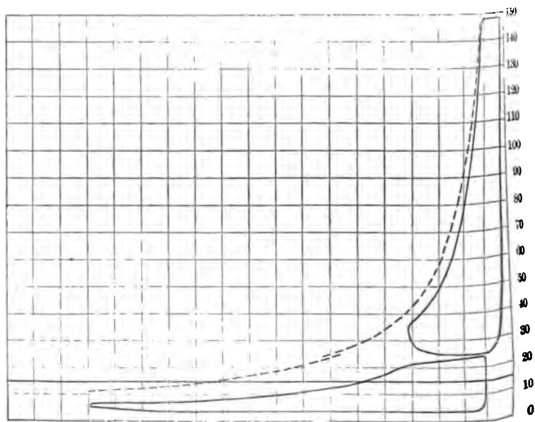
FIG. 11 COMBINED CARDS ENGINE NO. 3 CRANK END Time, 5:30
